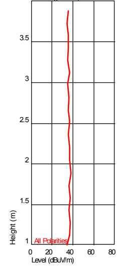
Height Plot ( 60.867133804 MHz )
