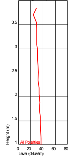
Height Plot ( 171.03927883 MHz )
