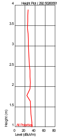
Height Plot ( 292.502605511 MHz )
