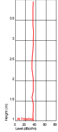
Height Plot ( 41.478156659 MHz )
