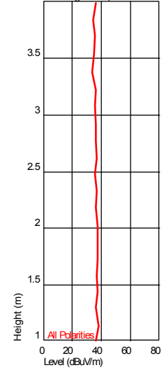
Height Plot ( 63.981362709 MHz )
