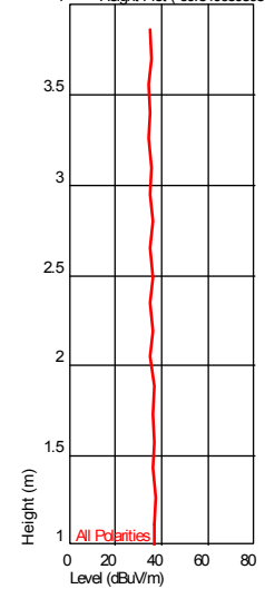
Height Plot ( 60.840680898 MHz )
