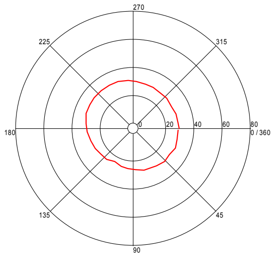
Turntable Plot ( 249.97535112 MHz )
