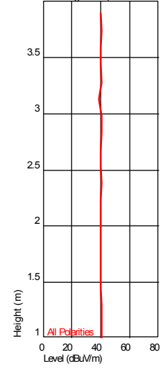
Height Plot ( 36.733065918 MHz )
