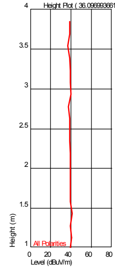
Height Plot ( 36.096993661 MHz )
