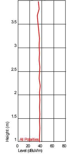
Height Plot ( 64.742885756 MHz )
