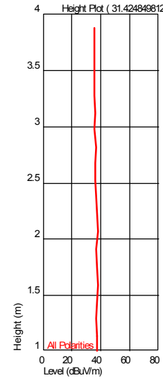
Height Plot ( 31.424849812 MHz )
