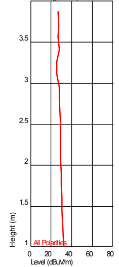
Height Plot ( 250.025852122 MHz )
