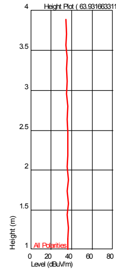
Height Plot ( 63.931663311 MHz )
