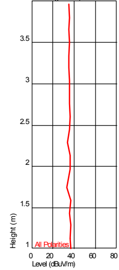
Height Plot ( 60.940881299 MHz )
