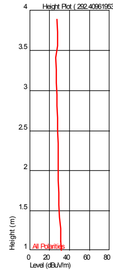
Height Plot ( 292.409619539 MHz )
