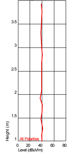
Height Plot ( 51.043487387 MHz )
