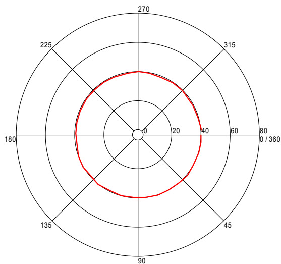
Turntable Plot ( 36.778757301 MHz )
