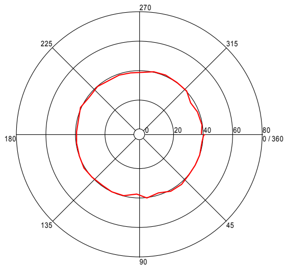
Turntable Plot ( 51.072345102 MHz )
