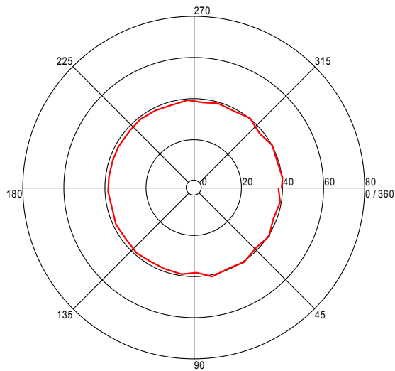
Turntable Plot ( 36.055310295 MHz )
