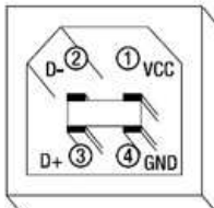
“B” socket from front
