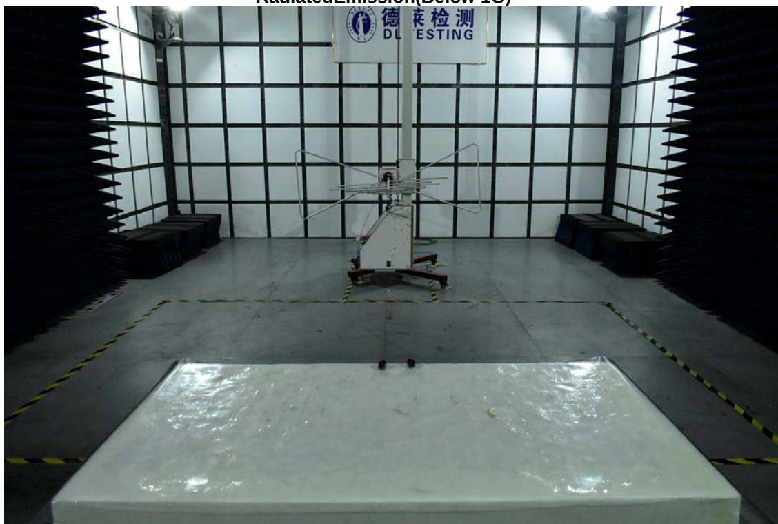
RadiatedEmission(Below 1G)
