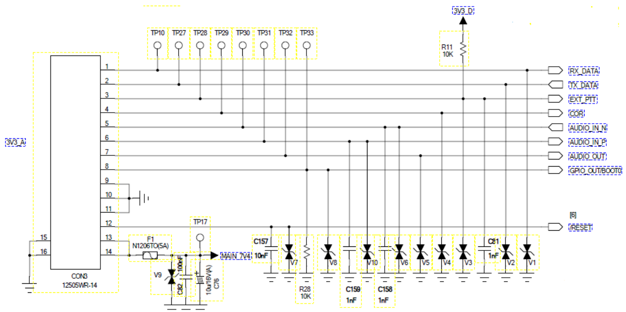
Fig 3. Pin Descriptions
