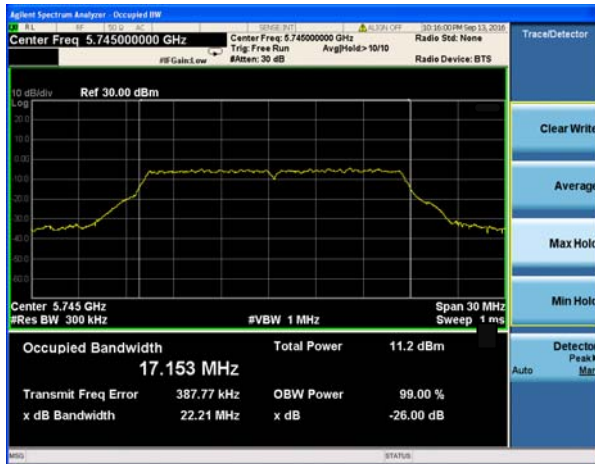
(802.11a) -26dB&amp;99% Bandwidth plot on channel 149
