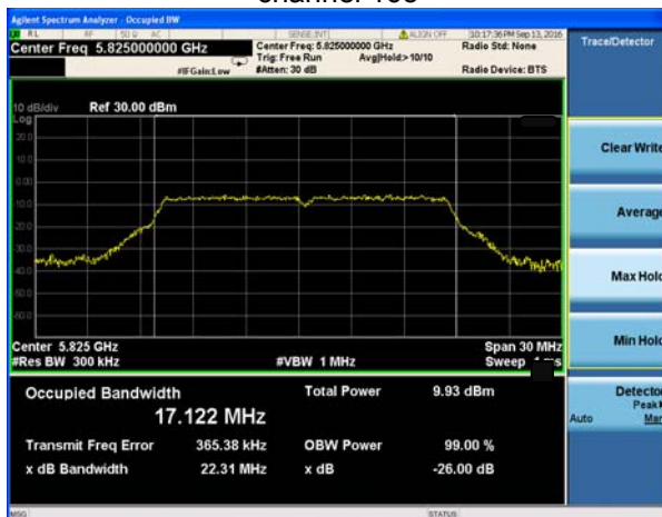
(802.11a) -26dB&amp;99% Bandwidth plot on channel 165
