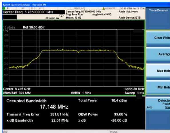
(802.11a) -26dB&amp;99% Bandwidth plot on channel 157
