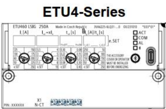
Electronic Trip Unit with Rotary Switches
