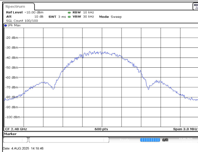
Frequency:2480MHz_1Mbps
