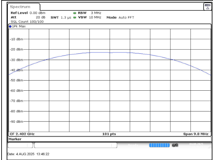
Frequency:2402MHz_2Mbps
