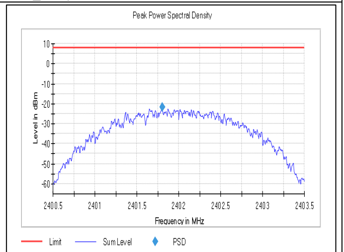
Frequency:2402MHz_2Mbps
