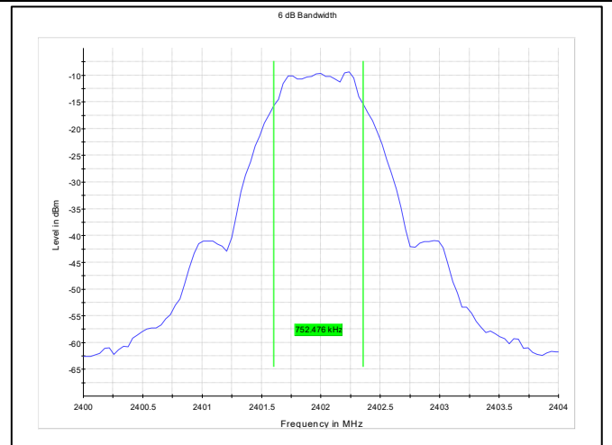
Frequency:2402MHz_1Mbps
