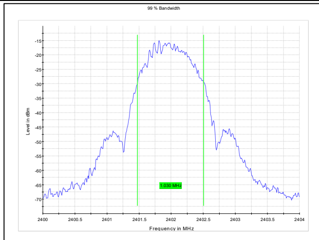
Frequency:2402MHz_1Mbps
