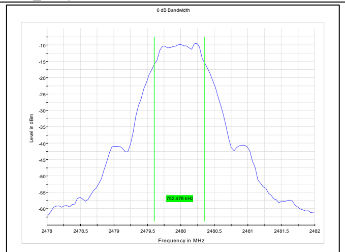
Frequency:2480MHz_1Mbps
