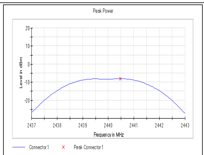
Frequency:2440MHz_2Mbps
