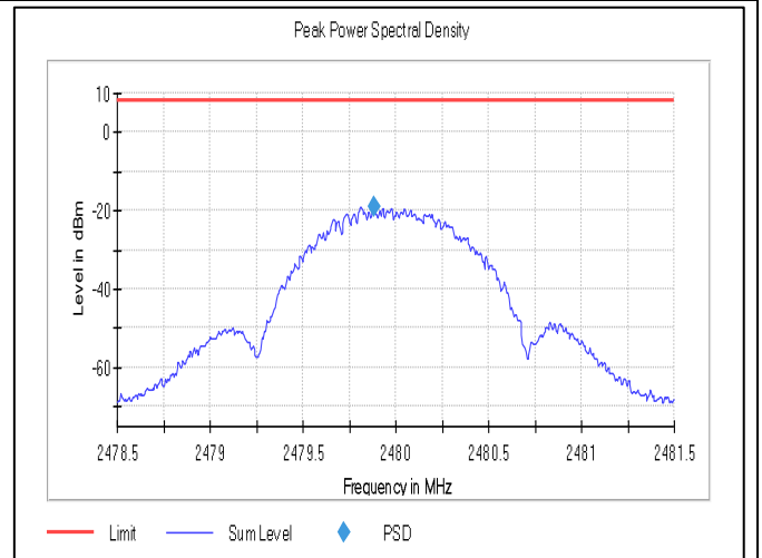
Frequency:2480MHz_1Mbps
