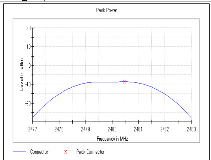
Frequency:2480MHz_2Mbps
