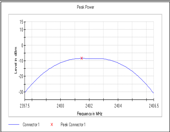
Frequency:2402MHz_2Mbps
