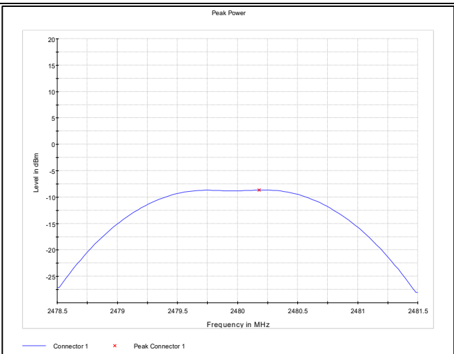
Frequency:2480MHz_1Mbps
