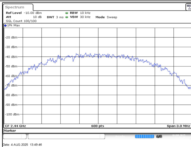
Frequency:2440MHz_2Mbps
