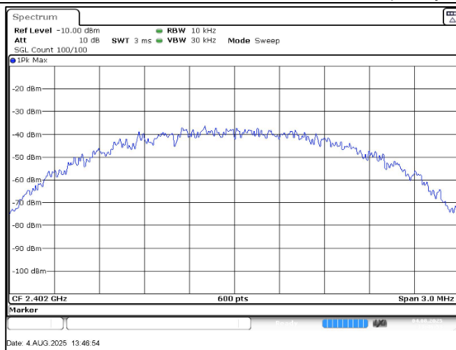
Frequency:2402MHz_2Mbps
