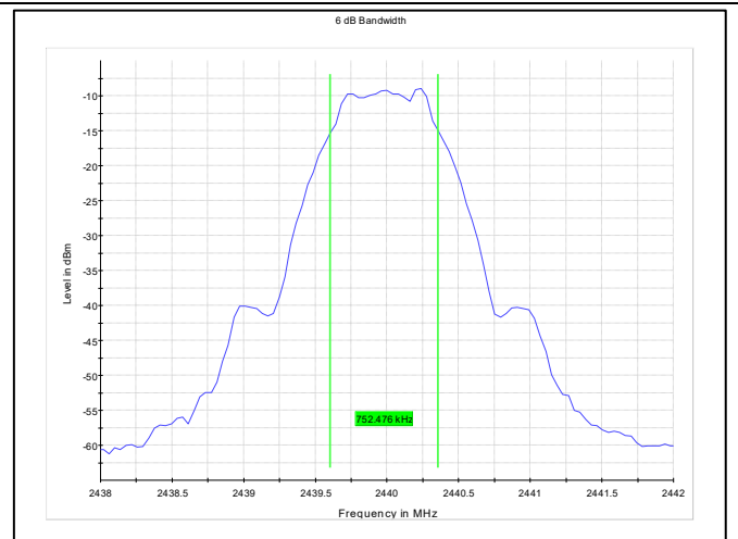
Frequency:2440MHz_1Mbps
