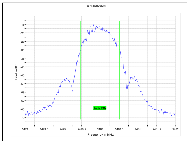
Frequency:2480MHz_1Mbps
