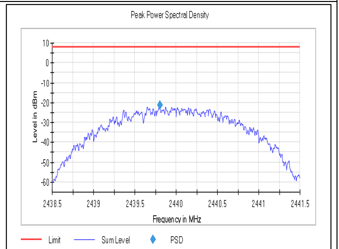
Frequency:2440MHz_2Mbps
