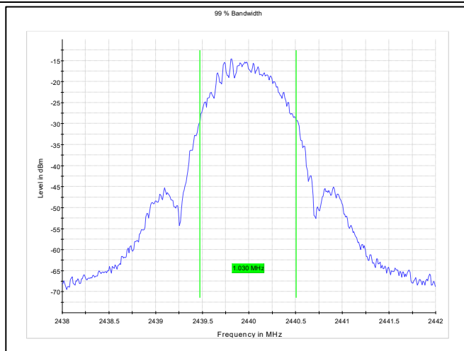
Frequency:2440MHz_1Mbps
