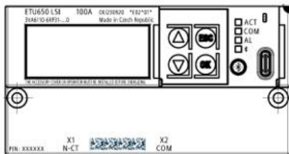
Electronic Trip Unit with Display
