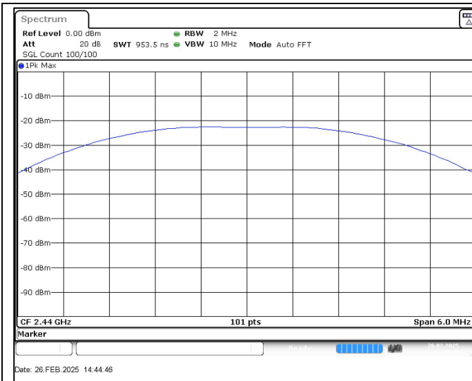
Frequency:2440MHz_2Mbps
