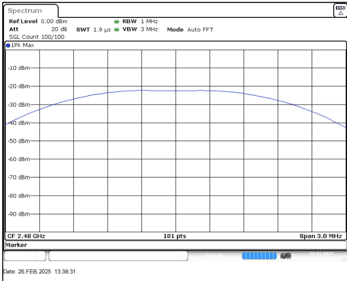
Frequency:2480MHz_1Mbps
