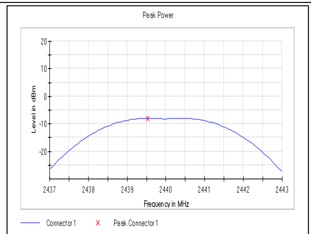
Frequency:2440MHz_2Mbps
