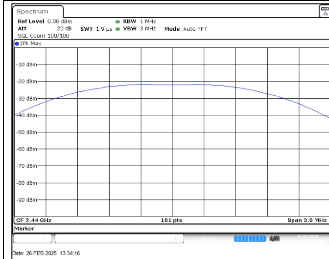
Frequency:2440MHz_1Mbps
