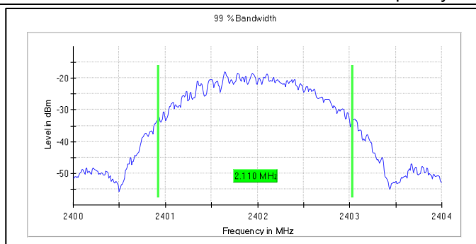
Frequency:2402MHz_2Mbps
