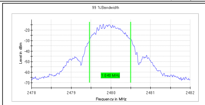
Frequency:2480MHz_1Mbps
