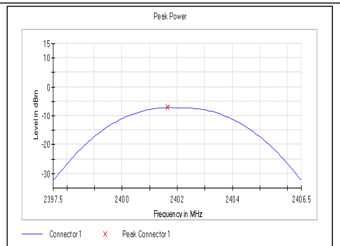
Frequency:2402MHz_1Mbps
