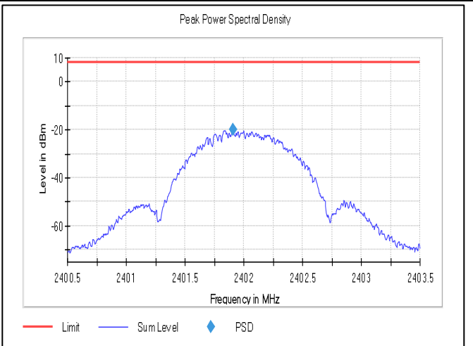
Frequency:2402MHz_1Mbps
