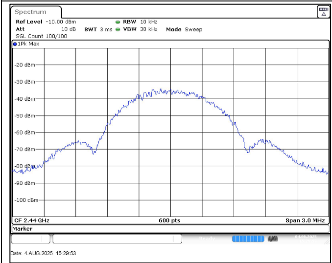
Frequency:2440MHz_1Mbps
