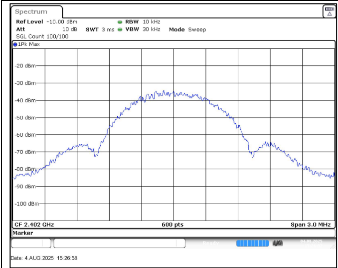
Frequency:2402MHz_1Mbps
