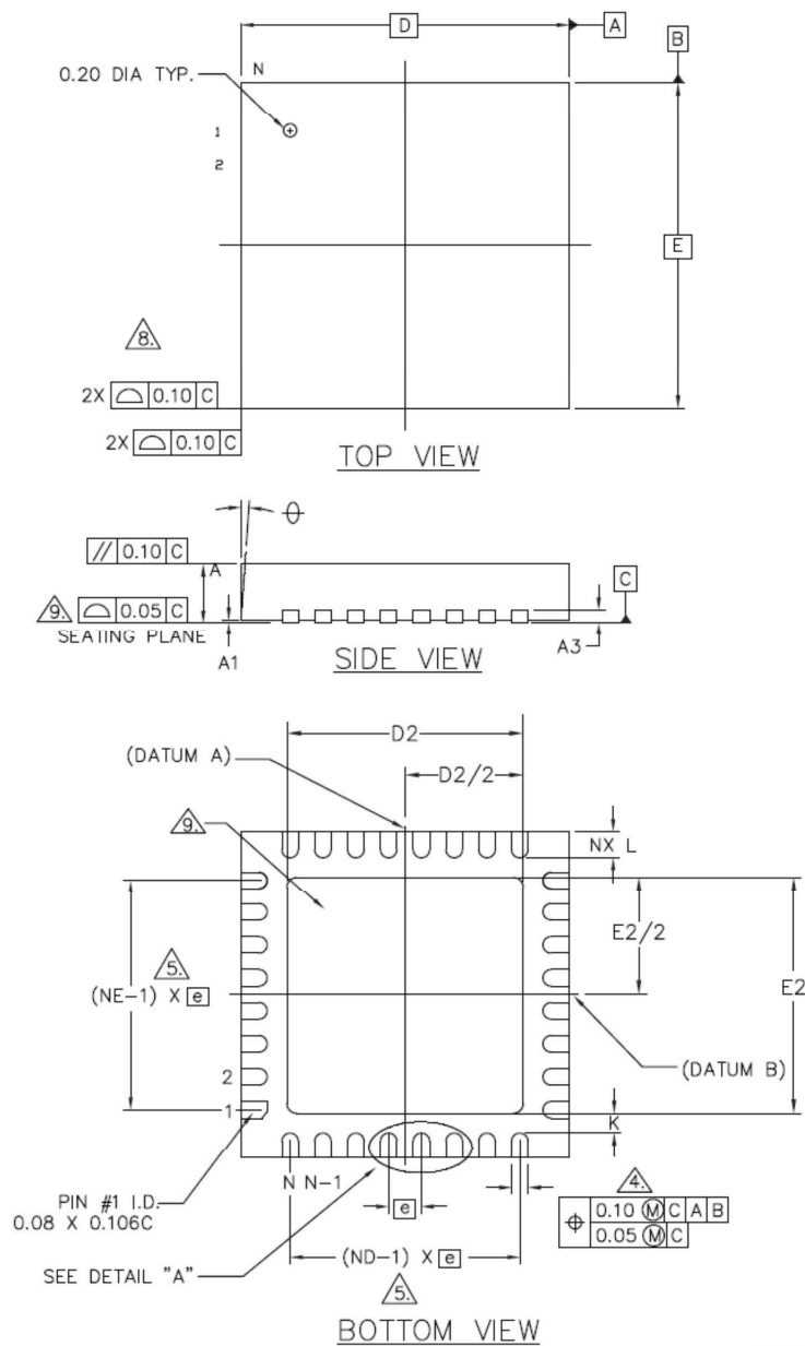
Figure 32. QFN32 (5 x 5 x 1 pitch 0.5 mm) package outline
