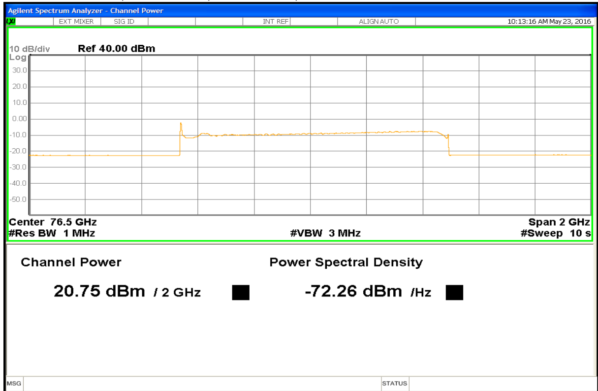
Plot 11: Antenna DN 100, Normal mode, RMS detector, T_{\max} / V_{\min} - V_{\max}
