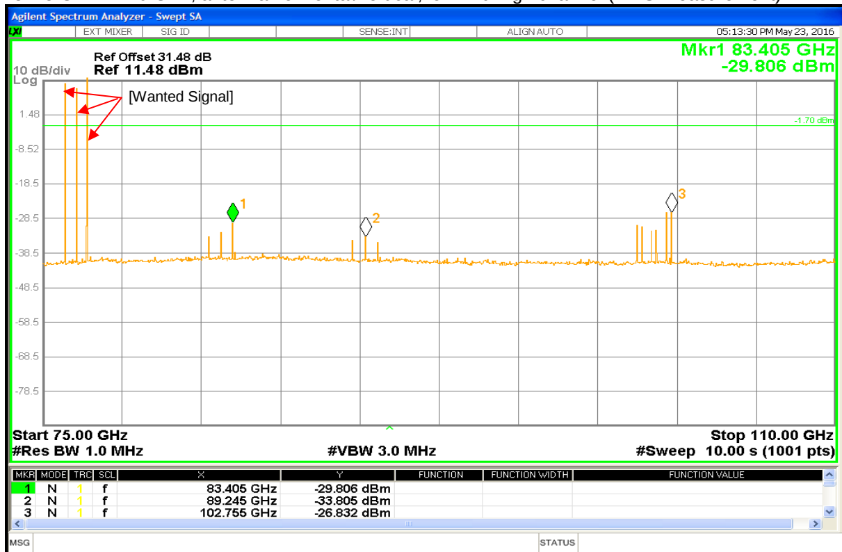
Plot 28: 75 GHz – 110 GHz, antenna horizontal/vertical, low-mid-high channel (RMS-measurement)
