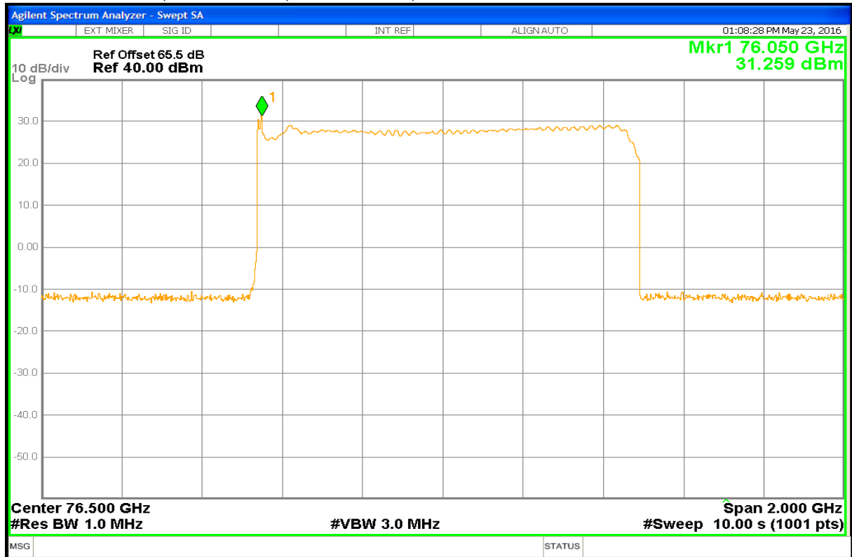
Plot 9: Antenna DN 100, Normal mode, Peak detector, T_{\max} / V_{\min} - V_{\max}
