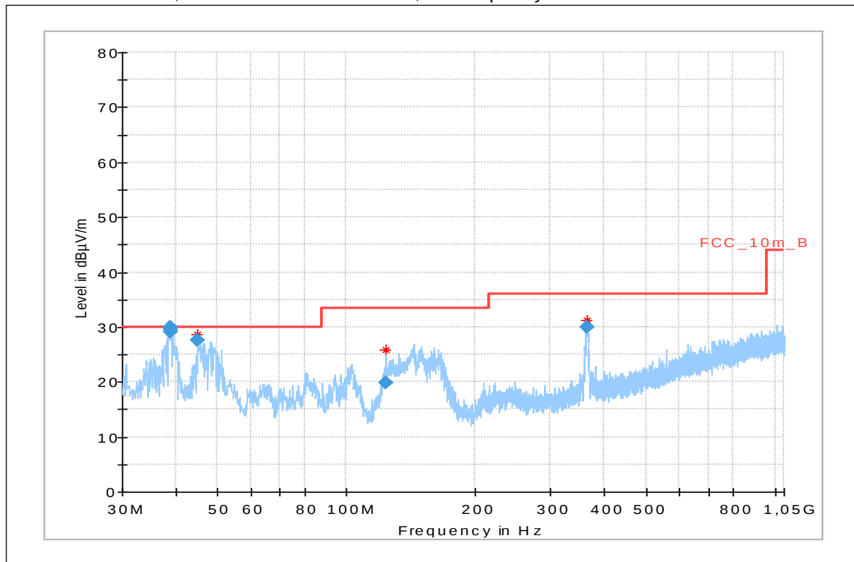
Plot 18: 30 MHz – 1 GHz, antenna horizontal / vertical, mid frequency
