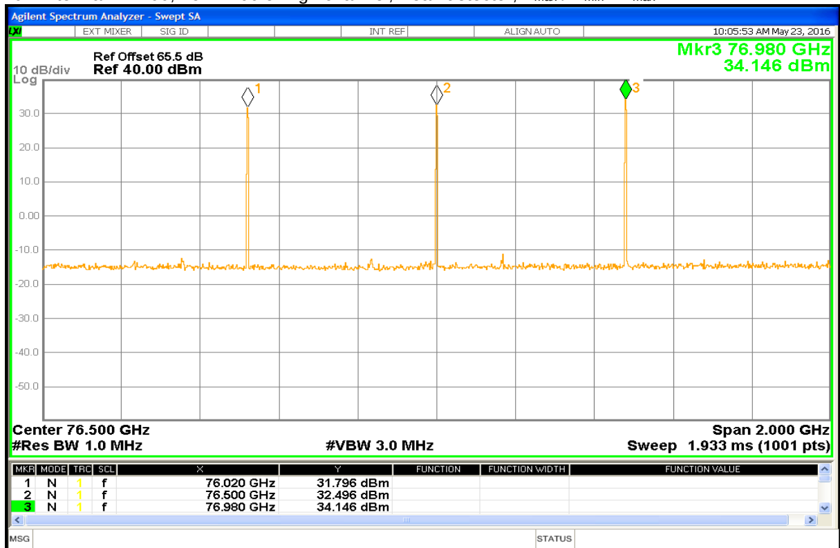
Plot 10: Antenna DN 100, Low-Middle-High channel, Peak detector, T_{\max} / V_{\min} - V_{\max}
