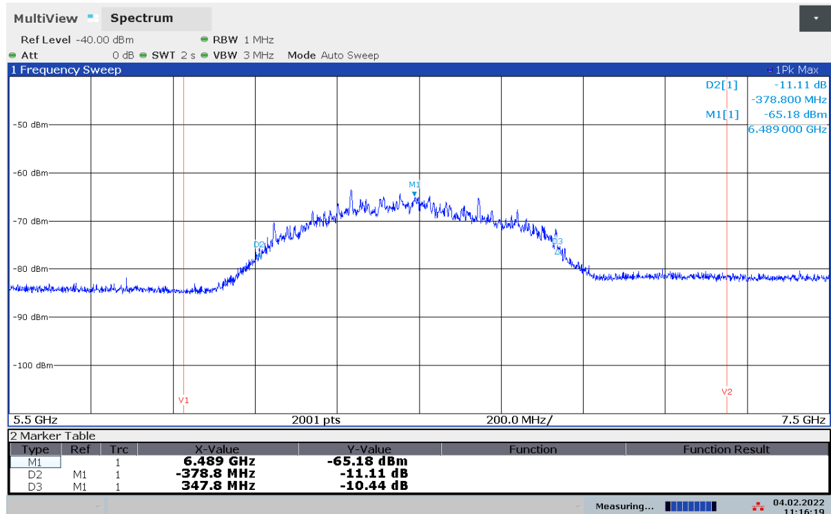
Plot 18: +20 °C, Vmin = 3.25 V (Note: below this value the DUT switches off automatically)
