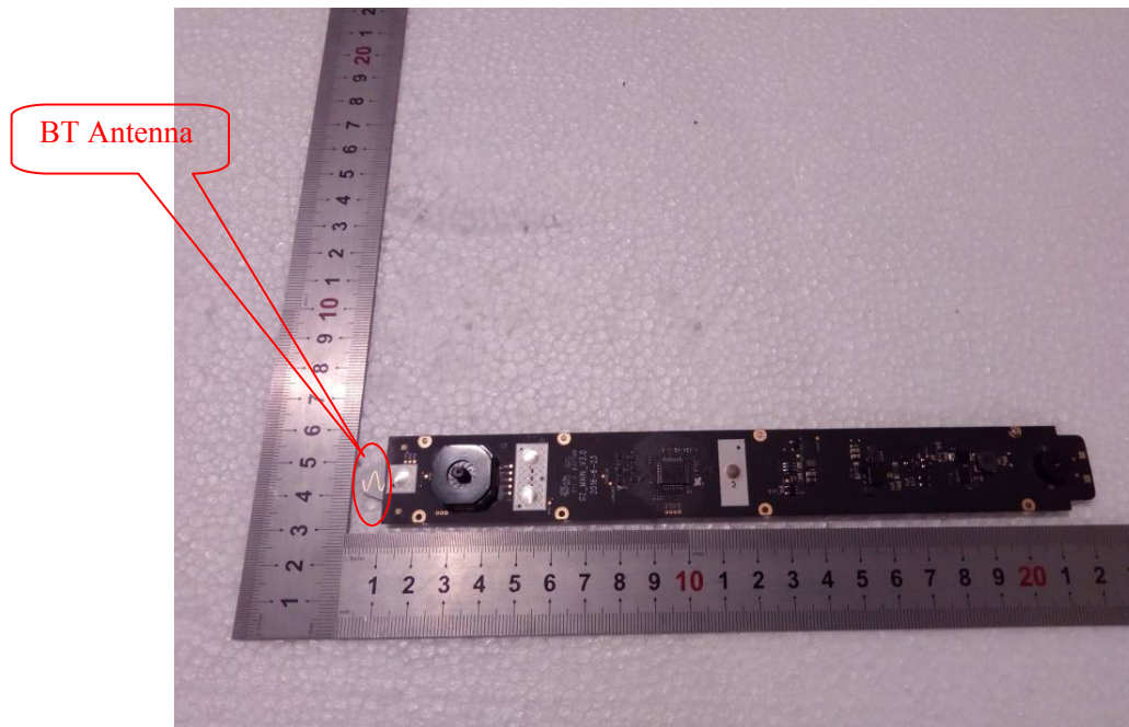
EUT – Main Board 4 Top View
