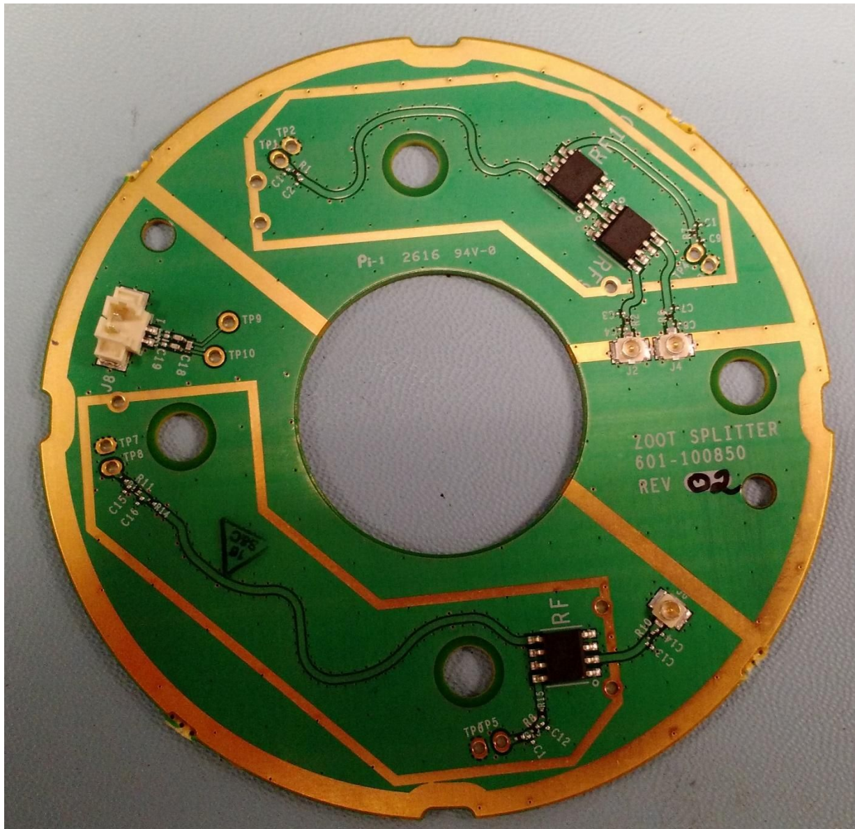
Antenna Splitter PCBA(same as TPv2)
