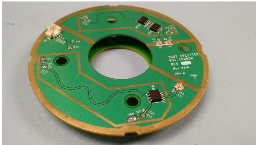
Antenna PCBAs and PCBA Assembly(same as TPv2)
