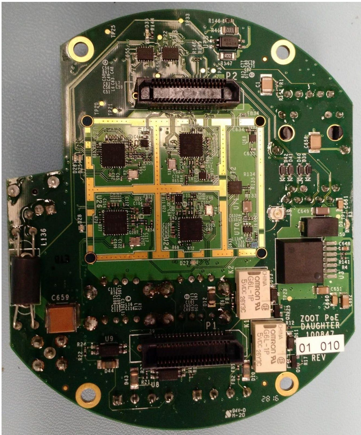
PoE Daughter PCBA(same as TPv2)
