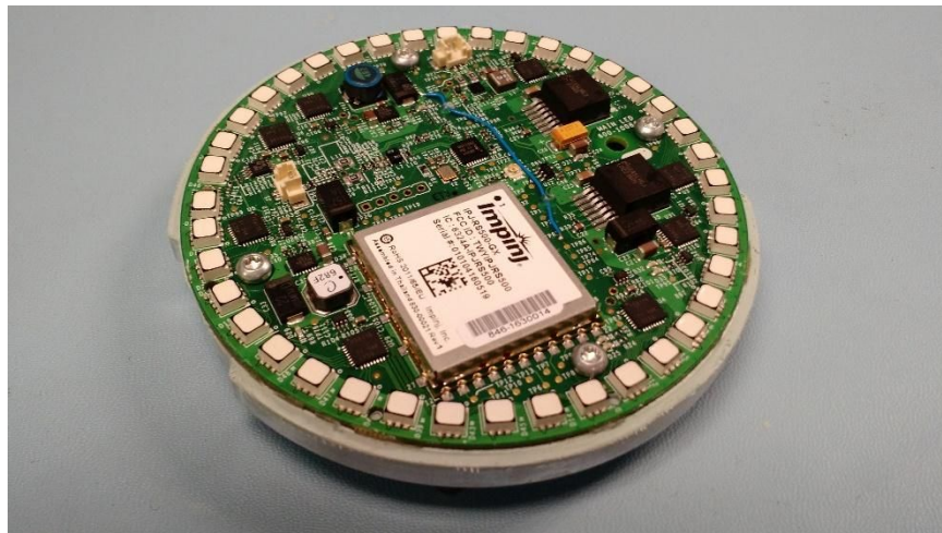
Main PCB and Heat Spreader(same as TPv2)
