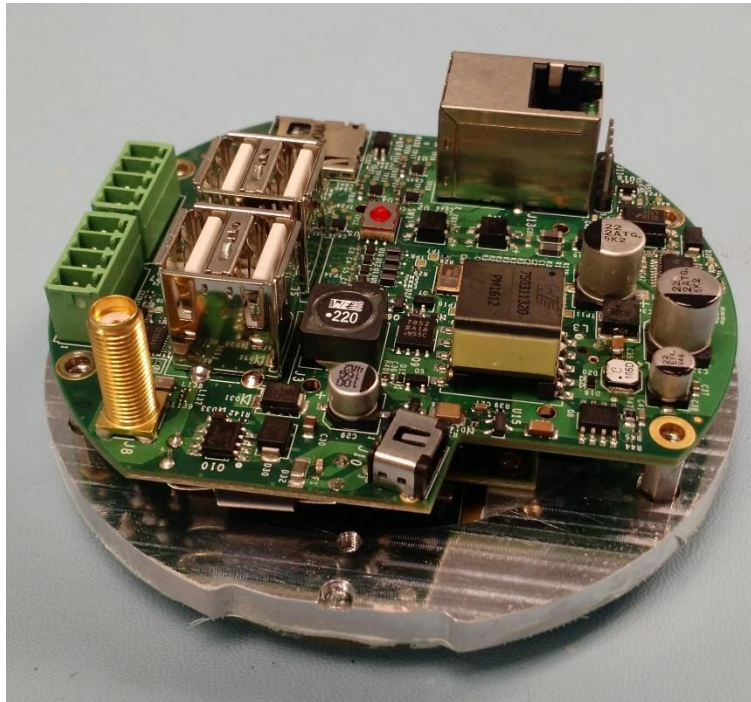
Main PCBA + Heat Spreader + Daughter PCBA(same as TPv2)
