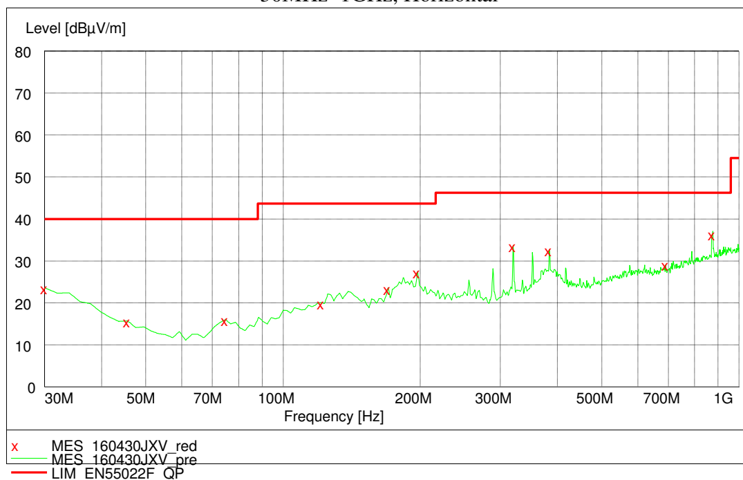
30MHz~1GHz, Horizontal
