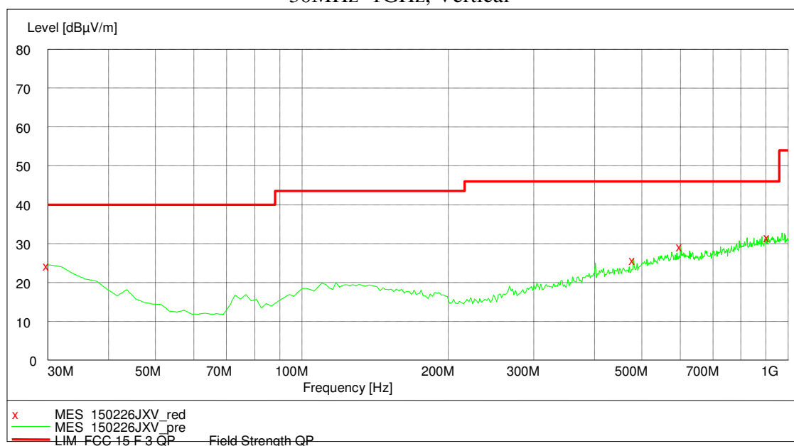
30MHz~1GHz, Vertical
