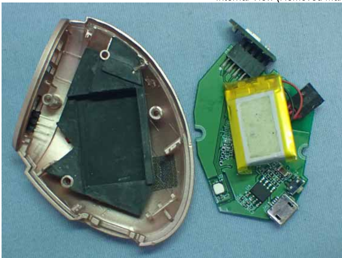
Figure 7 Internal View (Removed Main Board)
