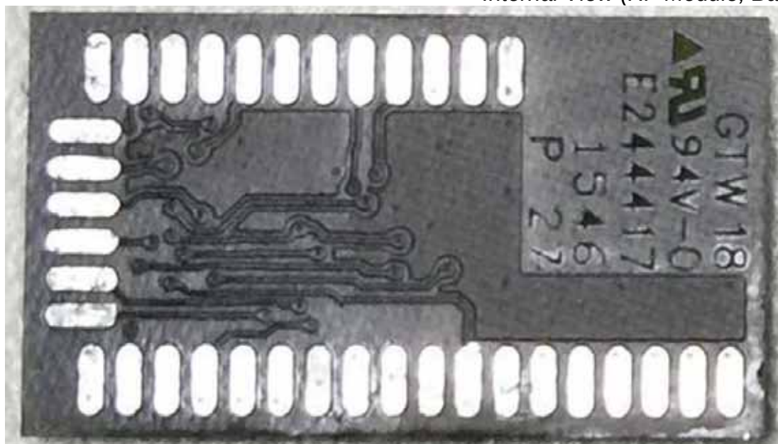
Figure 15 Internal View (RF Module, Back View)
