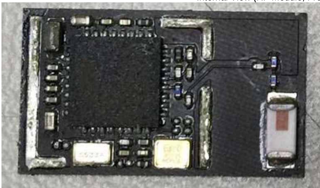
Figure 14 Internal View (RF Module, Front View)
