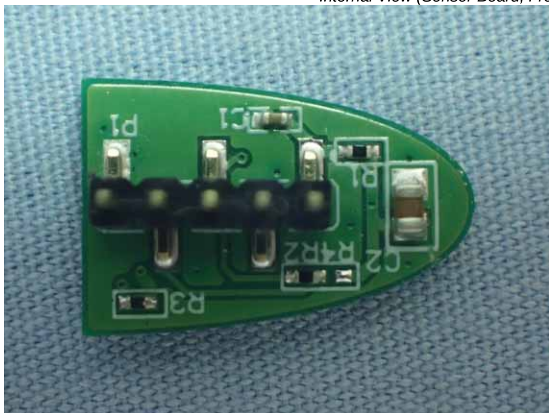
Figure 12 Internal View (Sensor Board, Front View)
