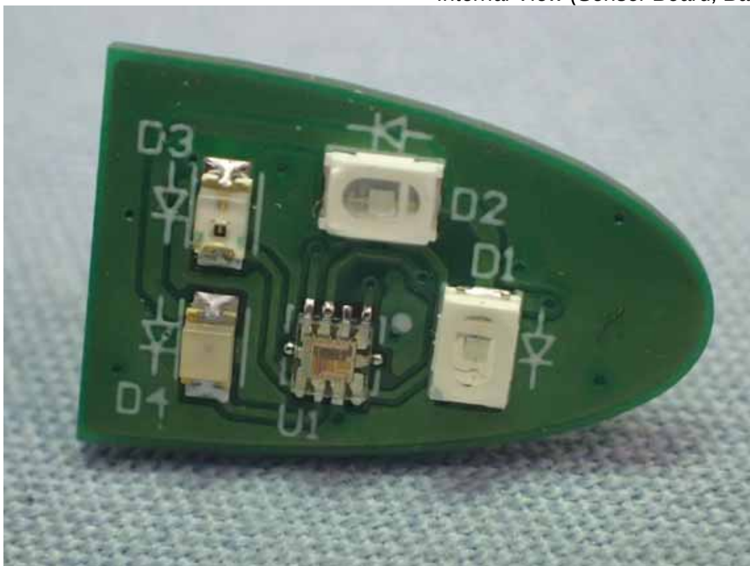
Figure 13 Internal View (Sensor Board, Back View)
