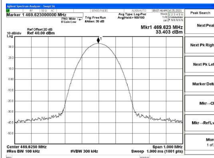
Channel 20 / 469.625 MHz
