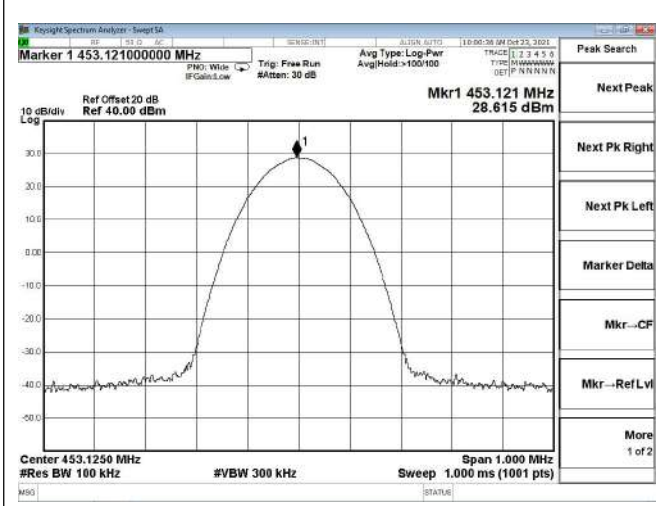
Channel 27 / 453.125 MHz
