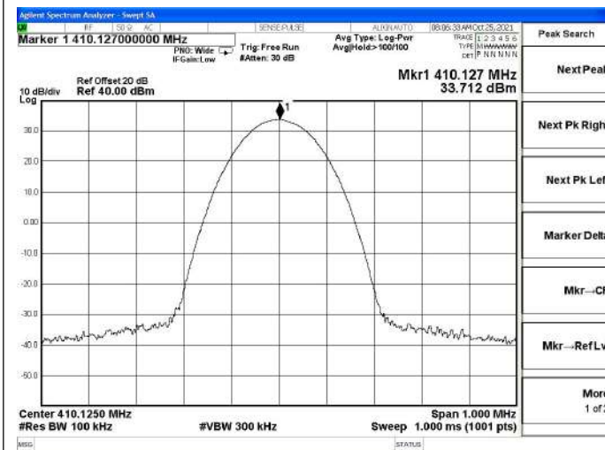
Channel 101 / 410.125 MHz
