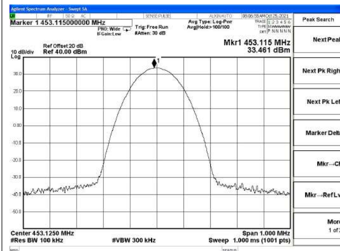
Channel 27 / 453.125 MHz
