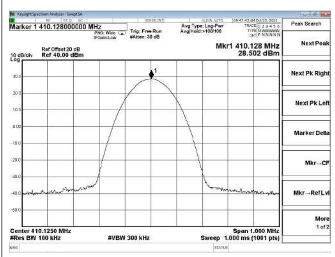
Channel 101/ 410.125 MHz
