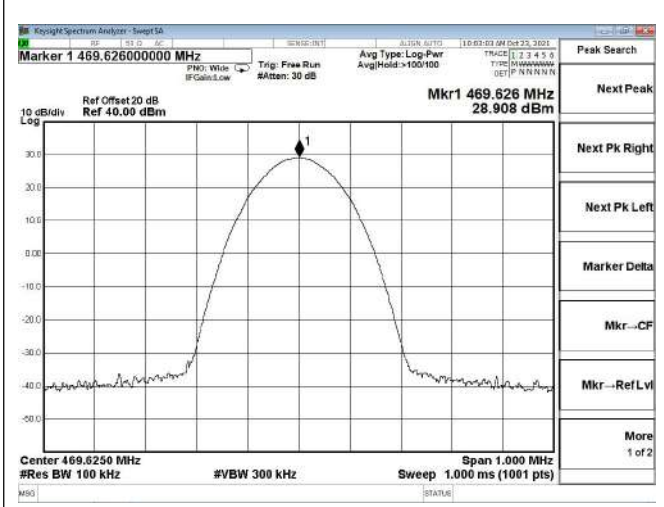
Channel 20 / 469.625 MHz
