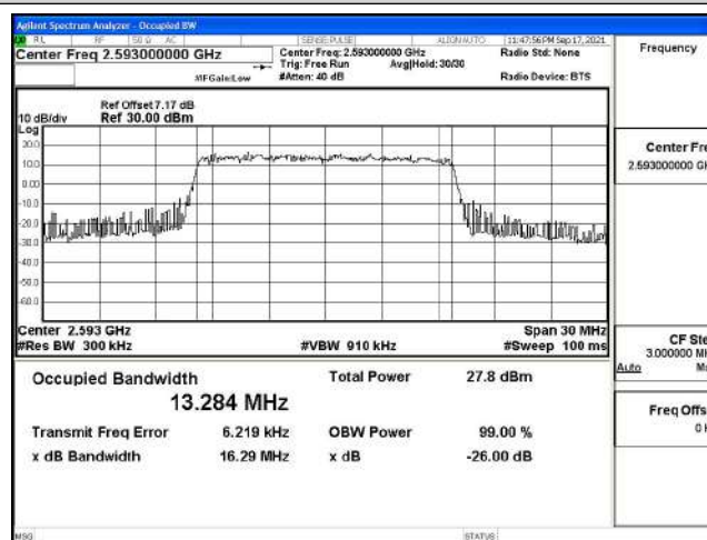
Band41-15MHz-16QAM-41515-75RB#0
