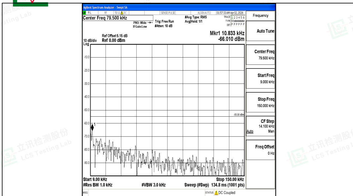
Band7_20MHz_QPSK_20850_1RB#0_0.009~0.15_0.009~0.15
