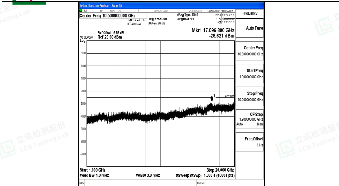
Band7_20MHz_16QAM_20850_1RB#0_1000~20000_1000~20000
