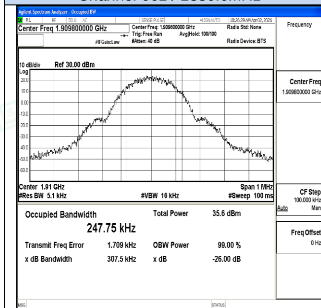
Channel 810 / 1909.8 MHz
