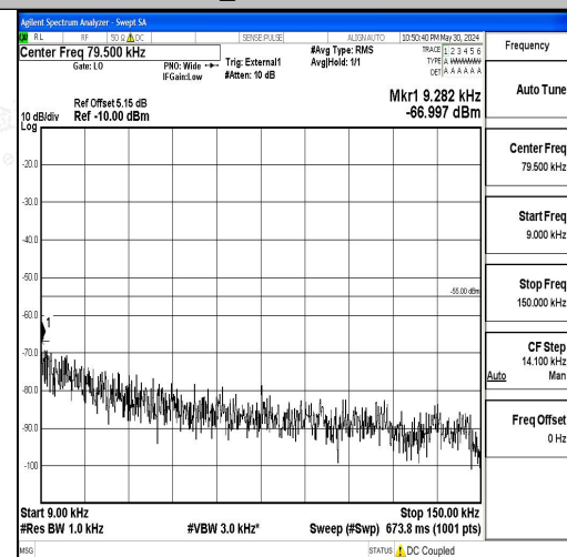
Band41_5MHz_16QAM_40620_1RB#0_0.009~0.15_5_0.009~0.15
