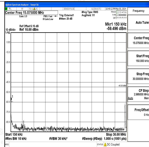
Band41_5MHz_QPSK_40620_1RB#0_0.15~30_0.15~30
