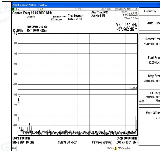
Band41_5MHz_16QAM_40620_1RB#0_0.15~30_0.15~30
