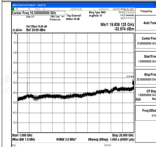
Band41_5MHz_16QAM_40620_1RB#0_1000~20000_1000~20000
