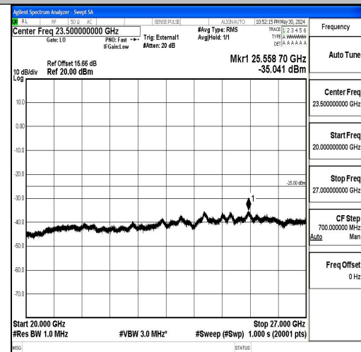
Band41_5MHz_16QAM_40620_1RB#0_20000~27000_000_1000~20000
