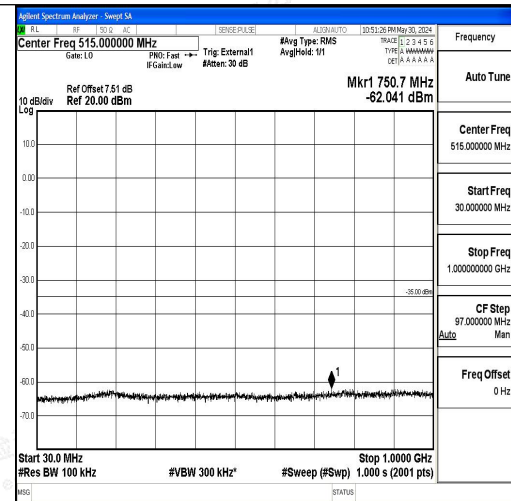
Band41_5MHz_16QAM_40620_1RB#0_30~1000_30~1000
