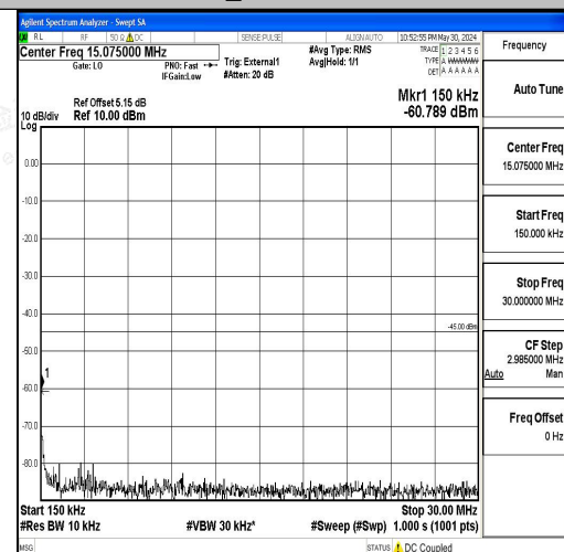
Band41_5MHz_QPSK_41565_1RB#0_0.15~30_0.15~30
