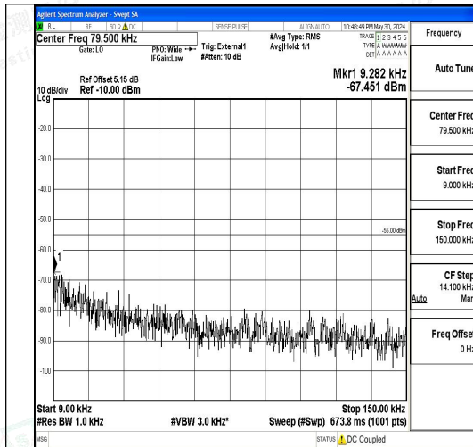
Band41_5MHz_QPSK_40620_1RB#0_0.009~0.15_5_0.009~0.15
