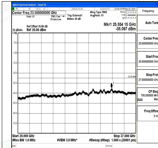
Band41_5MHz_QPSK_39675_1RB#0_20000~27000_20000~27000
