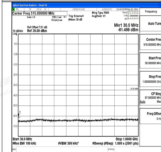
Band41_5MHz_QPSK_40620_1RB#0_30~1000_30~1000
