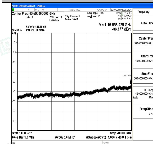
Band41_5MHz_16QAM_39675_1RB#0_1000~20000
