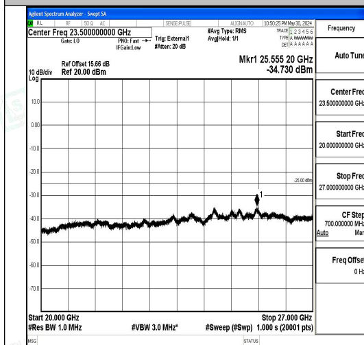
Band41_5MHz_QPSK_40620_1RB#0_20000~27000_000_20000~27000
