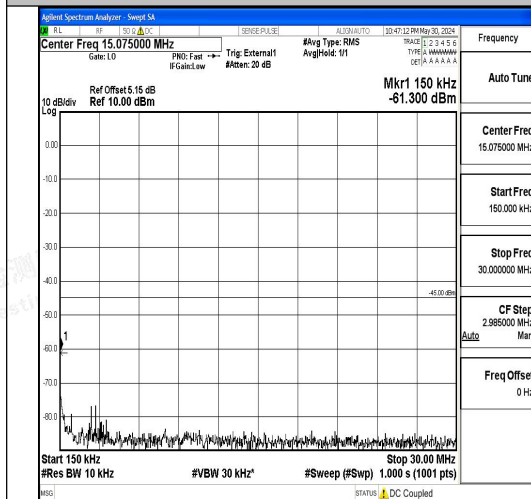
Band41_5MHz_16QAM_39675_1RB#0_0.15~30 0.15~30
