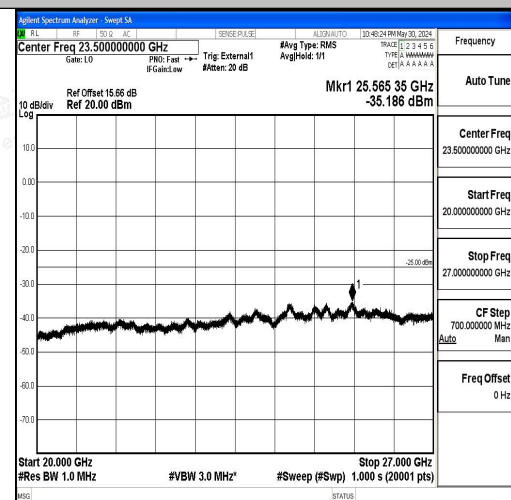
Band41_5MHz_16QAM_39675_1RB#0_20000~27000
