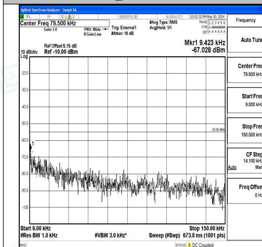
Band41_5MHz_QPSK_41565_1RB#0_0.009~0.1_5_0.009~0.15
