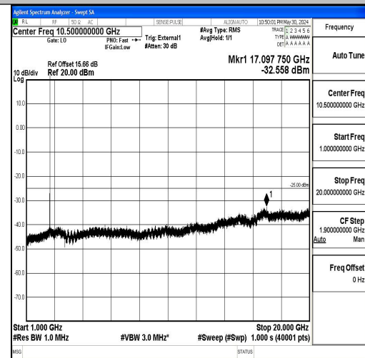
Band41_5MHz_QPSK_40620_1RB#0_1000~2000_0_1000~20000
