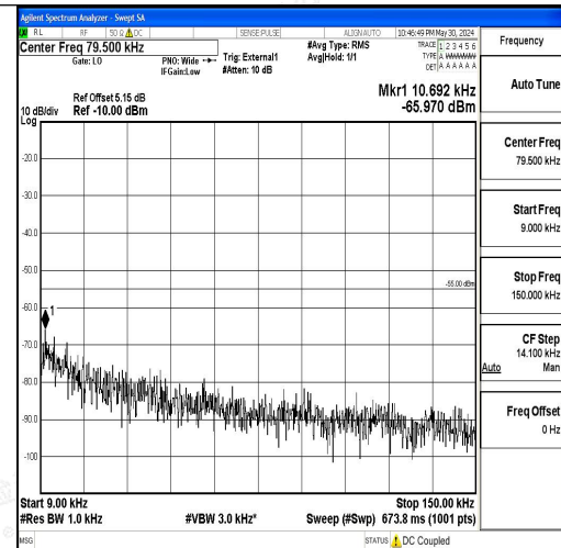
Band41_5MHz_16QAM_39675_1RB#0_0.009~0.1 5_0.009~0.15
