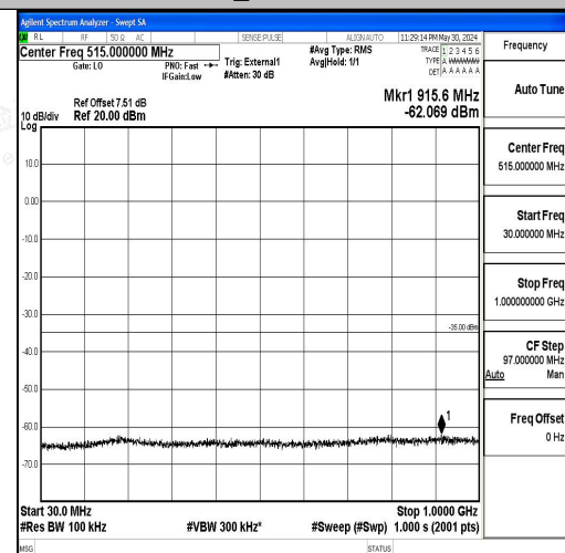
Band41_10MHz_16QAM_41540_1RB#0_30~1000_30~1000
