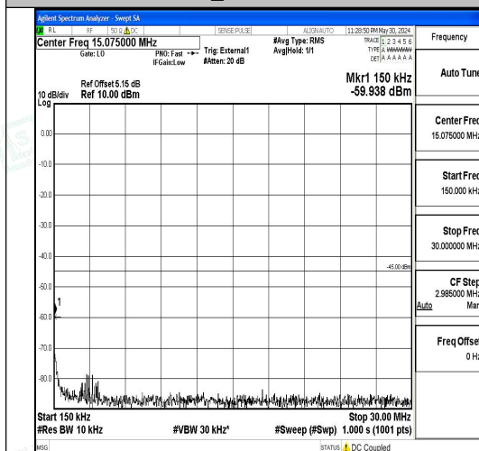
Band41_10MHz_16QAM_41540_1RB#0_0.15~30_0.15~30
