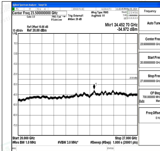
Band41_10MHz_QPSK_39700_1RB#0_20000~27000
