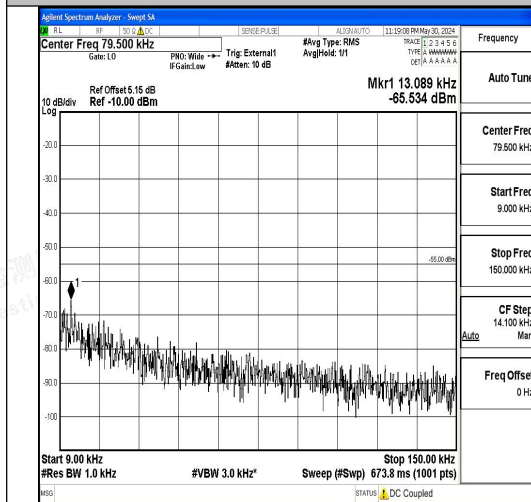
Band41_10MHz_QPSK_39700_1RB#0_0.009~0.15_0.009~0.15
