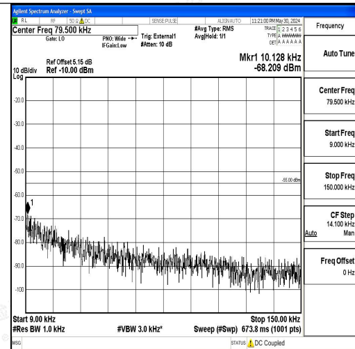
Band41_10MHz_16QAM_39700_1RB#0_0.009~0.15_0.009~0.15
