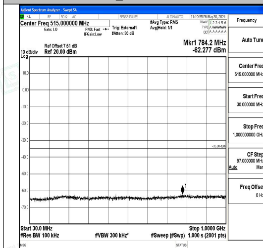
Band41_10MHz_QPSK_39700_1RB#0_30~1000_30~1000
