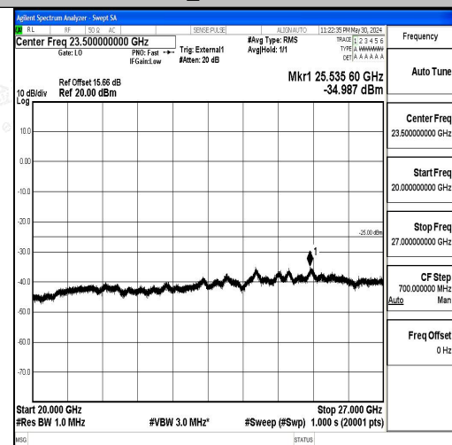
Band41_10MHz_16QAM_39700_1RB#0_20000~27000
