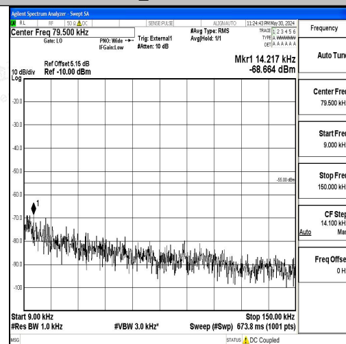
Band41_10MHz_16QAM_40620_1RB#0_0.009~0.15_0.009~0.15
