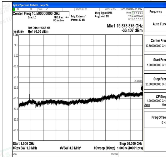
Band41_5MHz_16QAM_41565_1RB#0_1000~20000_000_1000~20000
