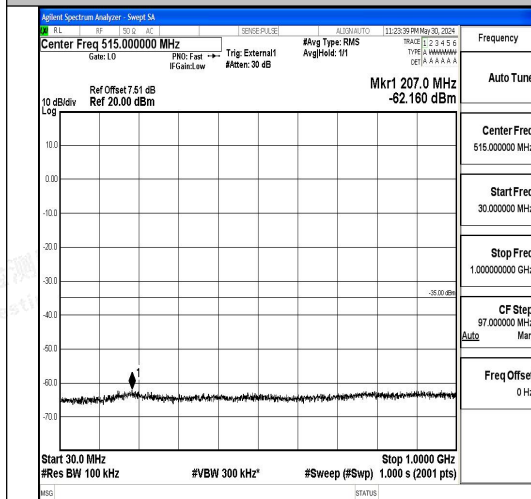
Band41_10MHz_QPSK_40620_1RB#0_30~1000_30~1000
