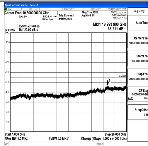
Band41_10MHz_QPSK_40620_1RB#0_1000~20000_1000~20000
