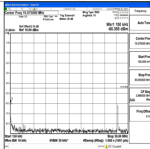
Band41_10MHz_QPSK_40620_1RB#0_0.15~30_0.15~30
