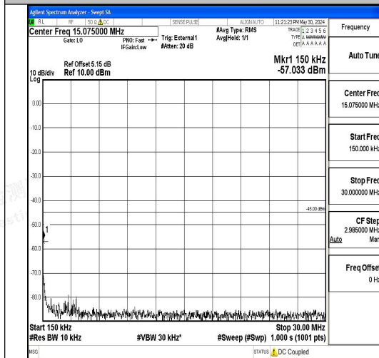
Band41_10MHz_16QAM_39700_1RB#0_0.15~30
