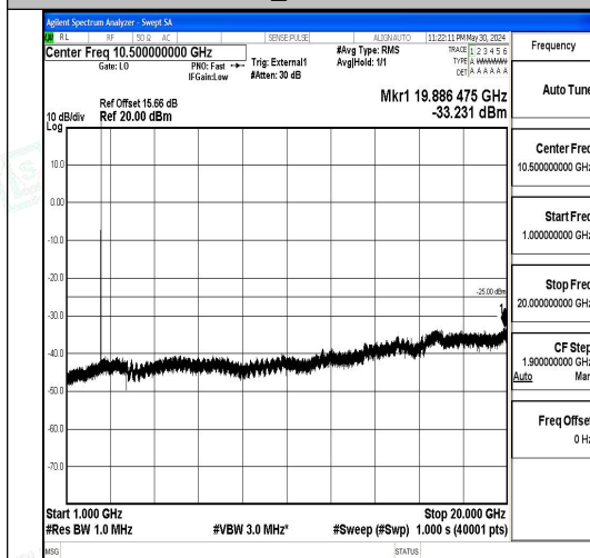
Band41_10MHz_16QAM_39700_1RB#0_1000~20000
