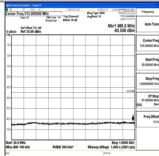
Band41_10MHz_16QAM_39700_1RB#0_30~1000 30~1000
