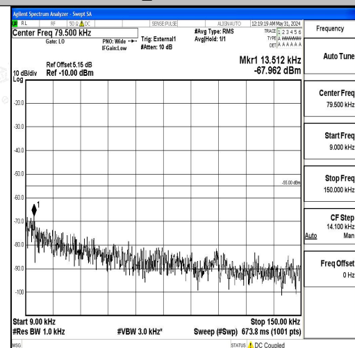
Band41_20MHz_16QAM_40620_1RB#0_0.009~0.15_0.009~0.15
