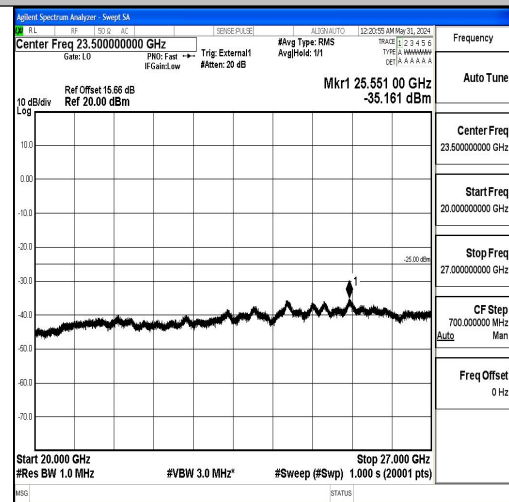
Band41_20MHz_16QAM_40620_1RB#0_2000~2 7000_20000~27000
