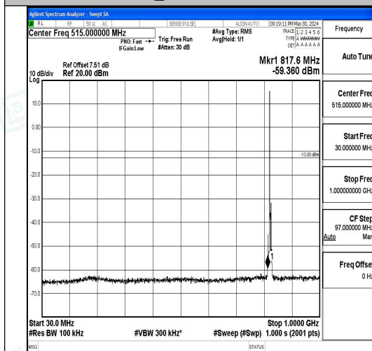
Band5_3MHz_QPSK_20415_1RB#0_30~1000
