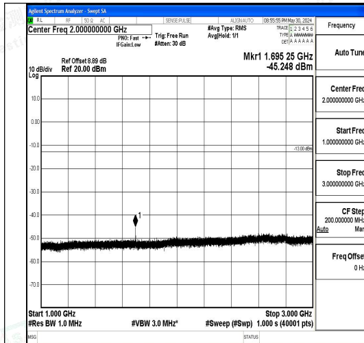
Band5_1.4MHz_16QAM_20643_1RB#0_1000~3000
