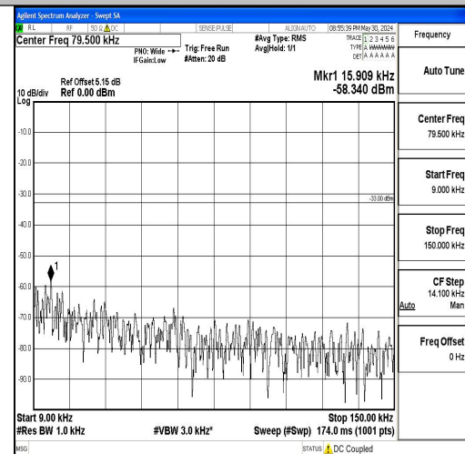
Band5_1.4MHz_16QAM_20643_1RB#0_0.009~0.15_15_0.009~0.15
