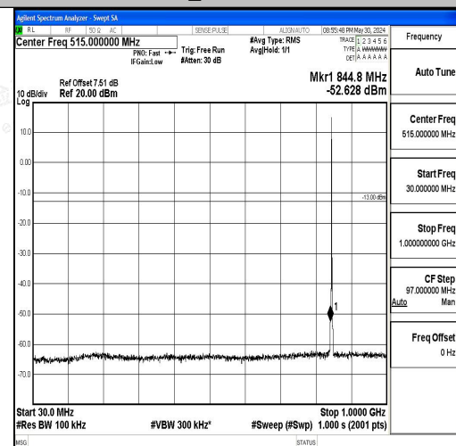
Band5_1.4MHz_16QAM_20643_1RB#0_30~1000_30~1000
