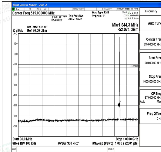
Band5_1.4MHz_QPSK_20643_1RB#0_30~1000_30~1000
