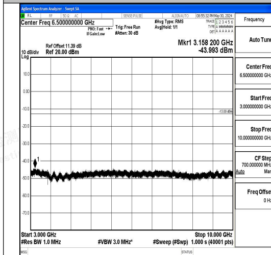
Band5_1.4MHz_QPSK_20643_1RB#0_3000~10000_00_3000~10000
