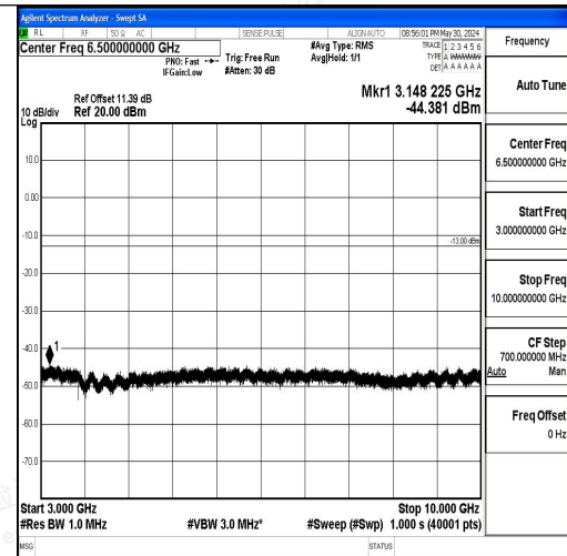
Band5_1.4MHz_16QAM_20643_1RB#0_3000~10000
