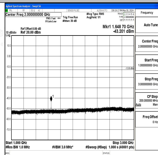
Band5_3MHz_QPSK_20415_1RB#0_1000~3000
