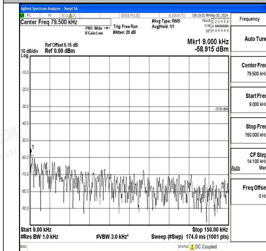
Band5_3MHz_QPSK_20415_1RB#0_0.009~0.15
