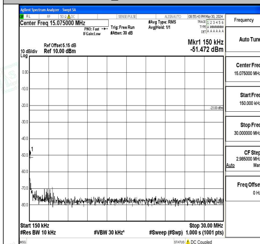
Band5_1.4MHz_16QAM_20643_1RB#0_0.15~30_0.15~30
