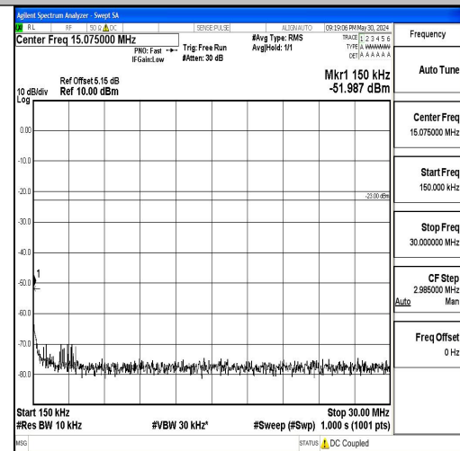
Band5_3MHz_QPSK_20415_1RB#0_0.15~30.0
