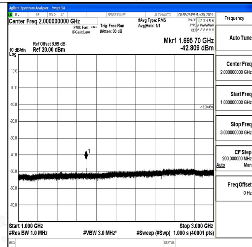
Band5_1.4MHz_QPSK_20643_1RB#0_1000~3000_0_1000~3000
