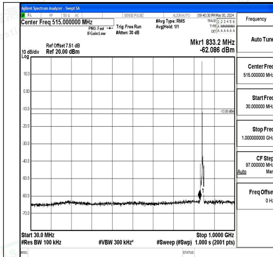
Band5_5MHz_QPSK_20625_1RB#0_30~1000_3 0~1000
