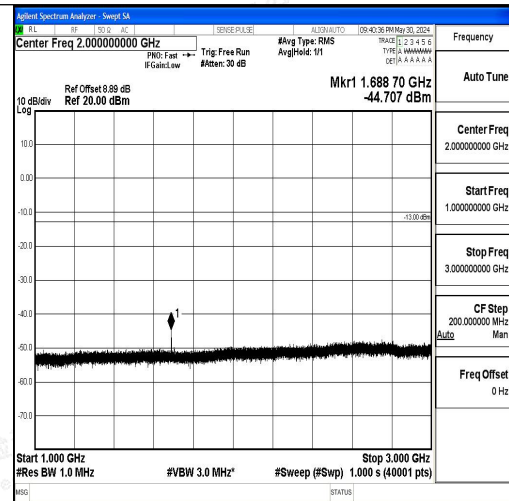
Band5_5MHz_QPSK_20625_1RB#0_1000~3000_ 1000~3000
