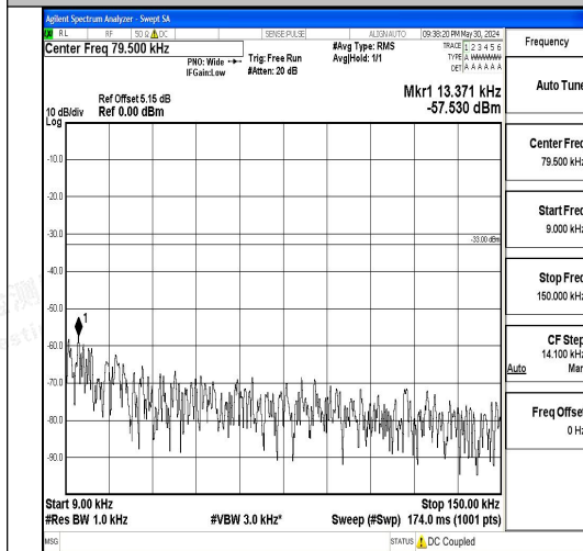
Band5_5MHz_QPSK_20425_1RB#0_0.009~0.15_0.009~0.15
