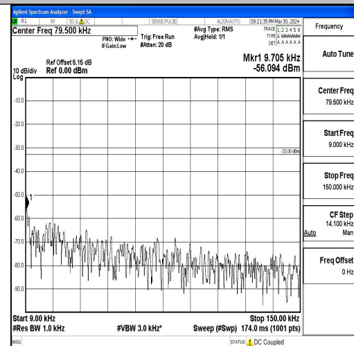
Band5_3MHz_16QAM_20635_1RB#0_0.009~0.15_0.009~0.15
