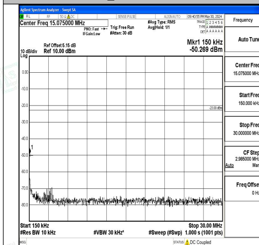
Band5_5MHz_16QAM_20625_1RB#0_0.15~30_ 0.15~30
