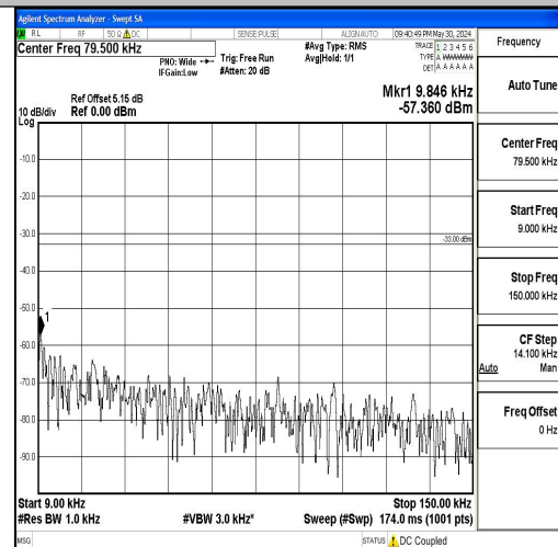
Band5_5MHz_16QAM_20625_1RB#0_0.009~0.15 _0.009~0.15
