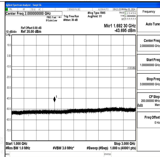
Band5_3MHz_QPSK_20635_1RB#0_1000~3000_1000~3000
