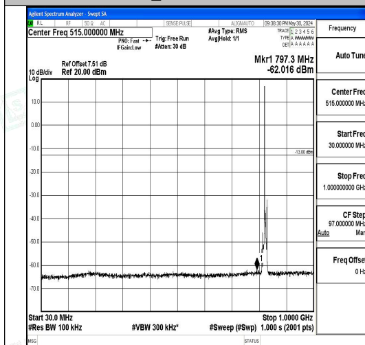
Band5_5MHz_QPSK_20425_1RB#0_30~1000_30~1000_0~1000
