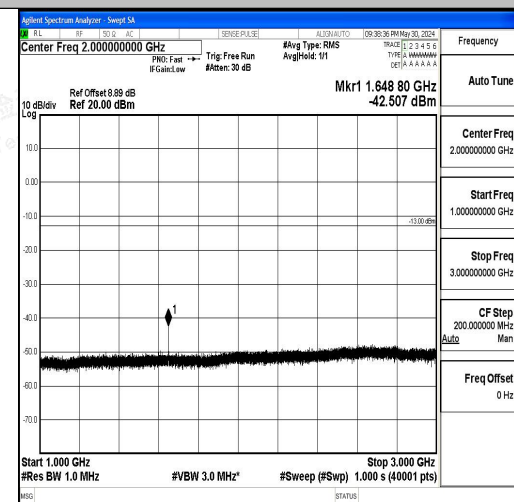
Band5_5MHz_QPSK_20425_1RB#0_1000~3000_1000~3000_1000~3000
