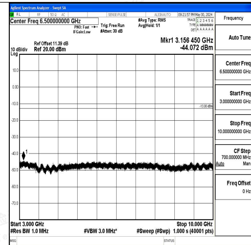
Band5_3MHz_16QAM_20635_1RB#0_3000~10000_0_3000~10000
