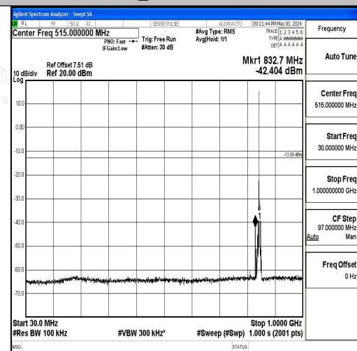
Band5_3MHz_16QAM_20635_1RB#0_30~1000_3_0~1000
