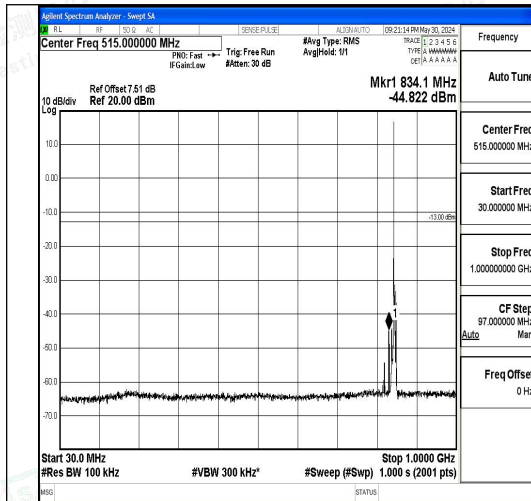
Band5_3MHz_QPSK_20635_1RB#0_30~1000_3 0~1000
