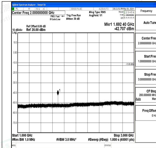
Band5_3MHz_16QAM_20635_1RB#0_1000~3000_1000~3000
