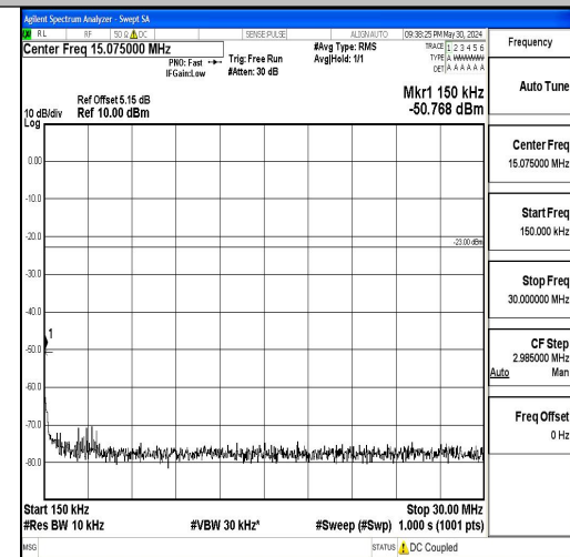
Band5_5MHz_QPSK_20425_1RB#0_0.15~30_0.15~30_5~30
