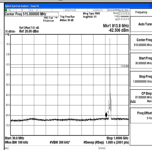
Band5_5MHz_16QAM_20625_1RB#0_30~1000_3 0~1000
