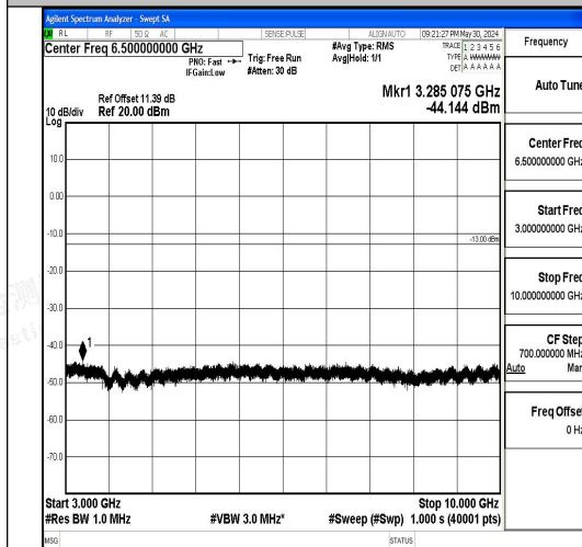
Band5_3MHz_QPSK_20635_1RB#0_3000~1000_0_3000~10000
