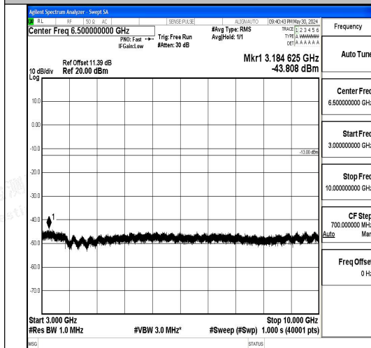
Band5_5MHz_QPSK_20625_1RB#0_3000~1000 0_3000~10000
