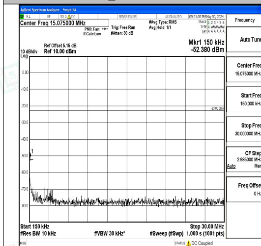
Band5_3MHz_16QAM_20635_1RB#0_0.15~30_0.15~30
