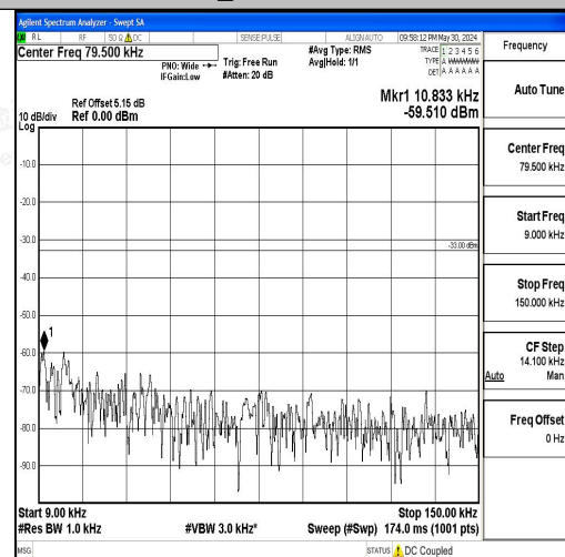
Band5_10MHz_16QAM_20525_1RB#0_0.009~0.1 5_0.009~0.15
