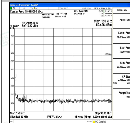
Band5_10MHz_16QAM_20600_1RB#0_0.15~30_0.15~30
