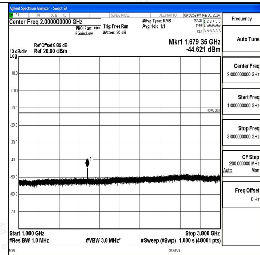
Band5_10MHz_QPSK_20600_1RB#0_1000~3000_1000~3000
