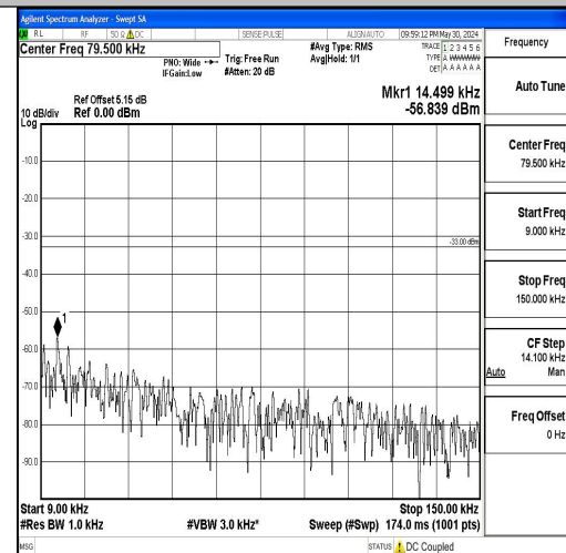
Band5_10MHz_16QAM_20600_1RB#0_0.009~0.15_5_0.009~0.15
