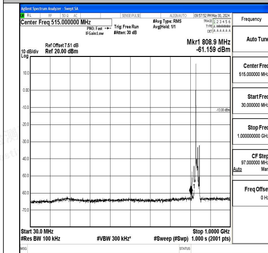
Band5_10MHz_QPSK_20525_1RB#0_30~1000_ 30~1000
