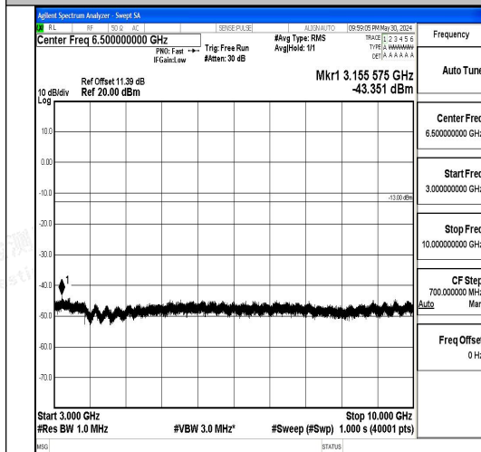
Band5_10MHz_QPSK_20600_1RB#0_3000~10000_00_3000~10000
