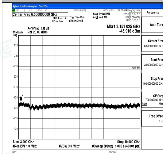
Band5_10MHz_QPSK_20525_1RB#0_3000~100 00_3000~10000
