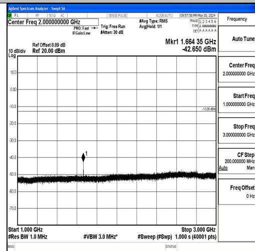
Band5_10MHz_QPSK_20525_1RB#0_1000~3000_ _1000~3000
