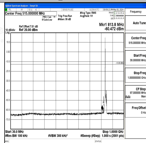
Band5_10MHz_16QAM_20600_1RB#0_30~1000_30~1000
