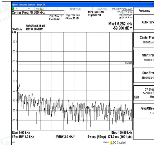
Band5_10MHz_QPSK_20525_1RB#0_0.009~0.15 5_0.009~0.15
