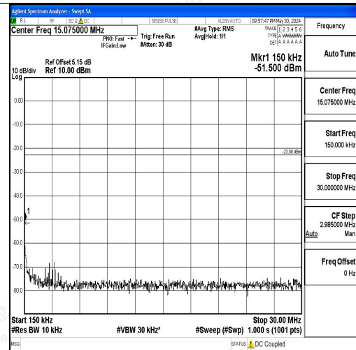
Band5_10MHz_QPSK_20525_1RB#0_0.15~30_0. 15~30
