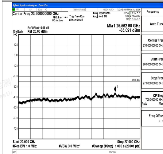
Band7_5MHz_QPSK_21425_1RB#0_20000~270 00_20000~27000
