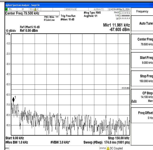
Band7_5MHz_16QAM_21425_1RB#0_0.009~0.15 _0.009~0.15
