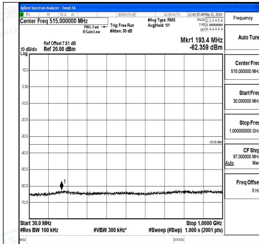
Band7_5MHz_QPSK_21425_1RB#0_30~1000_3 0~1000
