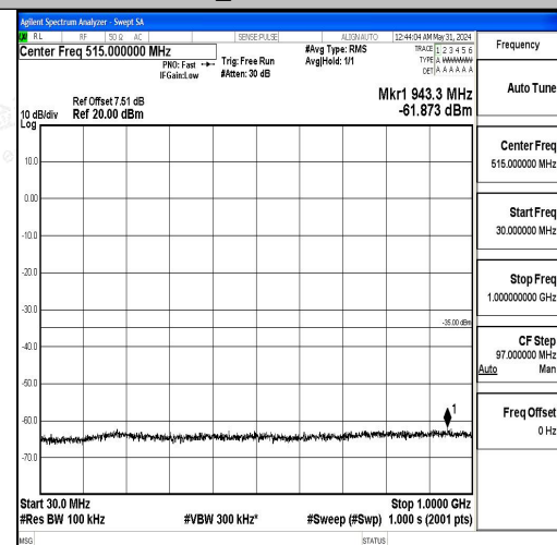
Band7_5MHz_16QAM_21425_1RB#0_30~1000_3 0~1000
