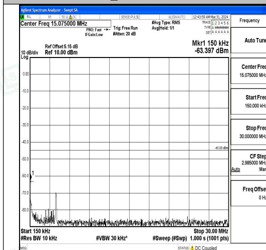
Band7_5MHz_16QAM_21425_1RB#0_0.15~30 0.15~30
