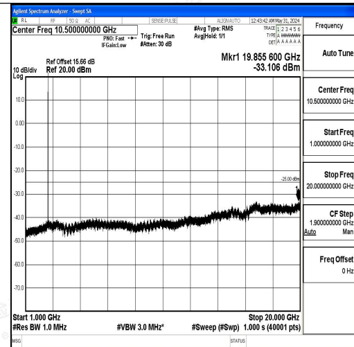
Band7_5MHz_QPSK_21425_1RB#0_1000~20000 _1000~20000
