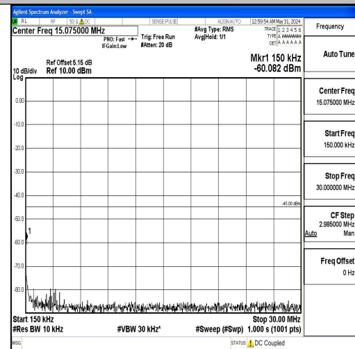
Band7_10MHz_QPSK_20800_1RB#0_0.15~30
