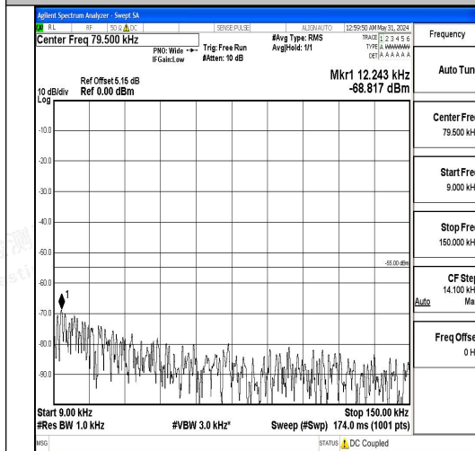
Band7_10MHz_QPSK_20800_1RB#0_0.009~0.15
