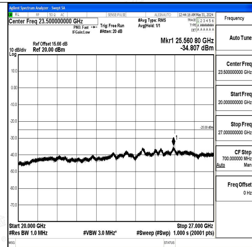
Band7_5MHz_16QAM_21425_1RB#0_20000~27000
