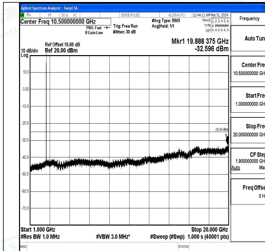
Band7_5MHz_16QAM_21425_1RB#0_1000~20000
