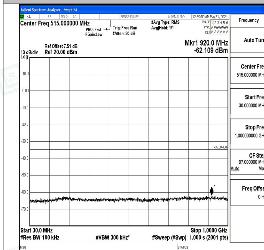
Band7_10MHz_QPSK_20800_1RB#0_30~1000
