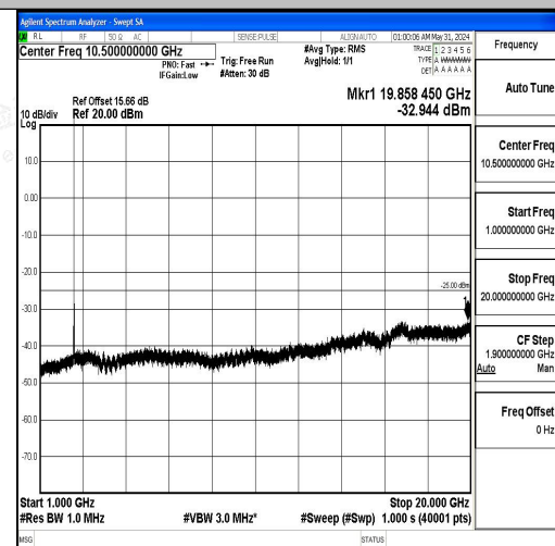
Band7_10MHz_QPSK_20800_1RB#0_1000~20000
