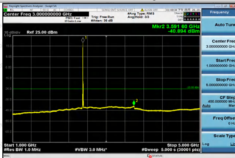
Band7-10MHz-QPSK-20800-1RB#0-Range3:5000~12000MHz
