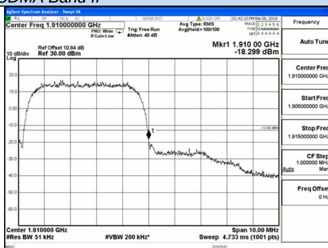
Channel 9538 / 1907.6 MHz
