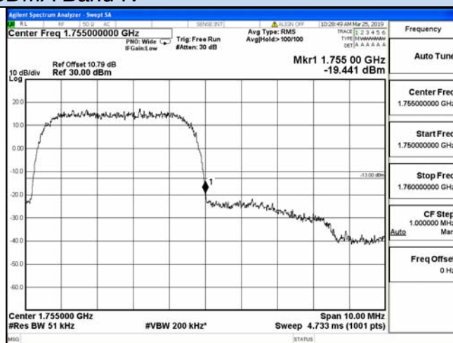
Channel 1512 / 1752 MHz
