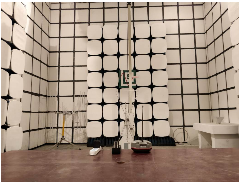
Below 1GHz
