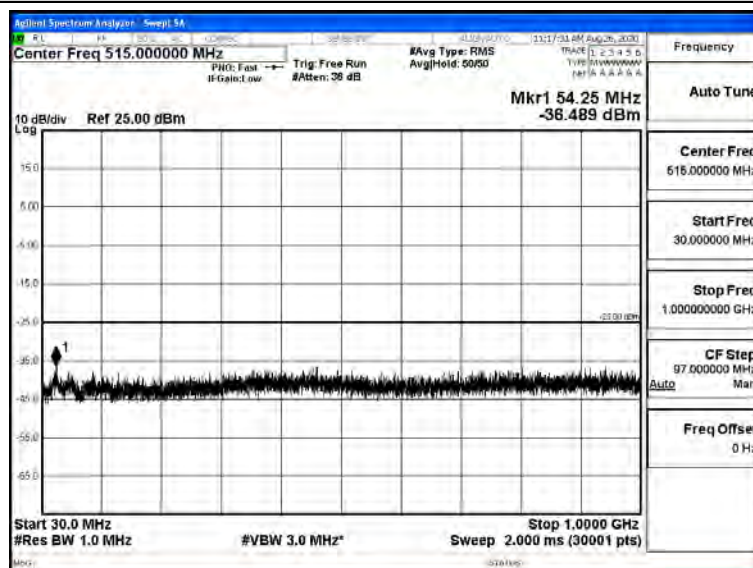
Band41-20MHz-QPSK-40620-1RB#0-Range3:30~1000MHz
