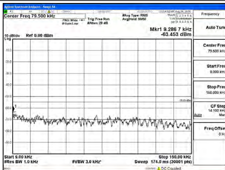
Band41-20MHz-16QAM-39750-1RB#0-Range1:0.009~0.15MHz
