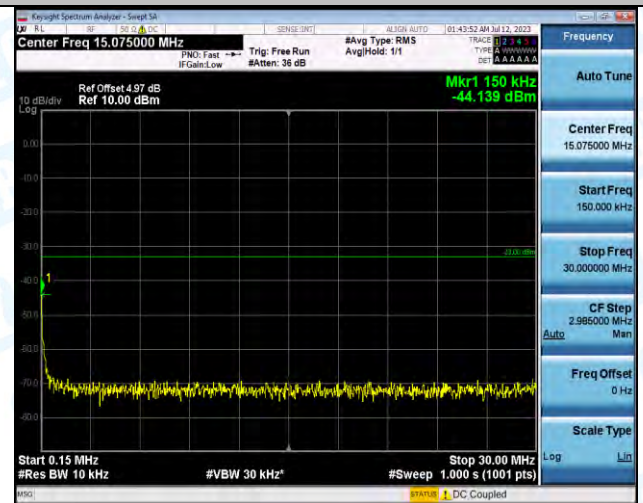
Band2-9538-2-0.15~30MHz-PASS
