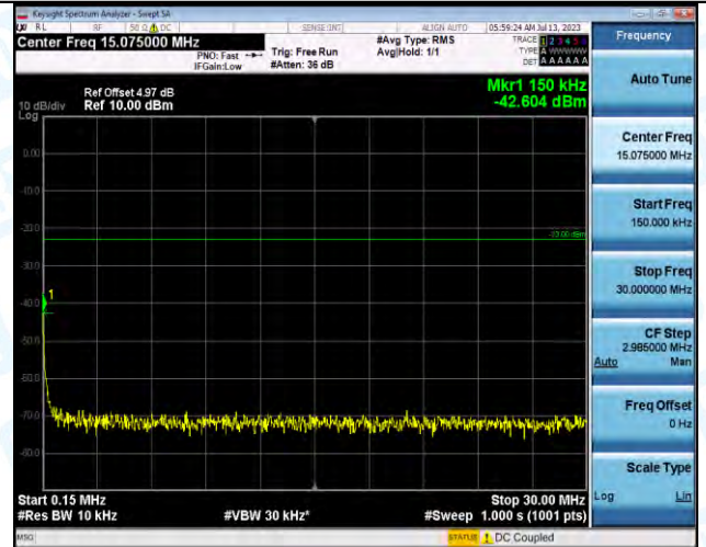
Band5-4233-0.15~30MHz-PASS
