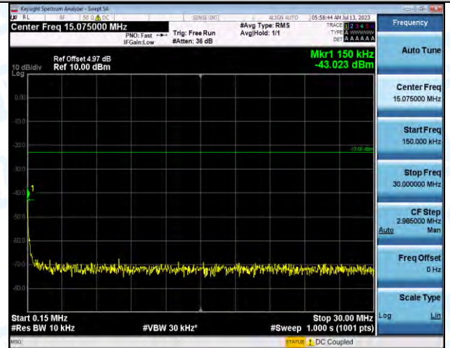
Band5-4182-0.15~30MHz-PASS
