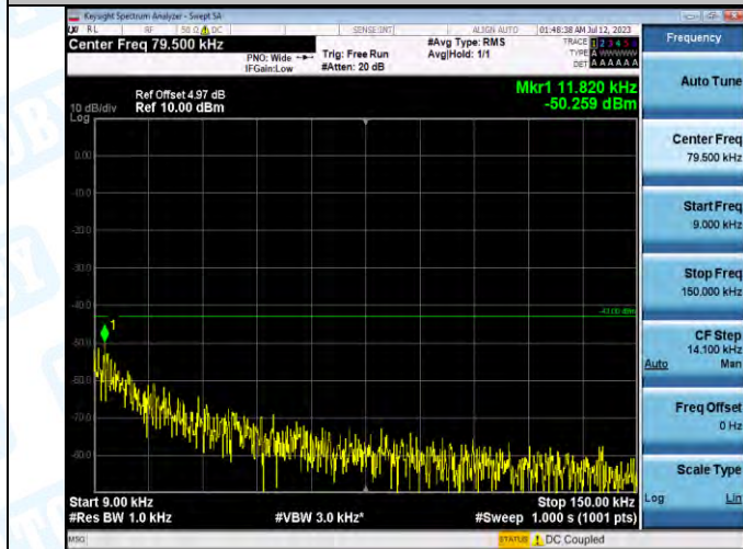
Band2-9400-4-0.009~0.15MHz-PASS
