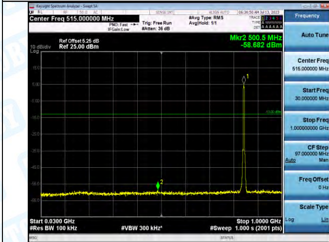
Band5-4233-1-30~1000MHz-PASS
