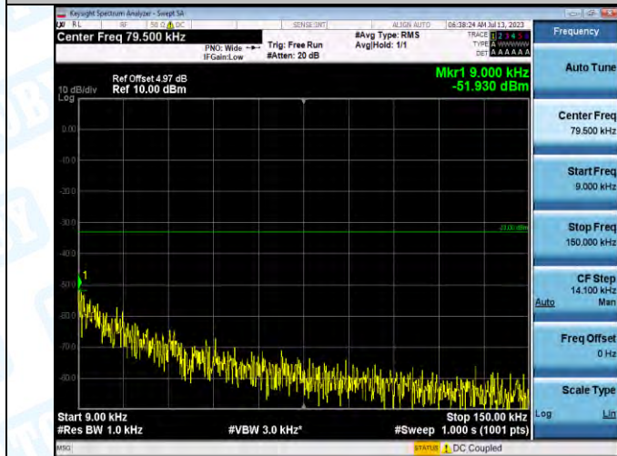
Band5-4182-2-0.009~0.15MHz-PASS
