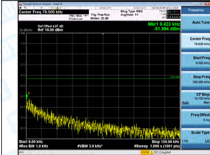
Band5-4233-1-0.009~0.15MHz-PASS
