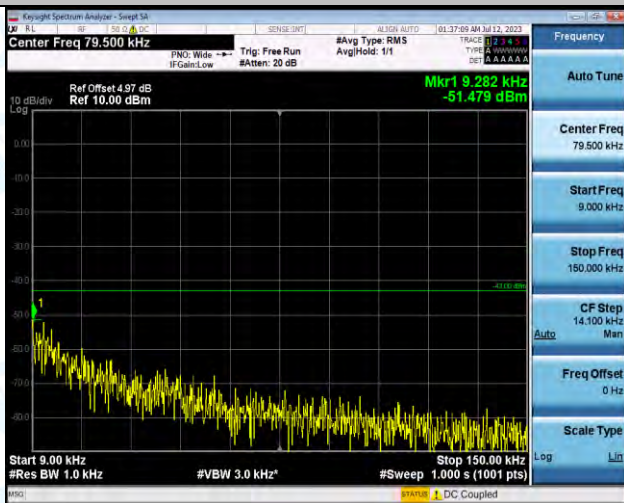
Band2-9538-0.009~0.15MHz-PASS
