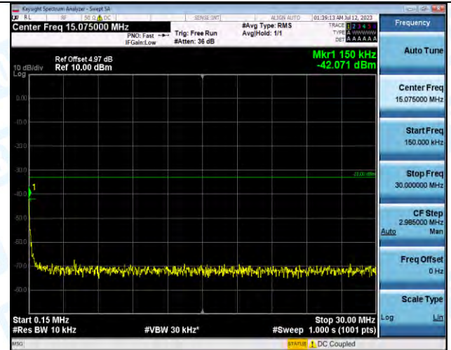
Band2-9262-1-0.15~30MHz-PASS
