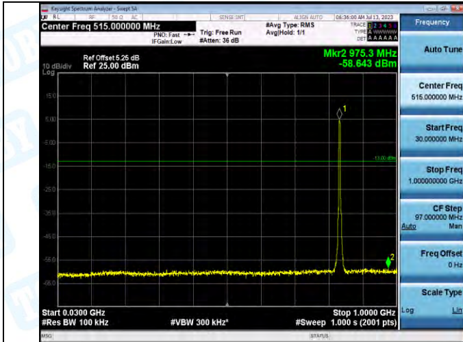
Band5-4182-1-30~1000MHz-PASS
