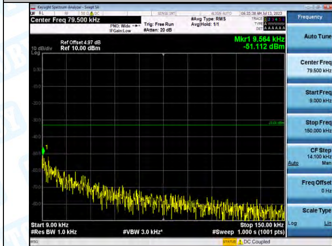
Band5-4182-1-0.009~0.15MHz-PASS
