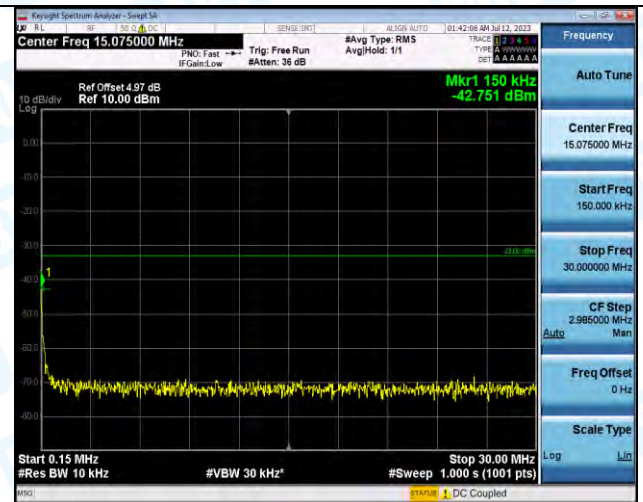
Band2-9262-2-0.15~30MHz-PASS
