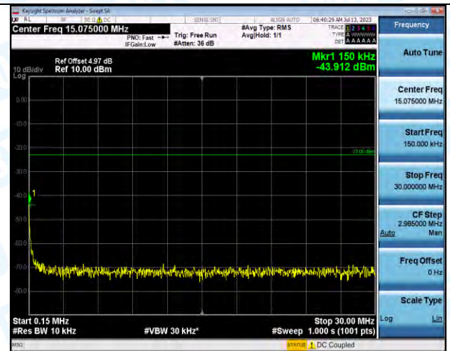
Band5-4132-3-0.15~30MHz-PASS
