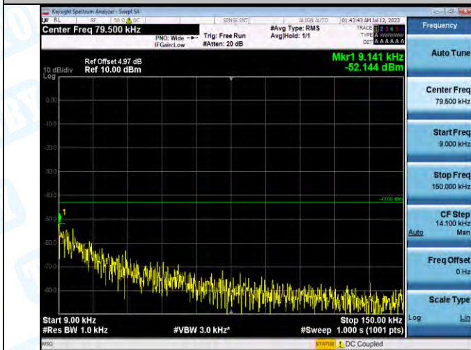
Band2-9538-2-0.009~0.15MHz-PASS
