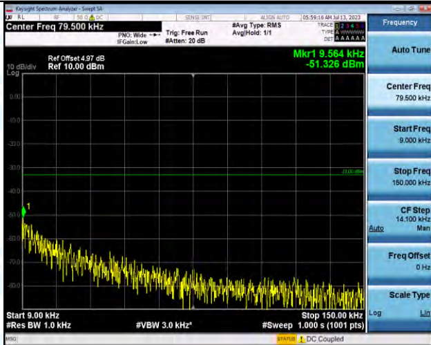
Band5-4233-0.009~0.15MHz-PASS
