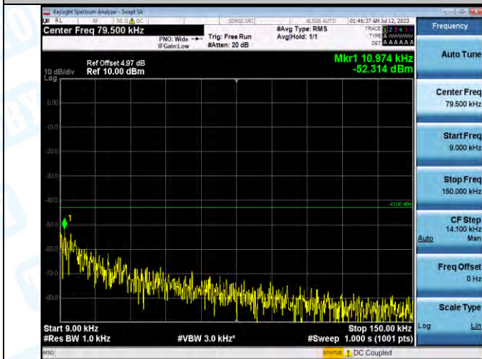
Band2-9538-3-0.009~0.15MHz-PASS
