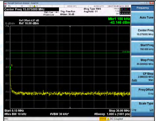
Band5-4132-2-0.15~30MHz-PASS
