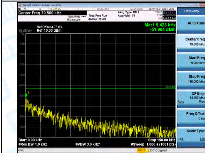
Band2-9538-1-0.009~0.15MHz-PASS
