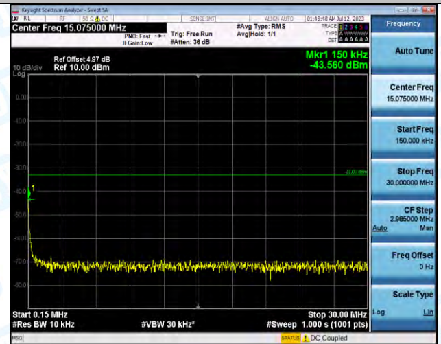
Band2-9400-4-0.15~30MHz-PASS
