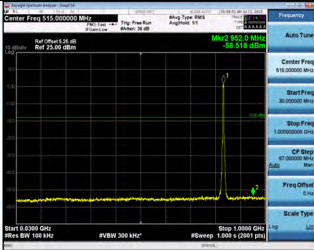
Band5-4182-30~1000MHz-PASS
