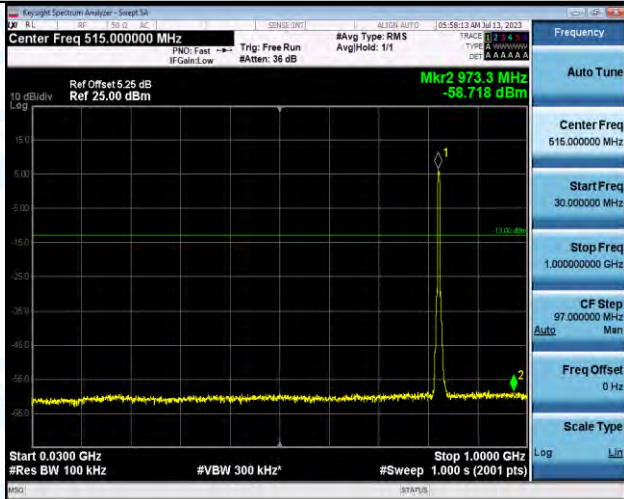
Band5-4132-30~1000MHz-PASS
