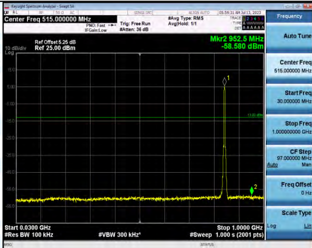
Band5-4233-30~1000MHz-PASS
