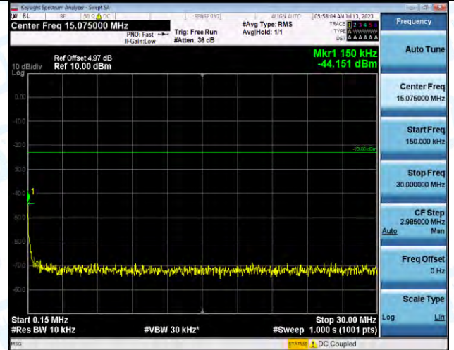
Band5-4132-0.15~30MHz-PASS
