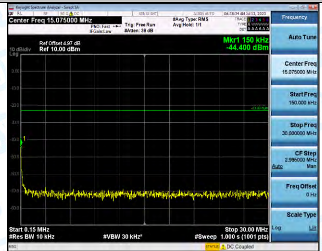
Band5-4182-2-0.15~30MHz-PASS
