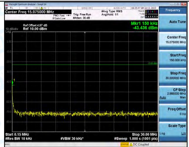
Band5-4182-1-0.15~30MHz-PASS
