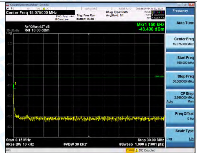
Band2-9262-3-0.15~30MHz-PASS
