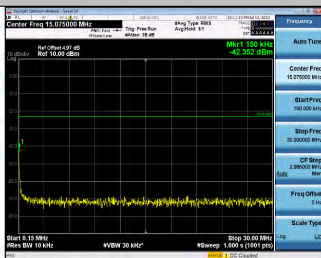
Band5-4182-3-0.15~30MHz-PASS
