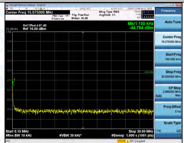
Band2-9400-5-0.15~30MHz-PASS
