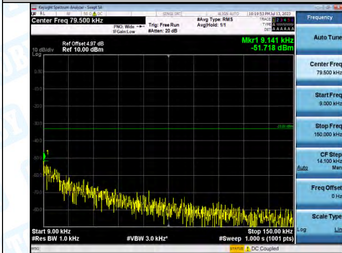
Band5-4182-5-0.009~0.15MHz-PASS
