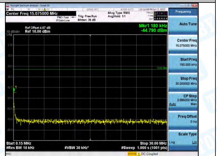
Band5-4182-4-0.15~30MHz-PASS
