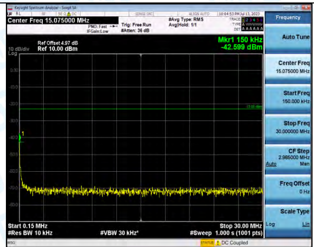
Band5-4132-2-0.15~30MHz-PASS
