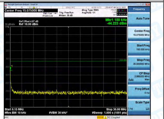
Band2-9538-4-0.15~30MHz-PASS
