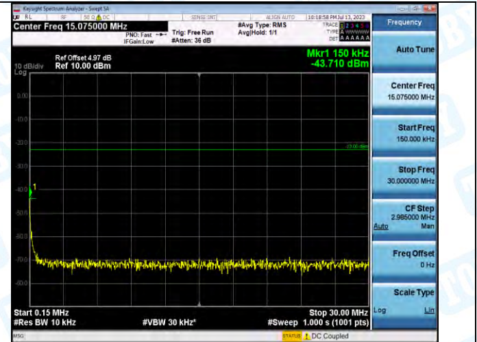
Band5-4132-5-0.15~30MHz-PASS
