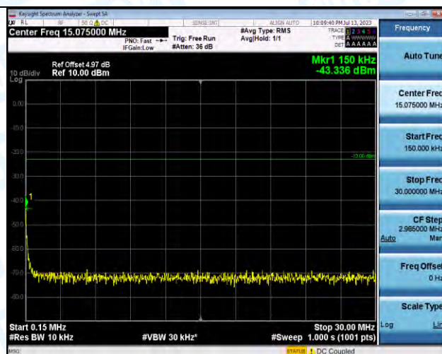
Band5-4132-3-0.15~30MHz-PASS
