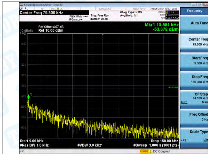
Band2-9262-1-0.009~0.15MHz-PASS
