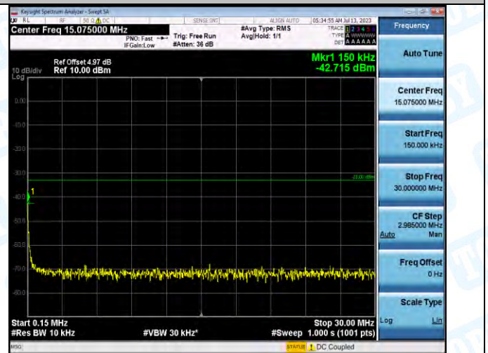
Band2-9538-2-0.15~30MHz-PASS
