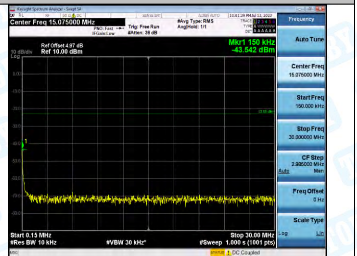
Band5-4182-1-0.15~30MHz-PASS
