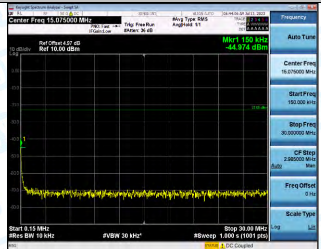
Band5-4182-4-0.15~30MHz-PASS
