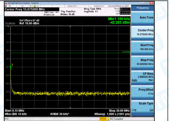
Band5-4132-4-0.15~30MHz-PASS
