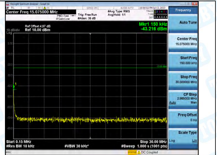
Band5-4132-1-0.15~30MHz-PASS
