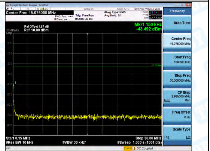
Band5-4233-2-0.15~30MHz-PASS
