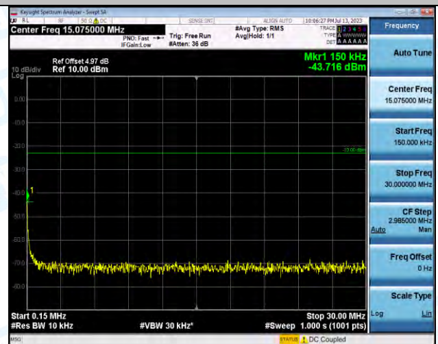
Band5-4182-2-0.15~30MHz-PASS
