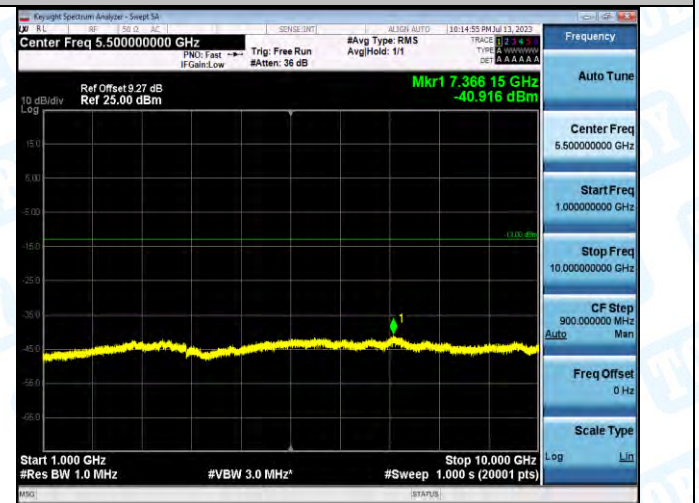
Band5-4132-4-1000~10000MHz-PASS
