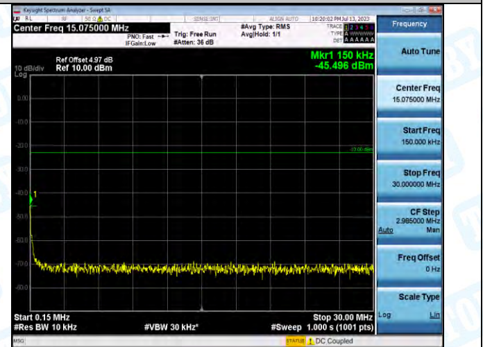
Band5-4182-5-0.15~30MHz-PASS
