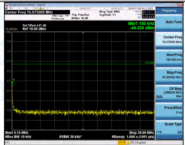
Band5-4233-4-0.15~30MHz-PASS
