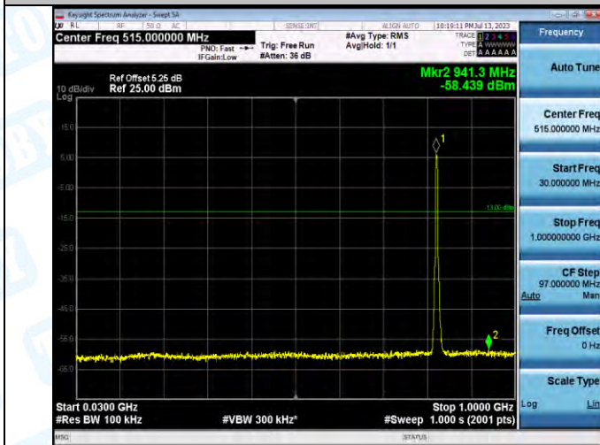
Band5-4132-5-30~1000MHz-PASS
