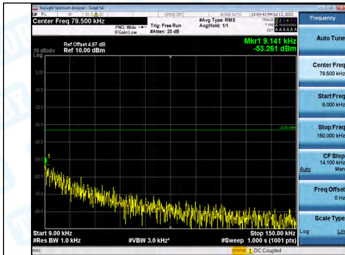
Band5-4132-2-0.009~0.15MHz-PASS
