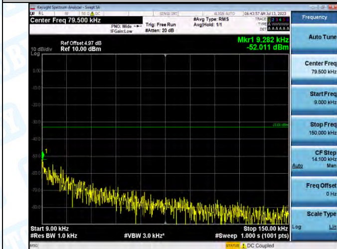
Band5-4182-4-0.009~0.15MHz-PASS
