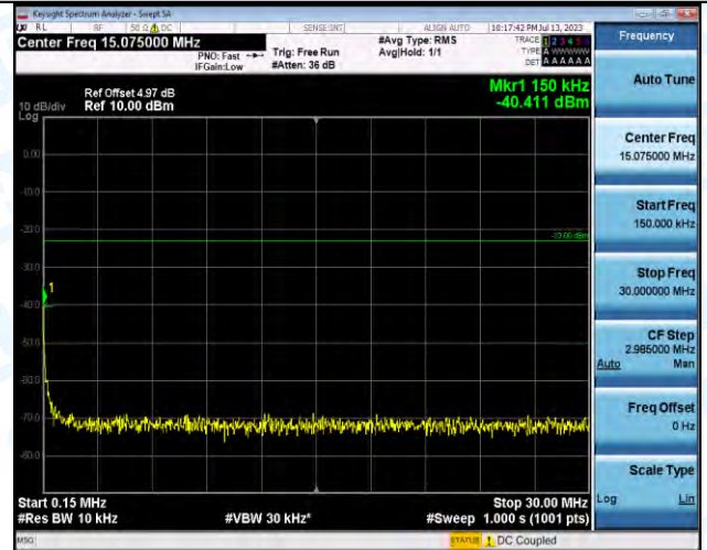
Band5-4233-4-0.15~30MHz-PASS
