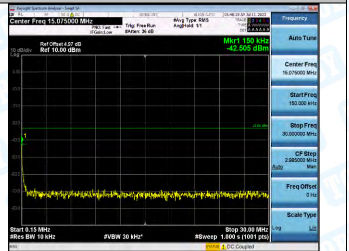
Band2-9538-5-0.15~30MHz-PASS
