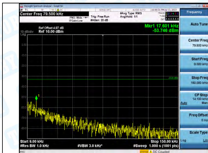
Band5-4132-3-0.009~0.15MHz-PASS
