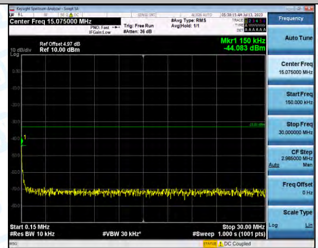
Band2-9400-3-0.15~30MHz-PASS
