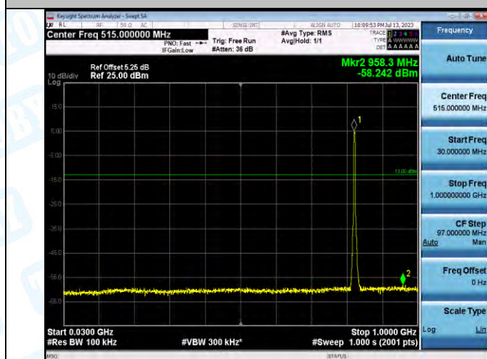
Band5-4132-3-30~1000MHz-PASS
