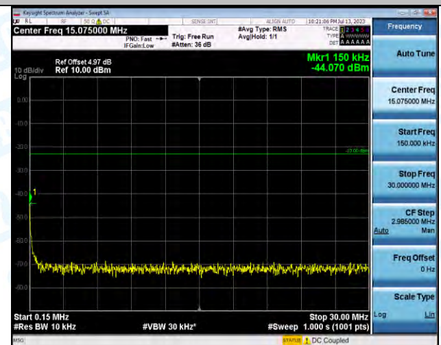
Band5-4233-5-0.15~30MHz-PASS
