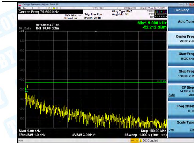
Band2-9262-4-0.009~0.15MHz-PASS
