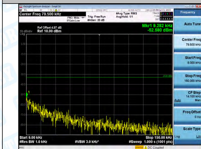
Band5-4182-3-0.009~0.15MHz-PASS
