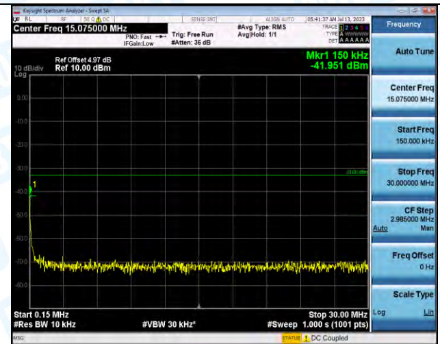
Band2-9262-4-0.15~30MHz-PASS
