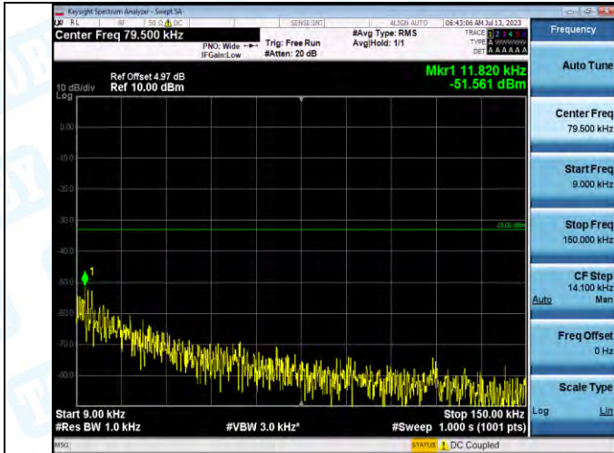
Band5-4132-4-0.009~0.15MHz-PASS
