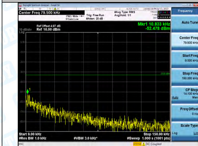
Band5-4182-2-0.009~0.15MHz-PASS
