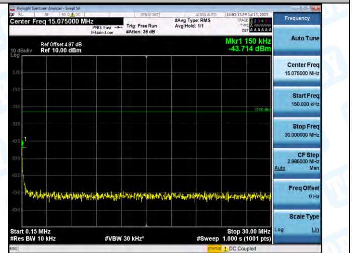
Band5-4233-1-0.15~30MHz-PASS
