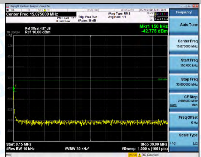
Band2-9400-1-0.15~30MHz-PASS
