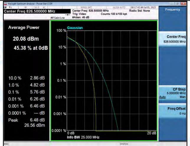
Band5-5MHz-16QAM-20425-25RB#0-PASS
