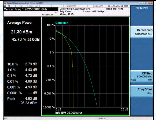
Band2-15MHz-16QAM-19125-1RB#0-PASS
