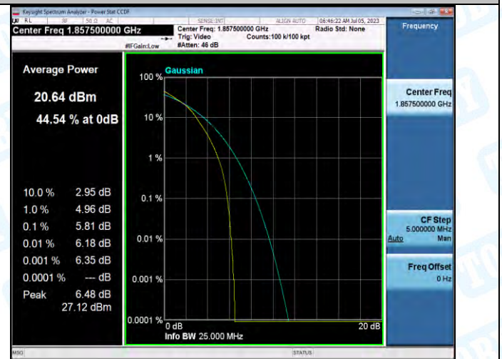
Band2-15MHz-16QAM-18675-75RB#0-PASS
