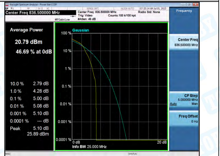
Band5-1.4MHz-16QAM-20525-1RB#0-PASS
