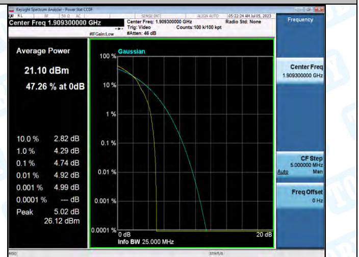
Band2-1.4MHz-16QAM-19193-1RB#0-PASS
