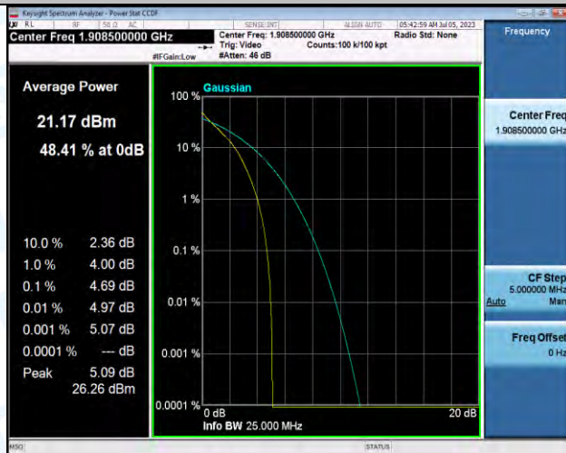
Band2-3MHz-QPSK-19185-15RB#0-PASS
