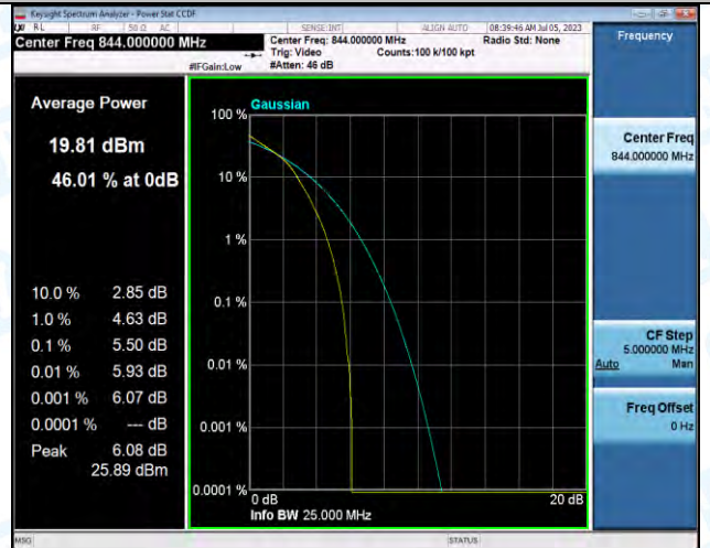
Band5-10MHz-16QAM-20600-50RB#0-PASS
