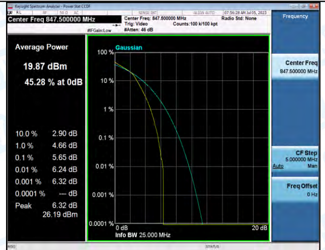
Band5-3MHz-16QAM-20635-15RB#0-PASS
