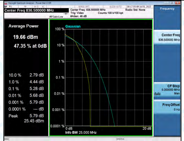
Band5-5MHz-16QAM-20525-25RB#0-PASS
