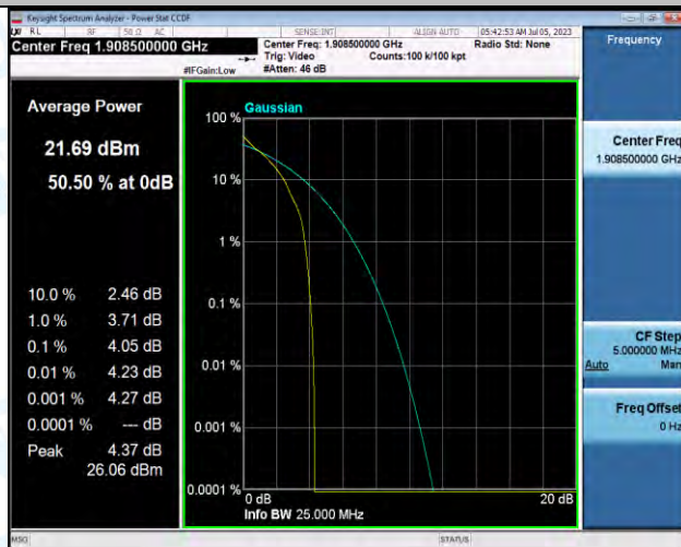
Band2-3MHz-QPSK-19185-1RB#0-PASS
