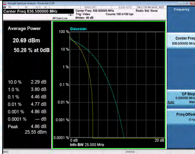
Band5-5MHz-QPSK-20525-25RB#0-PASS
