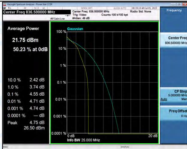
Band5-10MHz-QPSK-20525-1RB#0-PASS
