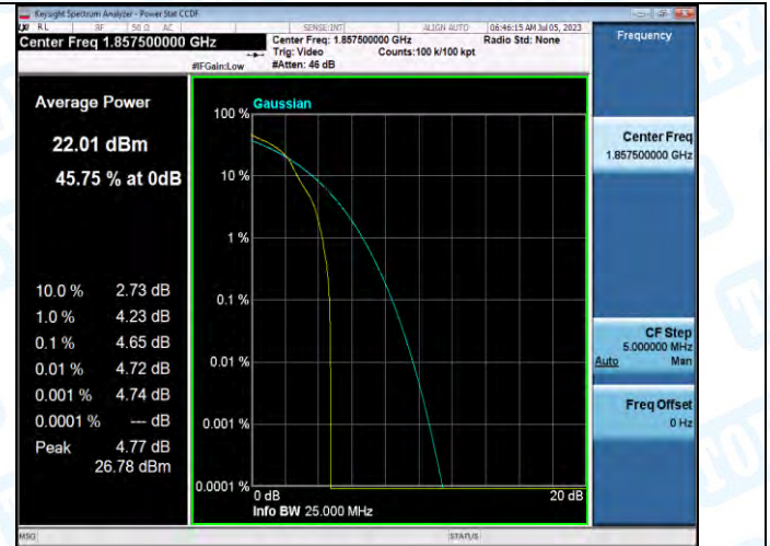
Band2-15MHz-16QAM-18675-1RB#0-PASS
