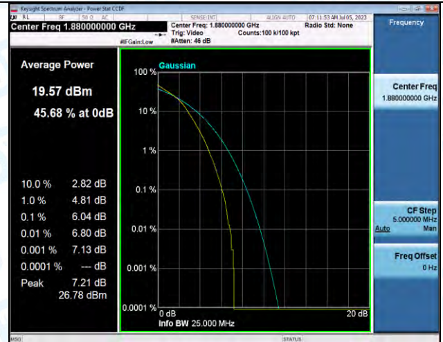
Band2-20MHz-16QAM-18900-100RB#0-PASS
