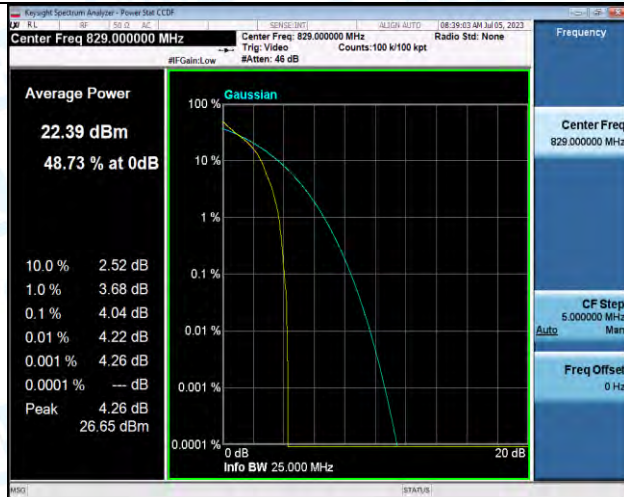
Band5-10MHz-QPSK-20450-1RB#0-PASS
