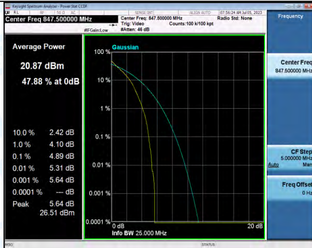
Band5-3MHz-QPSK-20635-15RB#0-PASS
