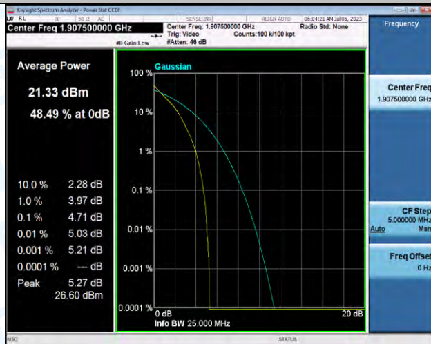
Band2-5MHz-QPSK-19175-25RB#0-PASS
