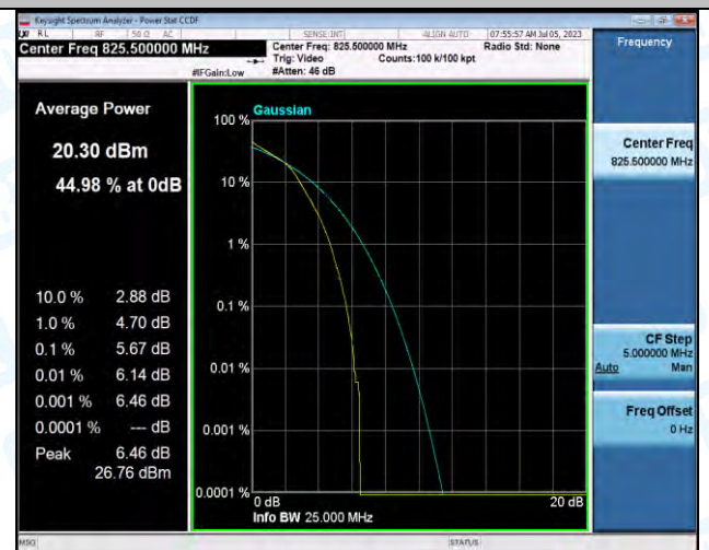
Band5-3MHz-16QAM-20415-15RB#0-PASS
