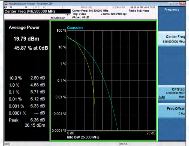
Band5-5MHz-16QAM-20625-25RB#0-PASS
