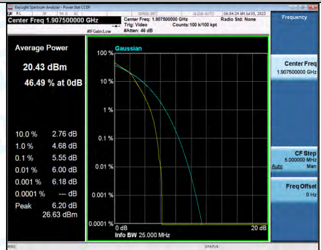
Band2-5MHz-16QAM-19175-25RB#0-PASS
