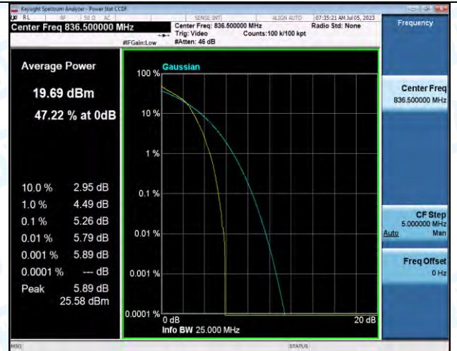
Band5-1.4MHz-16QAM-20525-6RB#0-PASS
