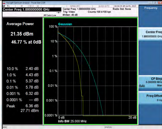
Band2-15MHz-QPSK-18900-75RB#0-PASS
