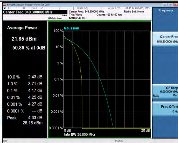
Band5-1.4MHz-QPSK-20643-1RB#0-PASS
