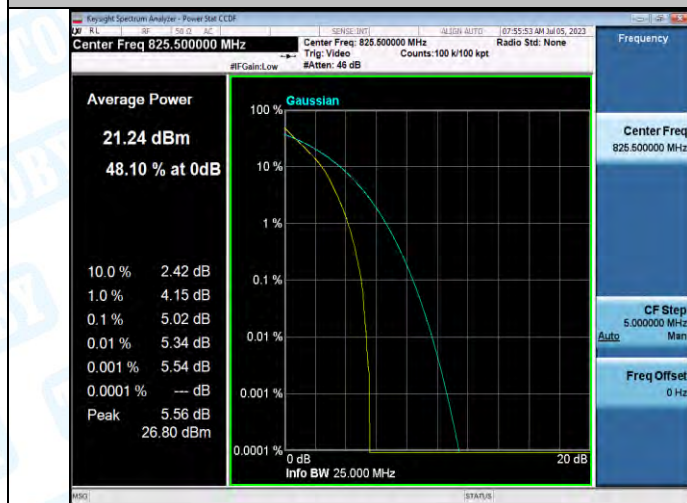
Band5-3MHz-QPSK-20415-15RB#0-PASS
