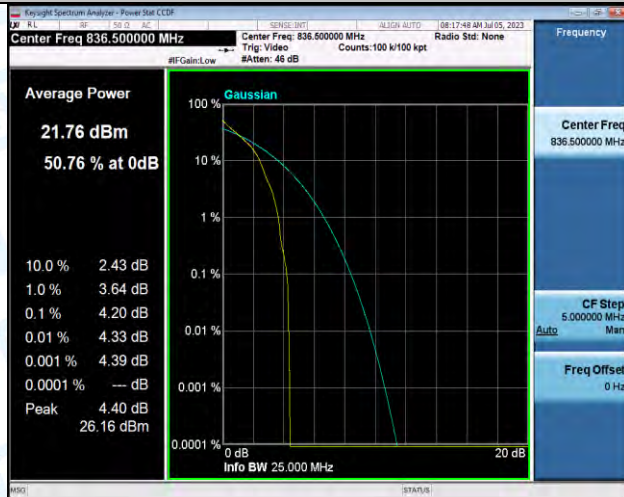
Band5-5MHz-QPSK-20525-1RB#0-PASS
