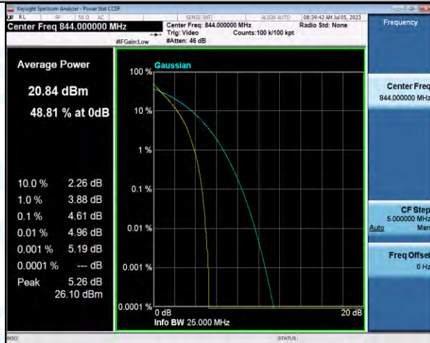
Band5-10MHz-QPSK-20600-50RB#0-PASS
