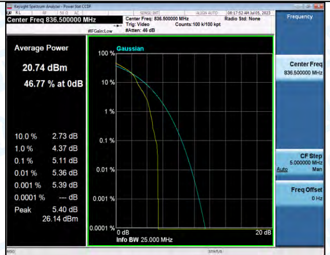
Band5-5MHz-16QAM-20525-1RB#0-PASS
