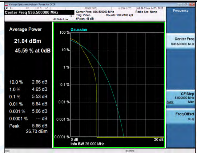
Band5-10MHz-16QAM-20525-1RB#0-PASS
