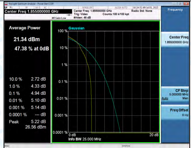
Band2-10MHz-16QAM-18650-1RB#0-PASS
