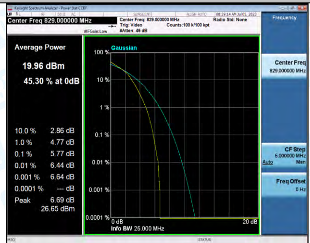
Band5-10MHz-16QAM-20450-50RB#0-PASS
