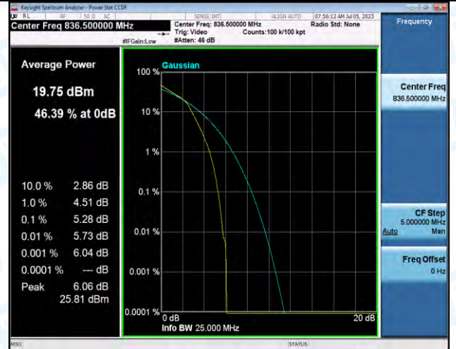
Band5-3MHz-16QAM-20525-15RB#0-PASS
