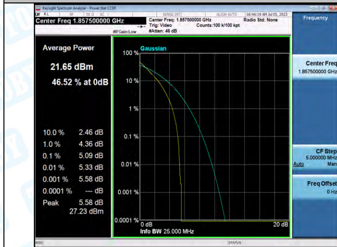
Band2-15MHz-QPSK-18675-75RB#0-PASS
