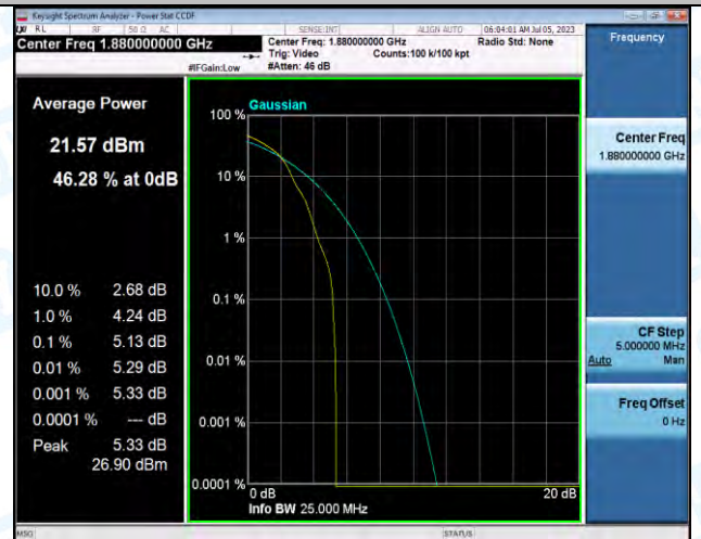
Band2-5MHz-16QAM-18900-1RB#0-PASS
