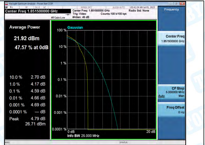
Band2-3MHz-16QAM-18615-1RB#0-PASS
