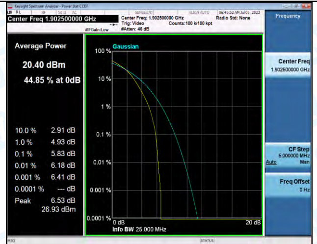
Band2-15MHz-16QAM-19125-75RB#0-PASS
