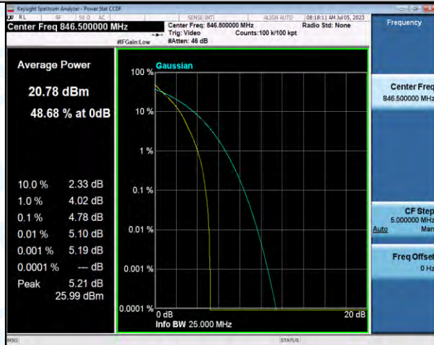
Band5-5MHz-QPSK-20625-25RB#0-PASS
