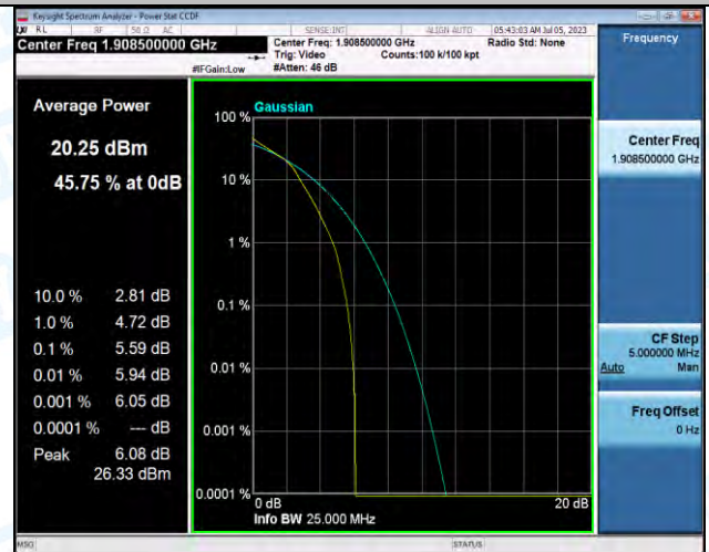
Band2-3MHz-16QAM-19185-15RB#0-PASS
