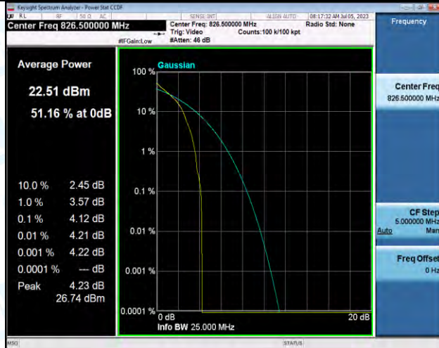
Band5-5MHz-QPSK-20425-1RB#0-PASS
