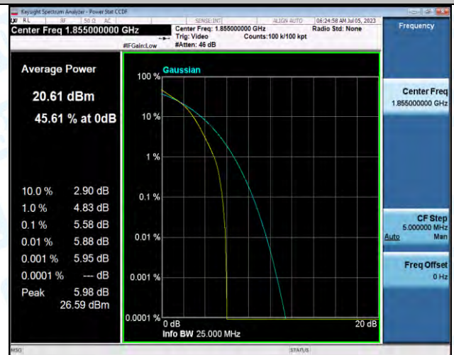
Band2-10MHz-16QAM-18650-50RB#0-PASS
