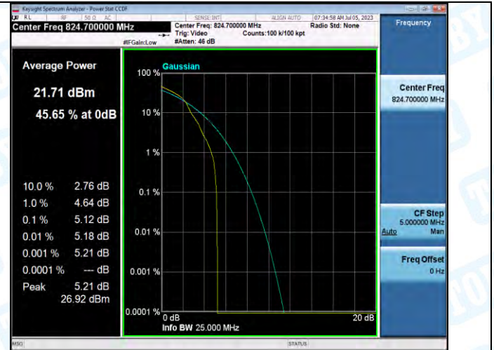
Band5-1.4MHz-16QAM-20407-1RB#0-PASS
