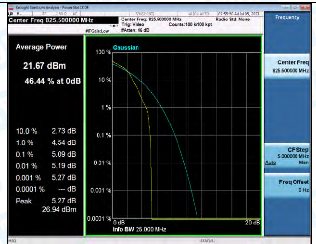
Band5-3MHz-16QAM-20415-1RB#0-PASS
