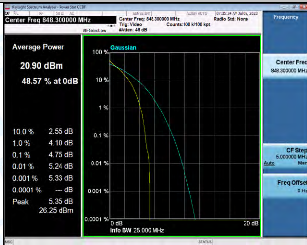
Band5-1.4MHz-QPSK-20643-6RB#0-PASS
