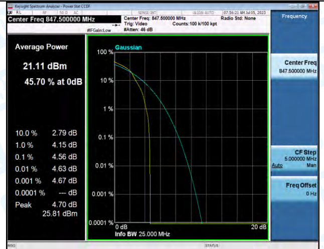
Band5-3MHz-16QAM-20635-1RB#0-PASS
