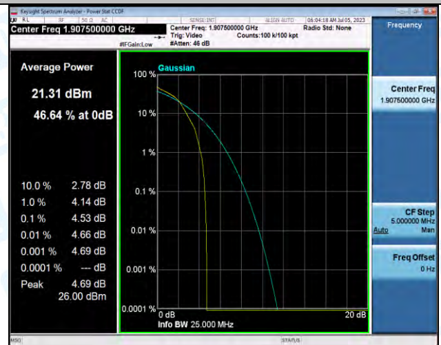
Band2-5MHz-16QAM-19175-1RB#0-PASS
