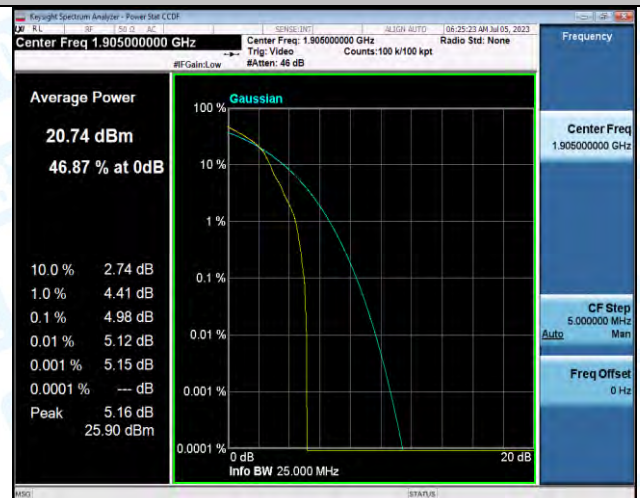
Band2-10MHz-16QAM-19150-1RB#0-PASS
