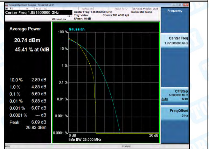
Band2-3MHz-16QAM-18615-15RB#0-PASS
