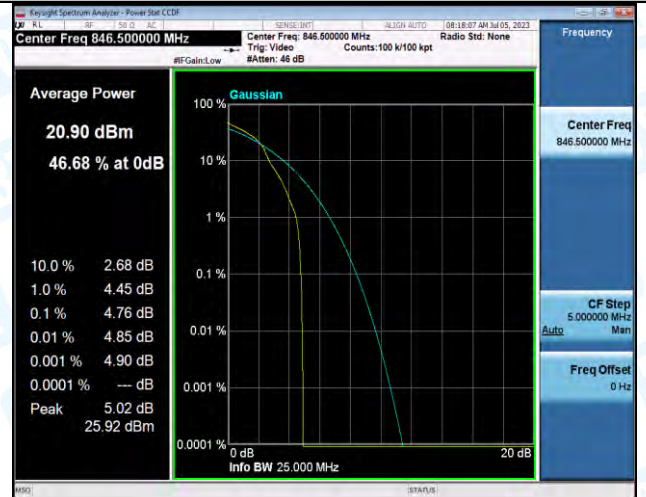
Band5-5MHz-16QAM-20625-1RB#0-PASS
