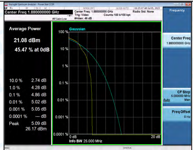
Band2-10MHz-16QAM-18900-1RB#0-PASS
