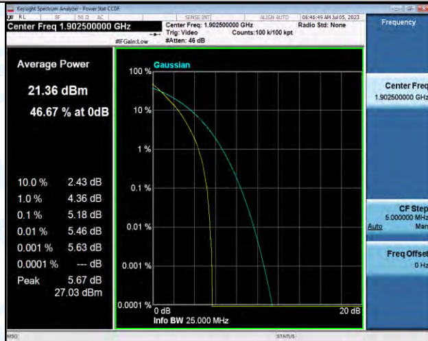
Band2-15MHz-QPSK-19125-75RB#0-PASS
