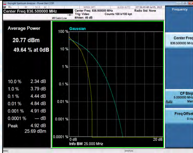
Band5-3MHz-QPSK-20525-15RB#0-PASS
