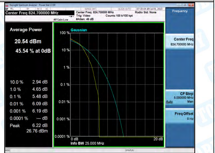
Band5-1.4MHz-16QAM-20407-6RB#0-PASS
