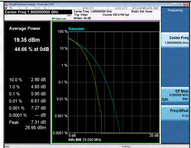
Band2-20MHz-16QAM-19100-100RB#0-PASS
