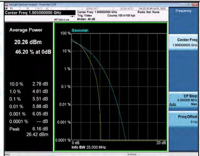
Band2-10MHz-16QAM-19150-50RB#0-PASS
