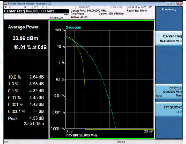
Band5-10MHz-16QAM-20600-1RB#0-PASS
