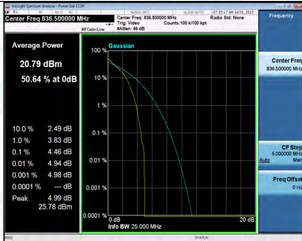
Band5-1.4MHz-QPSK-20525-6RB#0-PASS
