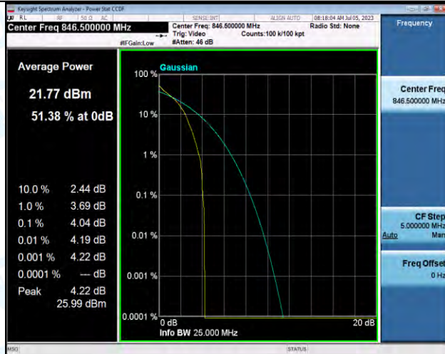
Band5-5MHz-QPSK-20625-1RB#0-PASS
