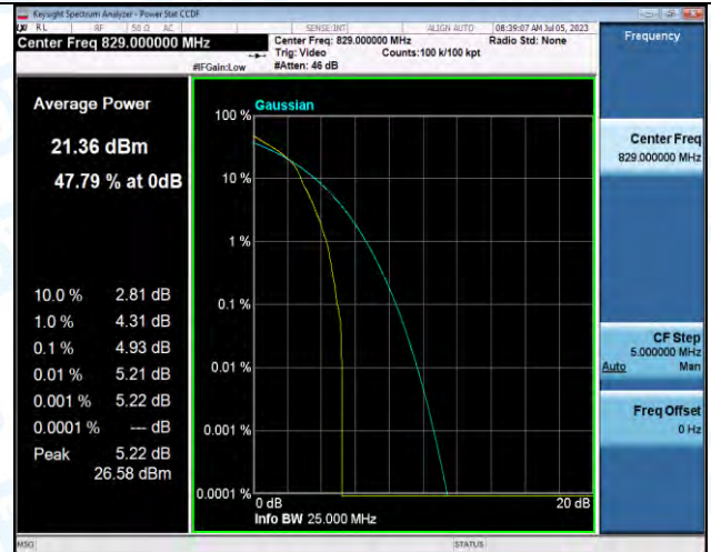
Band5-10MHz-16QAM-20450-1RB#0-PASS
