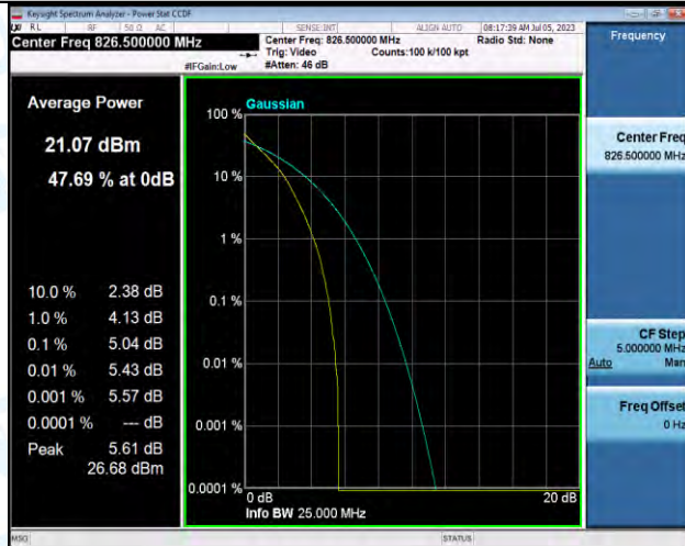
Band5-5MHz-QPSK-20425-25RB#0-PASS
