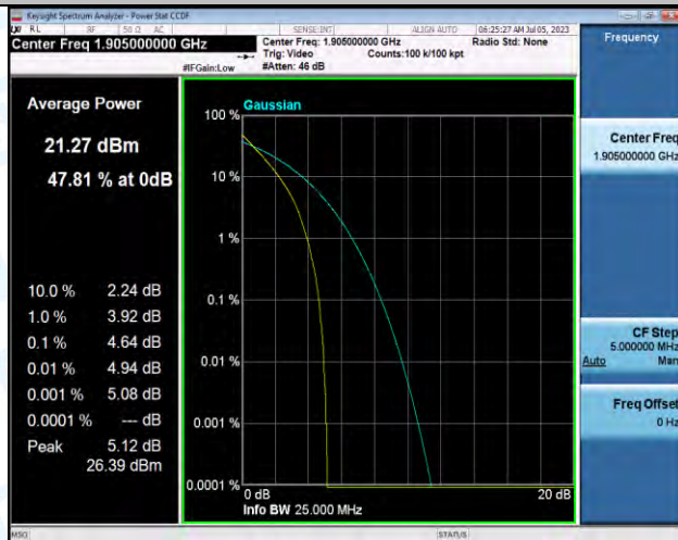
Band2-10MHz-QPSK-19150-50RB#0-PASS
