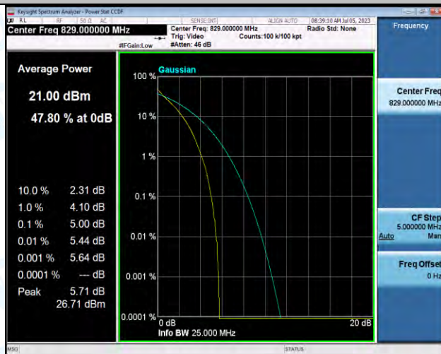
Band5-10MHz-QPSK-20450-50RB#0-PASS
