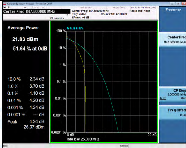
Band5-3MHz-QPSK-20635-1RB#0-PASS
