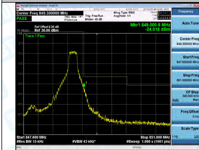
Band5_Band5_1.4MHz_QPSK_20643_1RB#5
