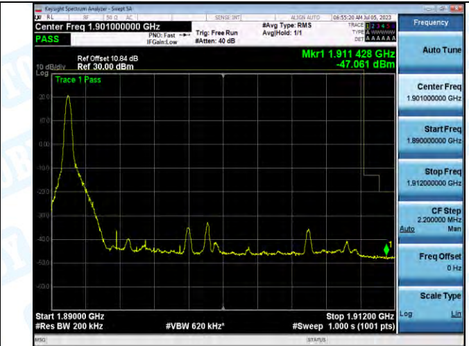
Band2_Band2_20MHz_16QAM_19100_1RB#0
