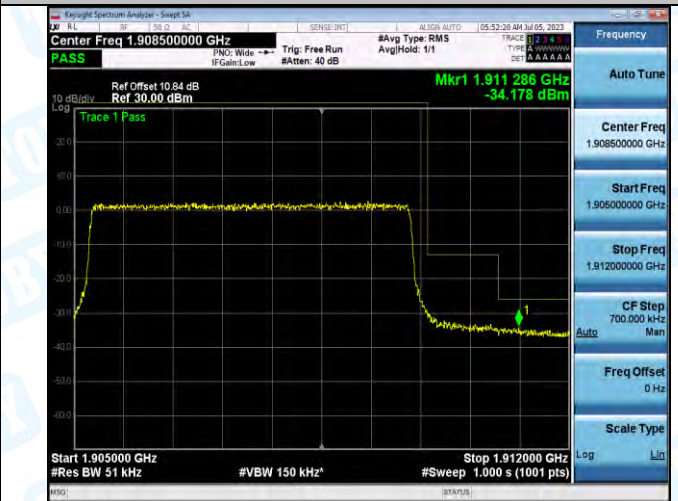
Band2_Band2_5MHz_16QAM_19175_25RB#0
