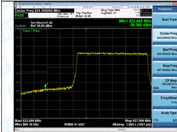
Band5_Band5_3MHz_QPSK_20415_15RB#0
