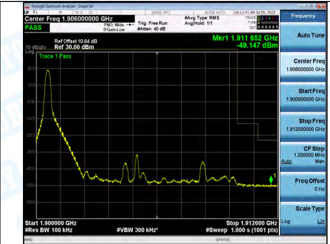
Band2_Band2_10MHz_16QAM_19150_1RB#0
