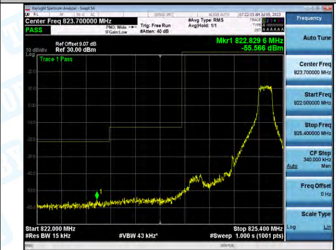
Band5_Band5_1.4MHz_16QAM_20407_1RB#5
