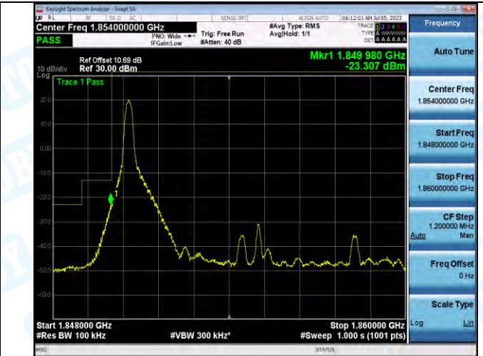
Band2_Band2_10MHz_16QAM_18650_1RB#0
