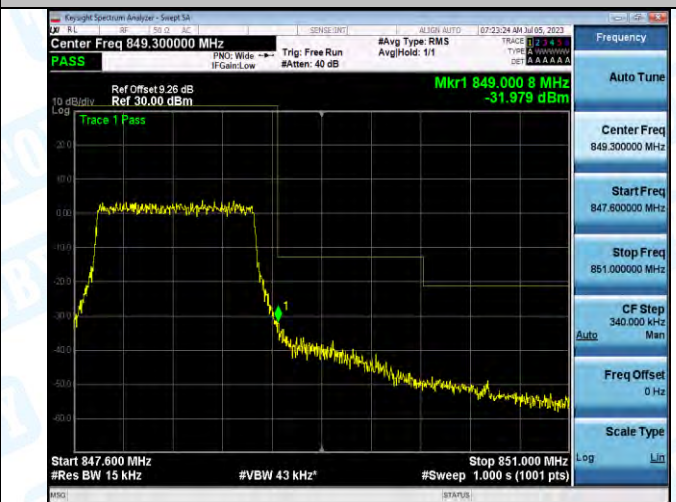
Band5_Band5_1.4MHz_16QAM_20643_6RB#0
