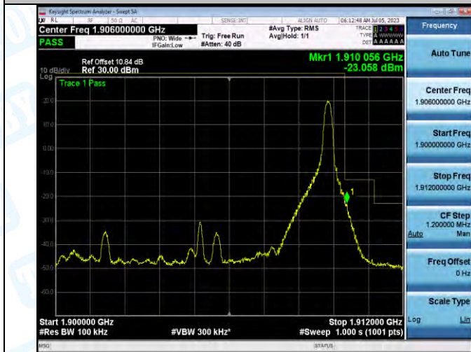
Band2_Band2_10MHz_QPSK_19150_1RB#49
