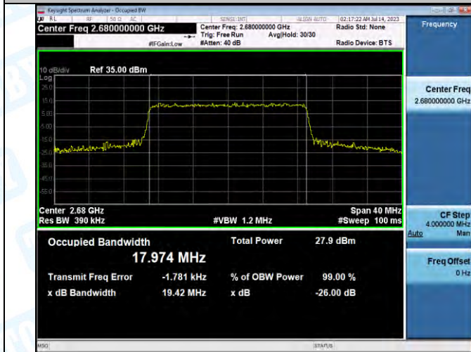
Band41-20MHz-QPSK-41490-100RB#0-PASS
