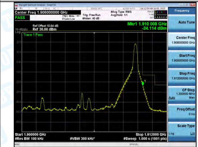
Band2_Band2_10MHz_16QAM_19150_1RB#49
