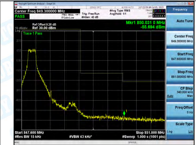
Band5_Band5_1.4MHz_16QAM_20643_1RB#0
