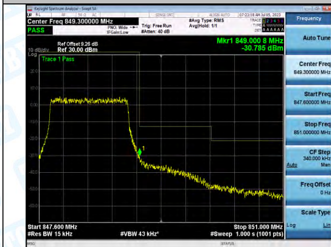
Band5_Band5_1.4MHz_QPSK_20643_6RB#0
