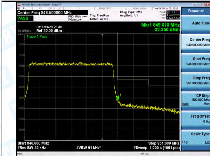
Band5_Band5_3MHz_QPSK_20635_15RB#0
