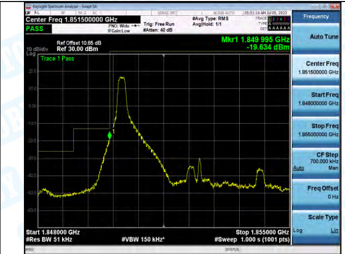
Band2_Band2_5MHz_16QAM_18625_1RB#0
