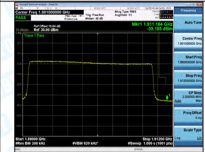
Band2_Band2_20MHz_16QAM_19100_100RB#0
