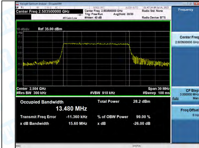
Band41-15MHz-QPSK-39725-75RB#0-PASS
