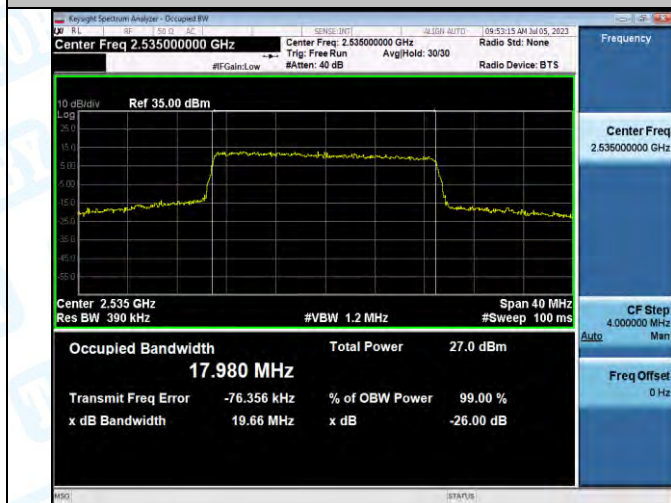
Band7-20MHz-QPSK-21100-100RB#0-PASS
