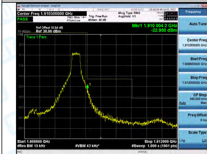
Band2_Band2_1.4MHz_QPSK_19193_1RB#5
