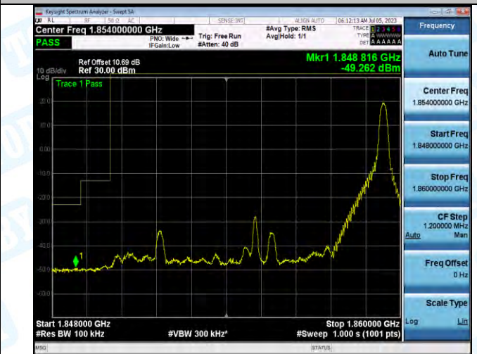
Band2_Band2_10MHz_16QAM_18650_1RB#49
