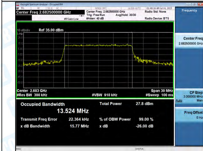
Band41-15MHz-QPSK-41515-75RB#0-PASS
