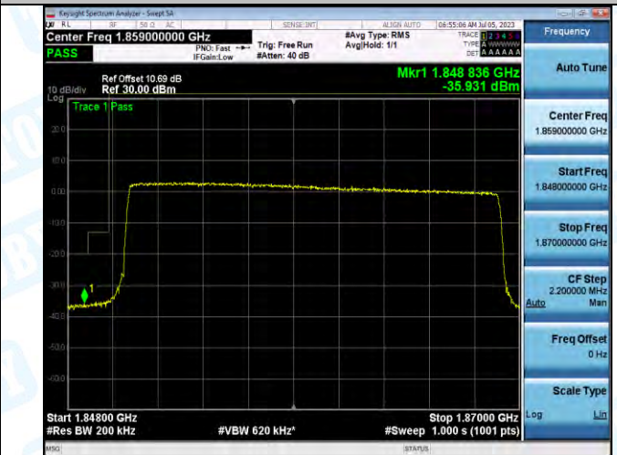
Band2_Band2_20MHz_16QAM_18700_100RB#0
