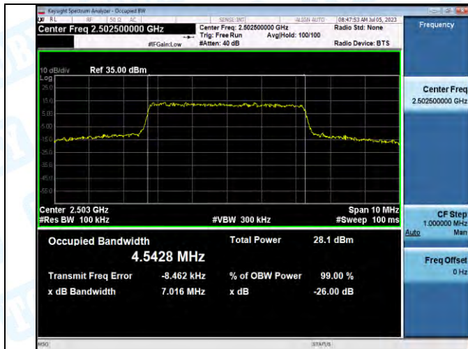
Band7-5MHz-QPSK-20775-25RB#0-PASS
