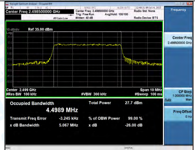
Band41-5MHz-16QAM-39675-25RB#0-PASS
