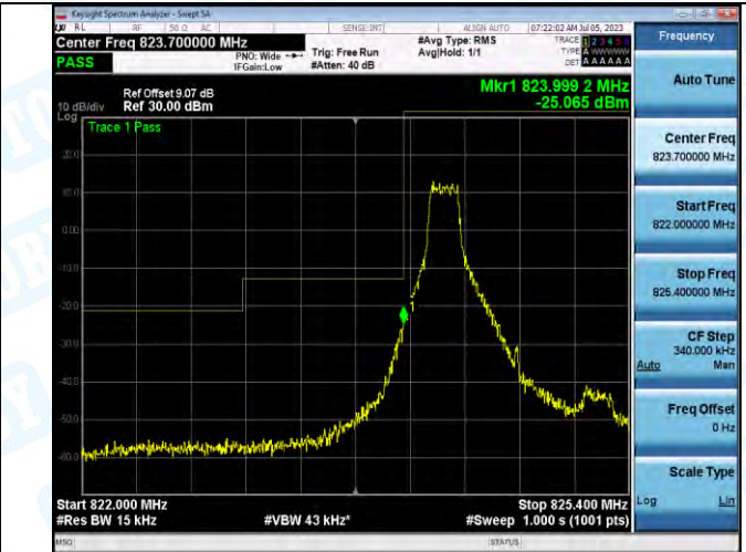
Band5_Band5_1.4MHz_16QAM_20407_1RB#0
