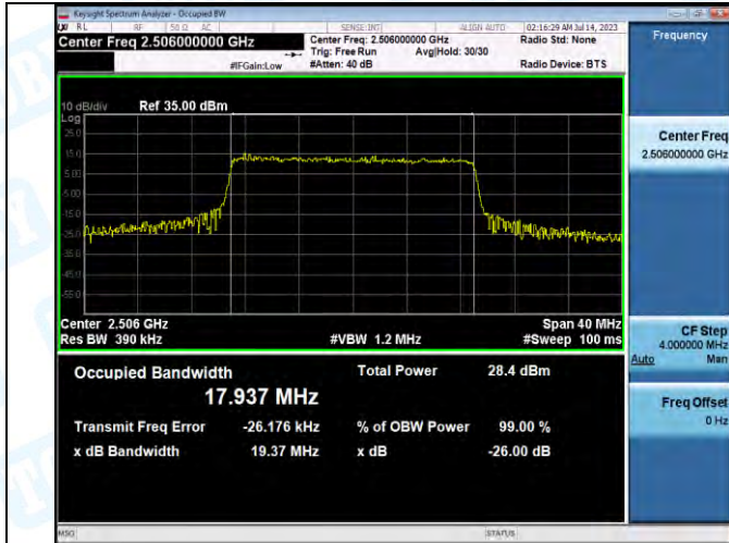
Band41-20MHz-QPSK-39750-100RB#0-PASS
