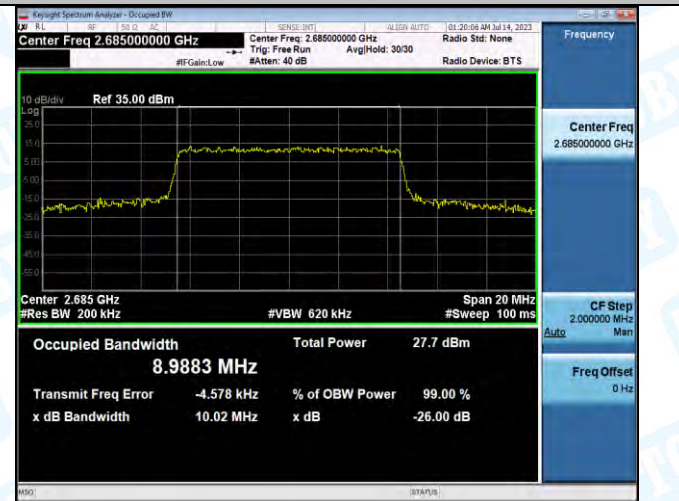
Band41-10MHz-16QAM-41540-50RB#0-PASS
