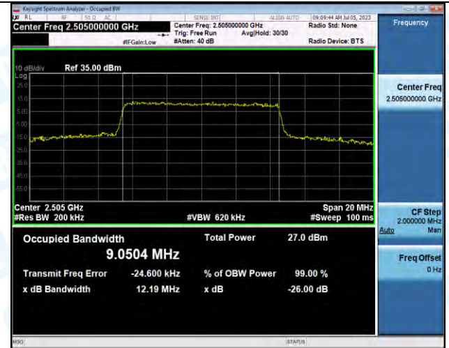
Band7-10MHz-16QAM-20800-50RB#0-PASS
