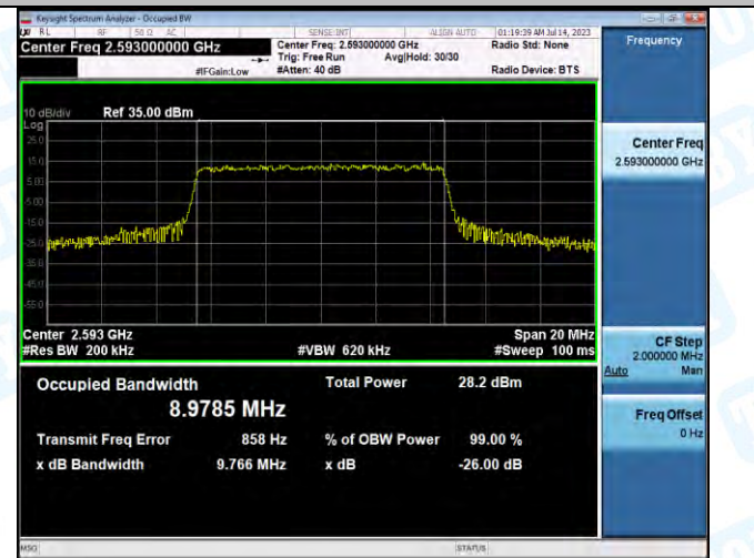
Band41-10MHz-16QAM-40620-50RB#0-PASS
