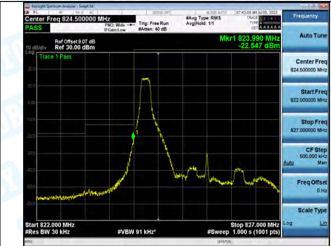
Band5_Band5_3MHz_16QAM_20415_1RB#0
