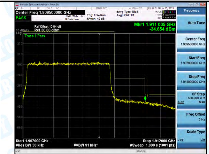
Band2_Band2_3MHz_16QAM_19185_15RB#0
