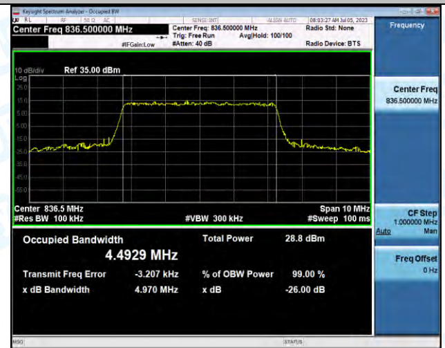
Band5-5MHz-16QAM-20525-25RB#0-PASS
