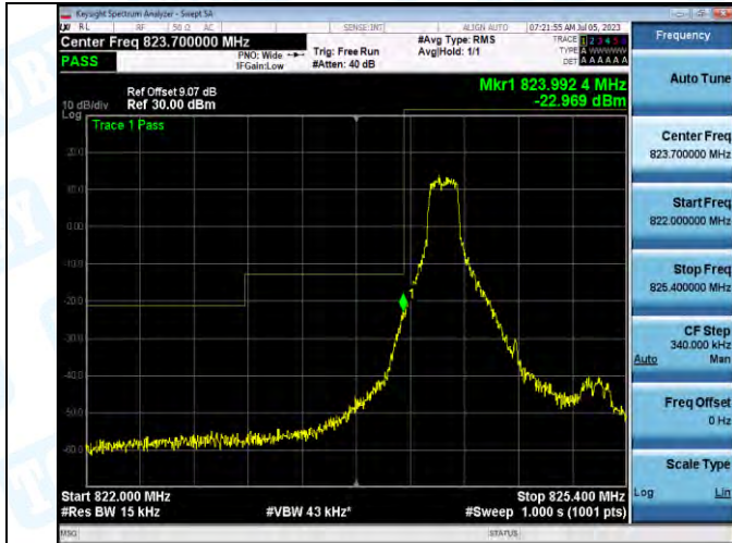
Band5_Band5_1.4MHz_QPSK_20407_1RB#0
