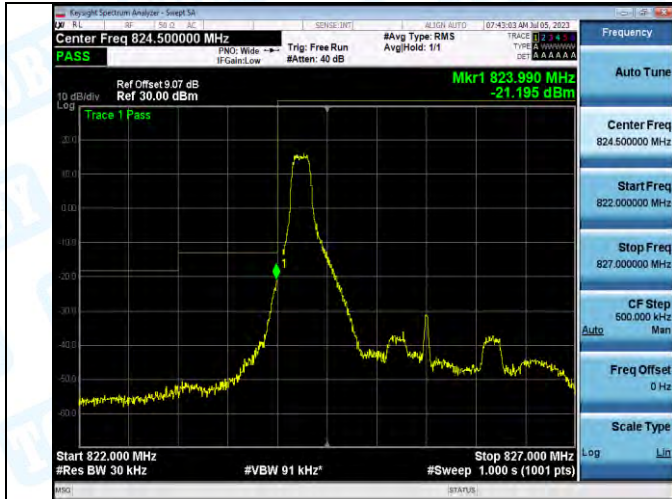
Band5_Band5_3MHz_QPSK_20415_1RB#0
