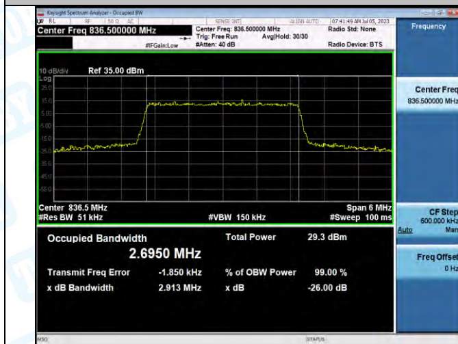
Band5-3MHz-QPSK-20525-15RB#0-PASS
