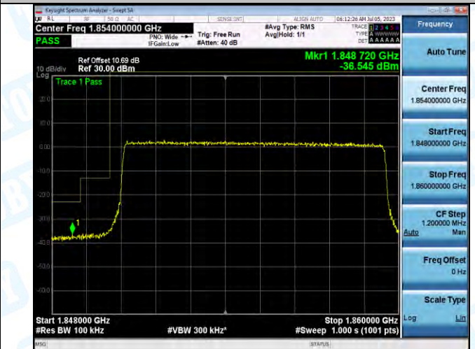
Band2_Band2_10MHz_16QAM_18650_50RB#0
