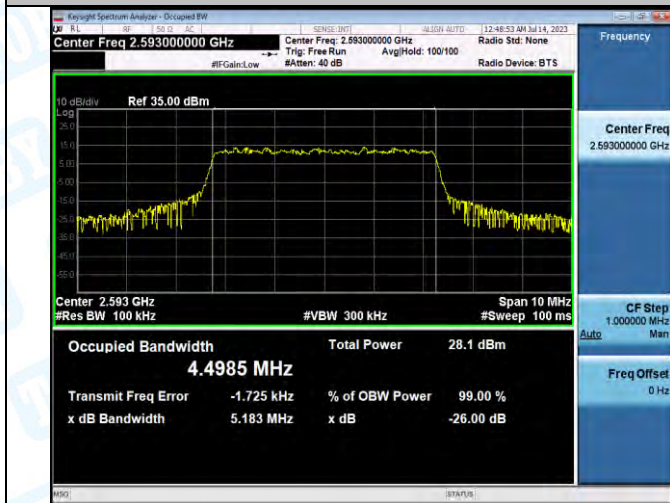
Band41-5MHz-QPSK-40620-25RB#0-PASS
