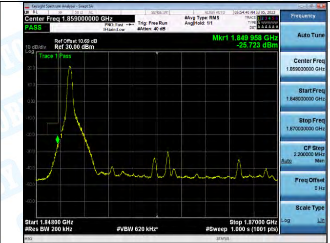
Band2_Band2_20MHz_16QAM_18700_1RB#0
