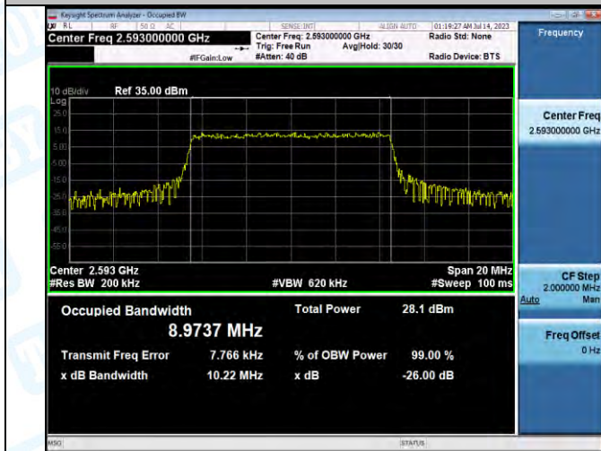
Band41-10MHz-QPSK-40620-50RB#0-PASS
