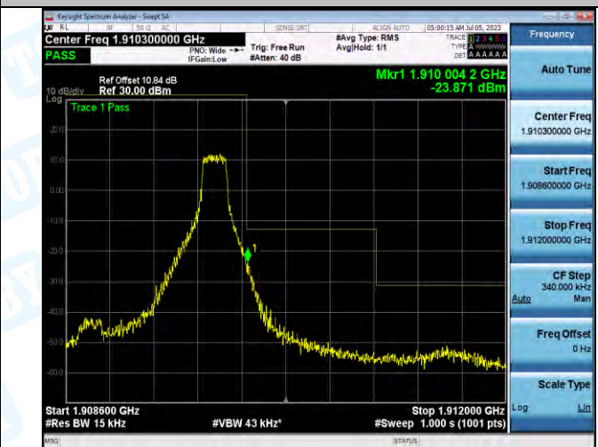
Band2_Band2_1.4MHz_16QAM_19193_1RB#5
