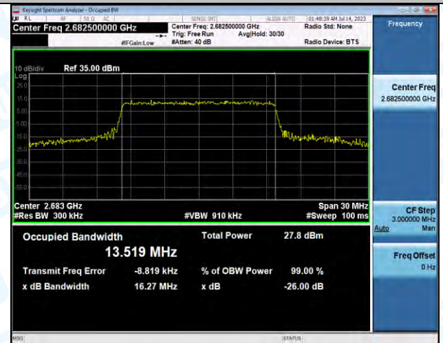
Band41-15MHz-16QAM-41515-75RB#0-PASS
