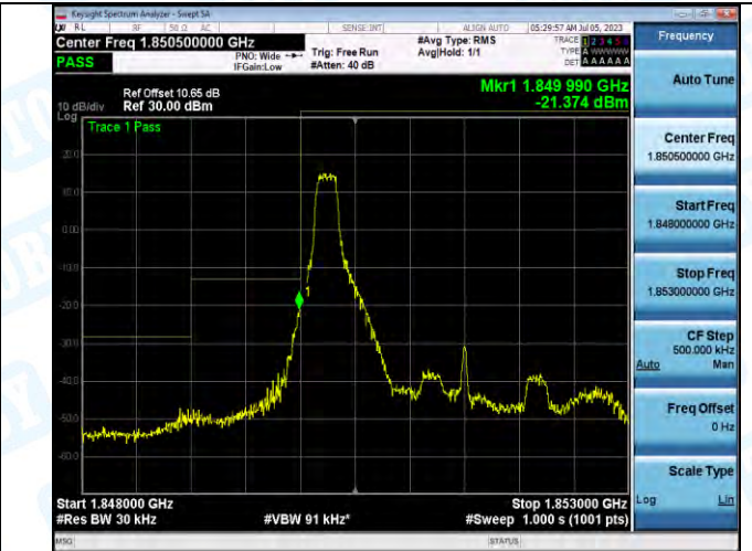
Band2_Band2_3MHz_16QAM_18615_1RB#0
