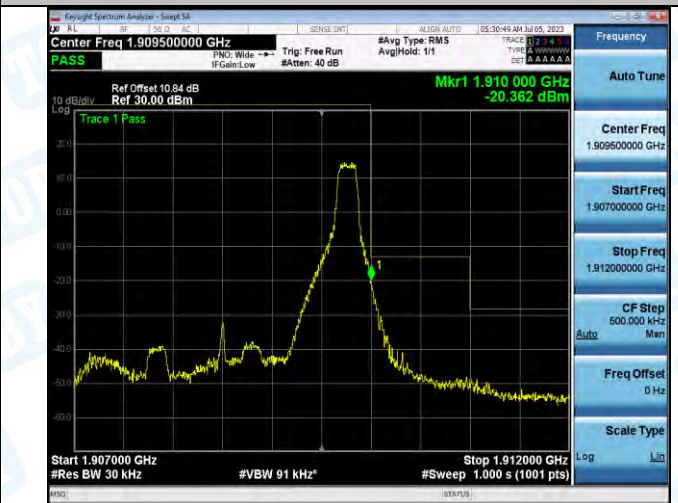
Band2_Band2_3MHz_16QAM_19185_1RB#14
