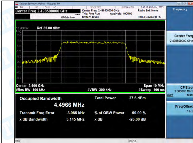
Band41-5MHz-QPSK-39675-25RB#0-PASS
