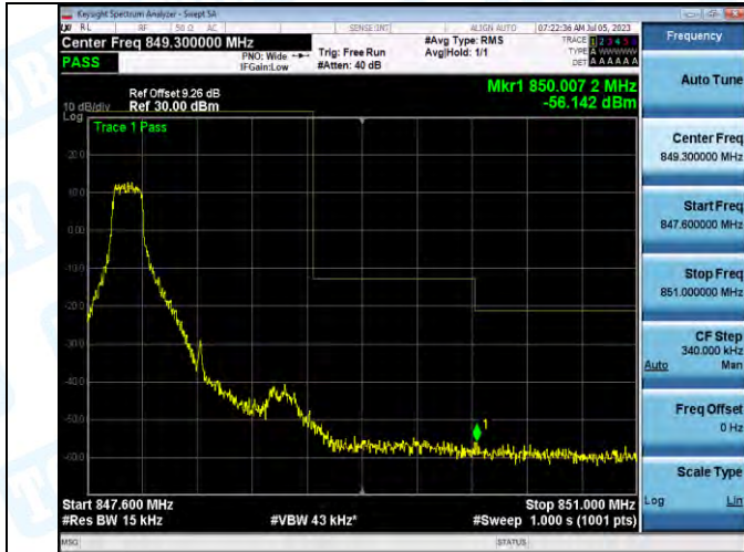
Band5_Band5_1.4MHz_QPSK_20643_1RB#0
