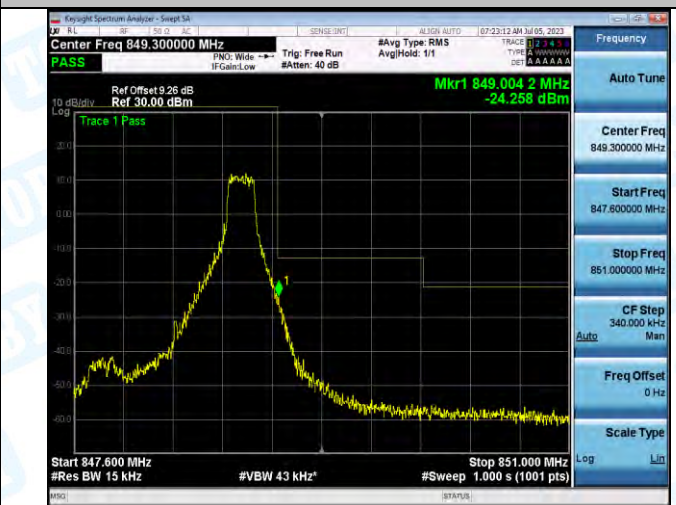
Band5_Band5_1.4MHz_16QAM_20643_1RB#5
