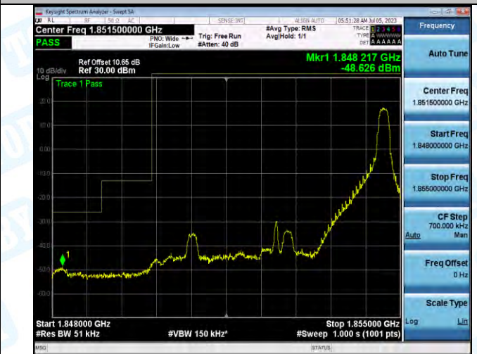
Band2_Band2_5MHz_16QAM_18625_1RB#24
