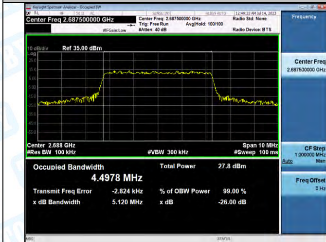
Band41-5MHz-QPSK-41565-25RB#0-PASS
