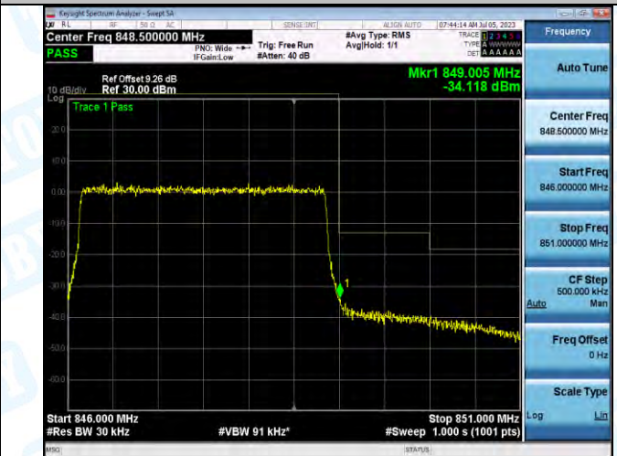
Band5_Band5_3MHz_16QAM_20635_15RB#0
