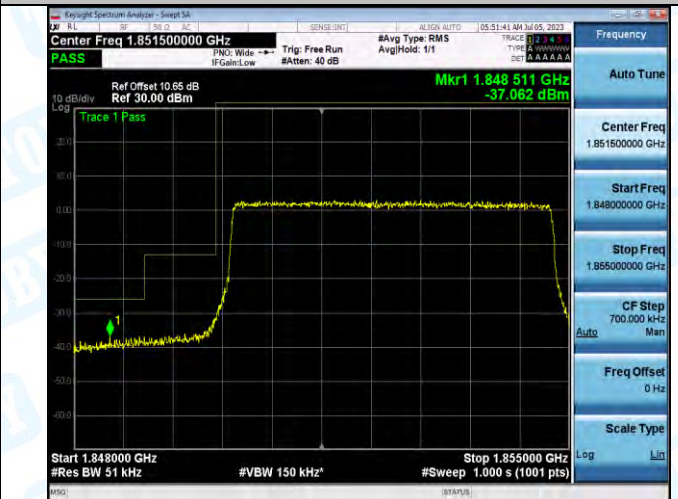
Band2_Band2_5MHz_16QAM_18625_25RB#0
