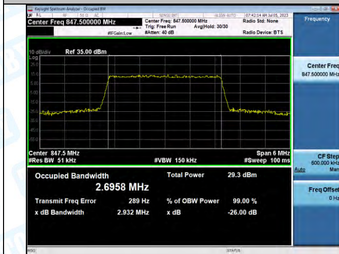
Band5-3MHz-QPSK-20635-15RB#0-PASS
