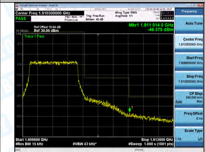
Band2_Band2_1.4MHz_16QAM_19193_6RB#0
