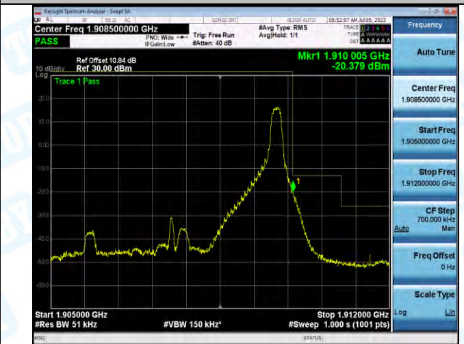
Band2_Band2_5MHz_16QAM_19175_1RB#24
