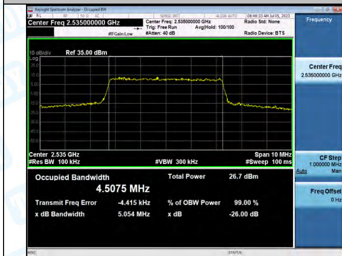
Band7-5MHz-QPSK-21100-25RB#0-PASS
