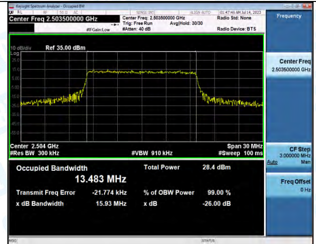
Band41-15MHz-16QAM-39725-75RB#0-PASS
