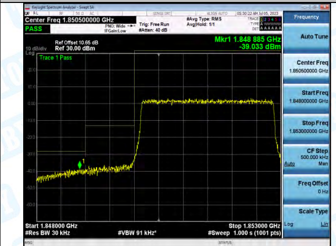
Band2_Band2_3MHz_16QAM_18615_15RB#0
