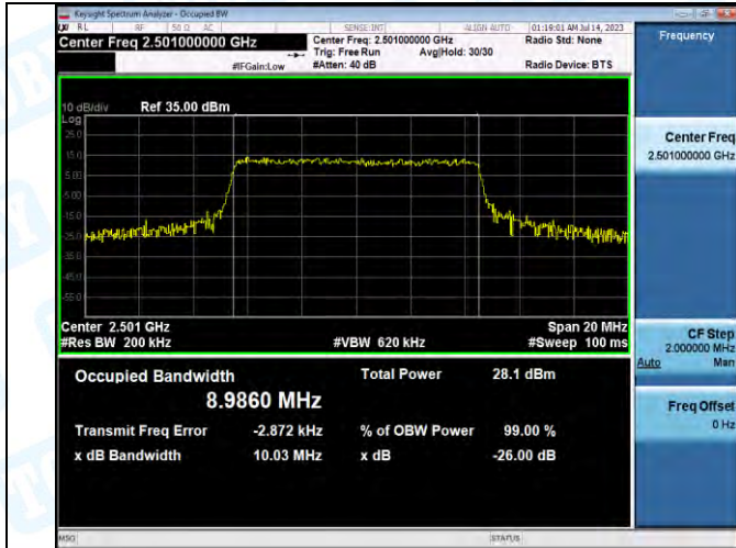
Band41-10MHz-QPSK-39700-50RB#0-PASS
