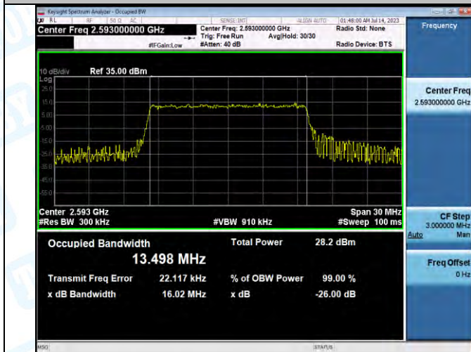
Band41-15MHz-QPSK-40620-75RB#0-PASS
