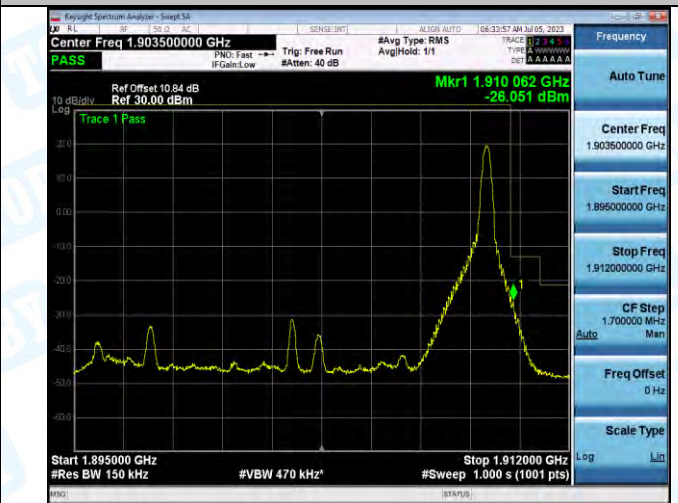
Band2_Band2_15MHz_16QAM_19125_1RB#74
