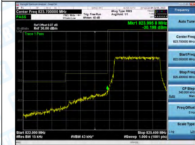
Band5_Band5_1.4MHz_QPSK_20407_6RB#0
