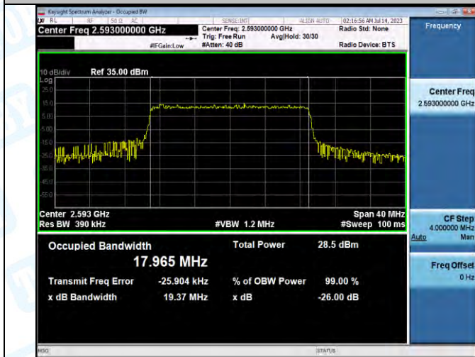
Band41-20MHz-QPSK-40620-100RB#0-PASS
