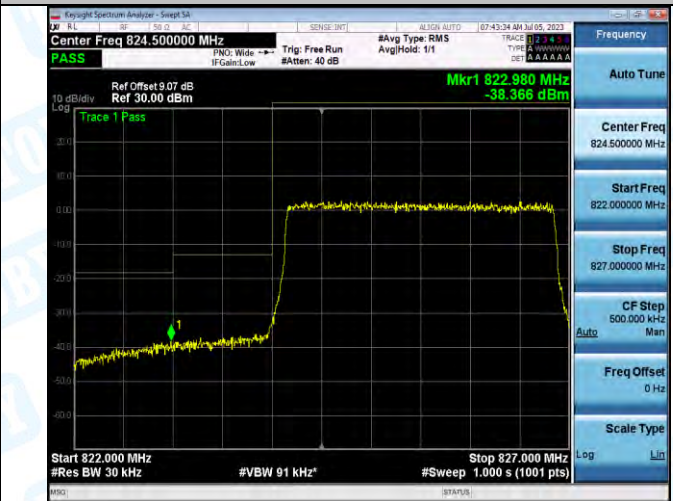
Band5_Band5_3MHz_16QAM_20415_15RB#0
