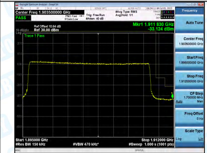
Band2_Band2_15MHz_16QAM_19125_75RB#0
