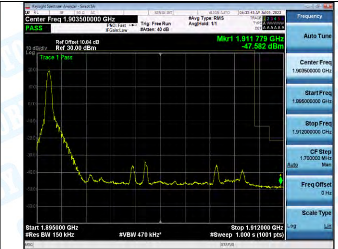
Band2_Band2_15MHz_16QAM_19125_1RB#0
