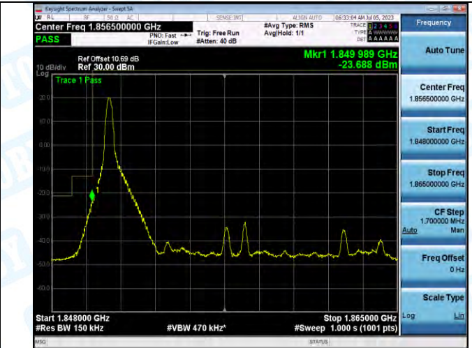
Band2_Band2_15MHz_16QAM_18675_1RB#0
