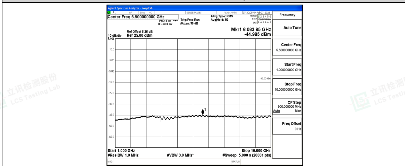
Band5-10MHz-16QAM-20600-1RB#0-Range4:1000~10000MHz
