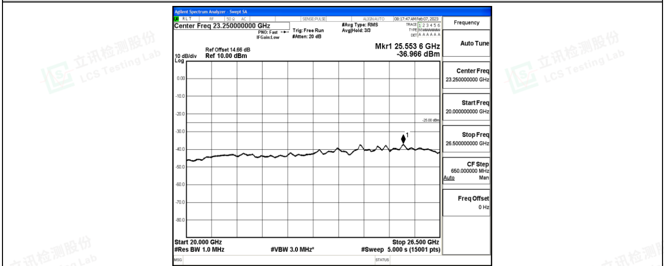
Band7-20MHz-16QAM-21350-1RB#0-Range6:20000~26500MHz
