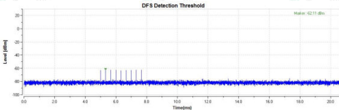
Radar Singal 5
