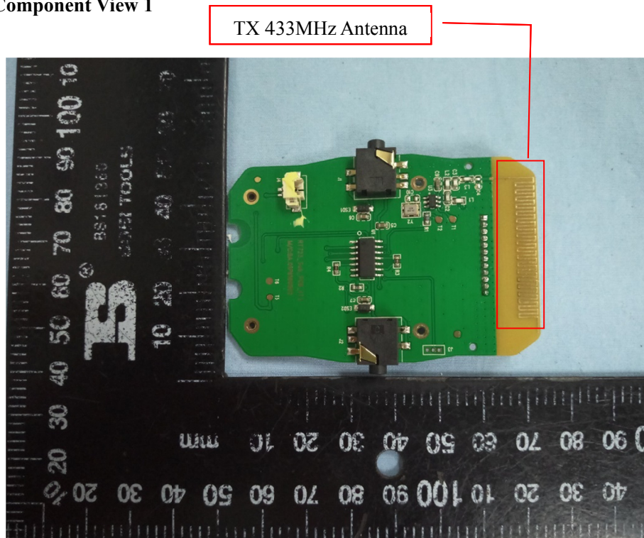
Solder Board-Component View 1
