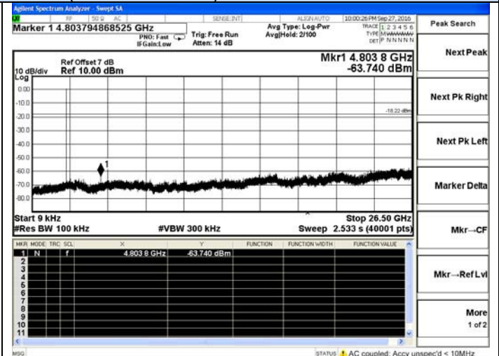
3DH1-Low channel
