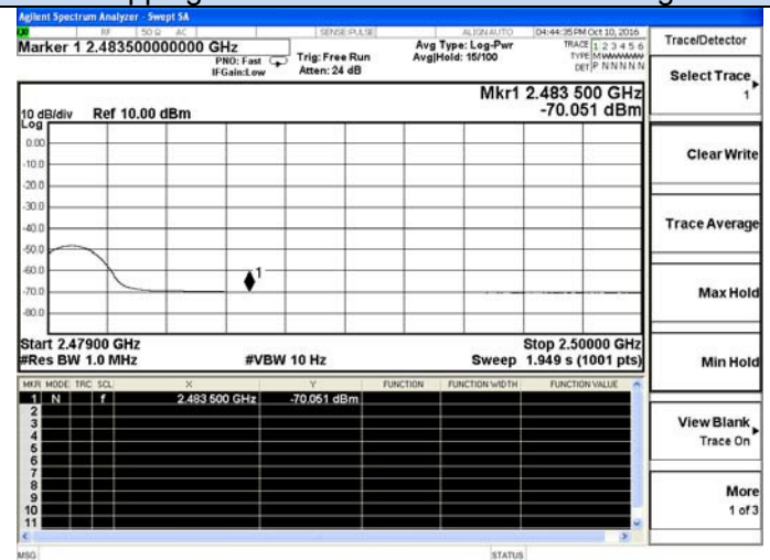
Hopping Off-8-DPSK- High channel-Average
