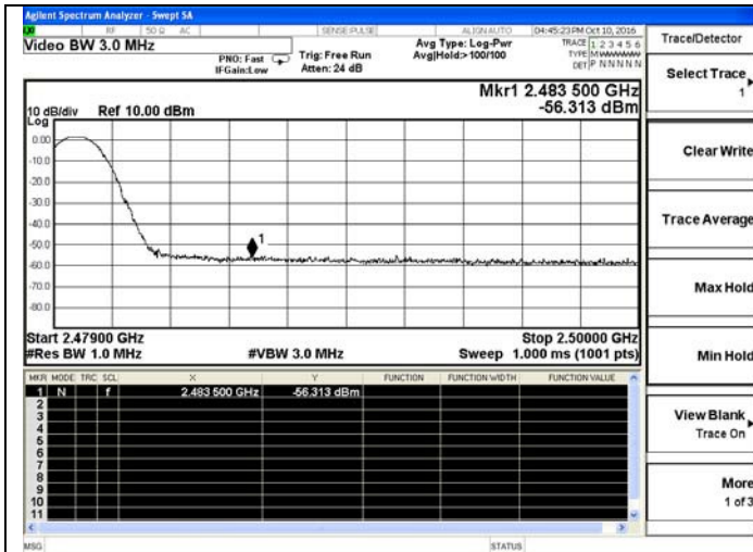
Hopping Off- \pi/4 -DQPSK- High channel-Peak
