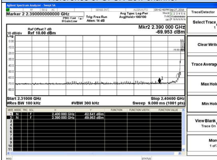
Hopping On-GFSK-Low channel
