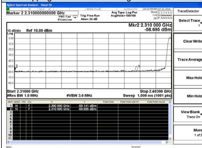
Hopping Off-8-DPSK- Low channel-Peak
