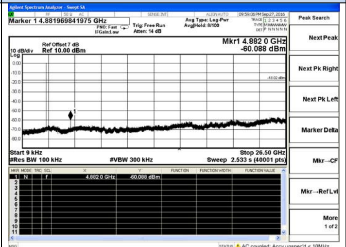
3DH1-Middle channel
