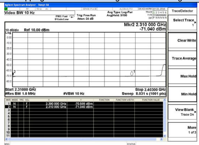
Hopping Off-8-DPSK- Low channel-Average
