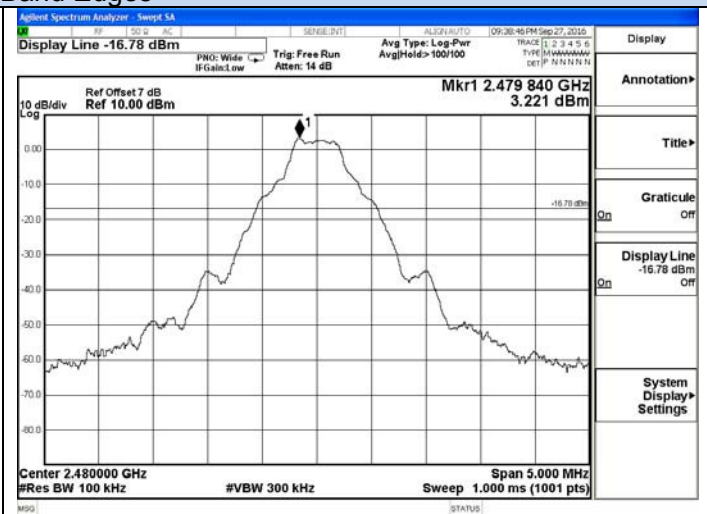
Test plot of Band Edges
