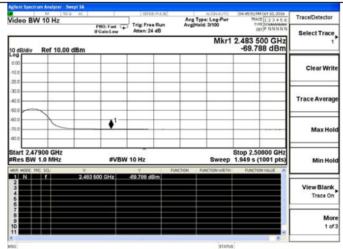
Hopping Off- \pi/4 -DQPSK- High channel-Average
