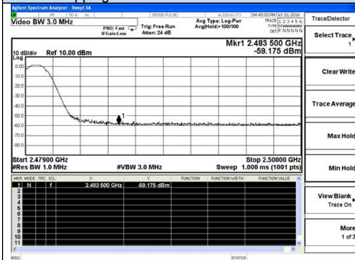
Hopping Off-8-DPSK- High channel-Peak
