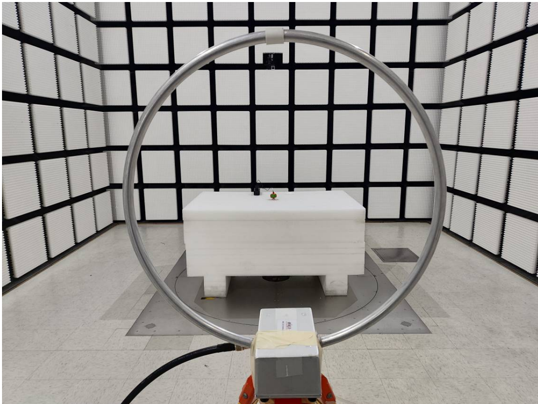
Radiated Emission 9k-30MHz Parallel View
