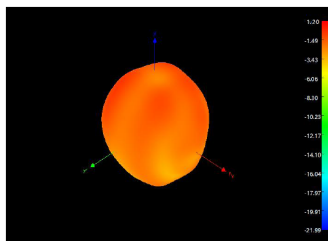
3D Radiation Pattern 2440MHz
