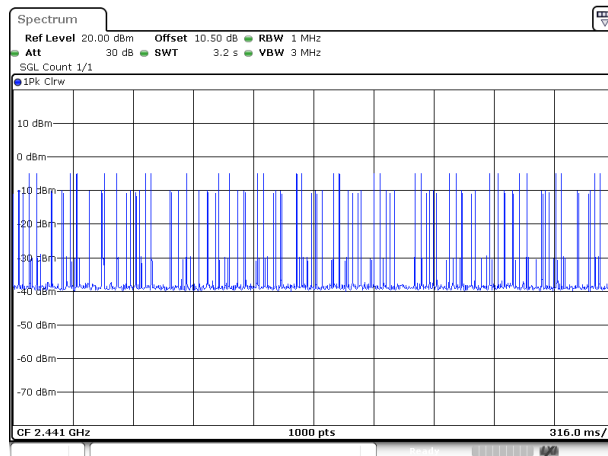
2DH1_Hopping
