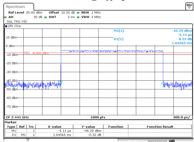
2DH3_Hopping
