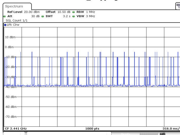
2DH3_Hopping
