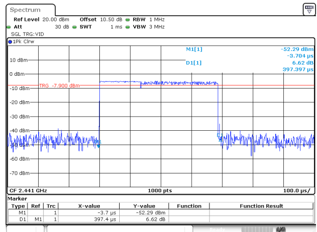
2DH1_Hopping
