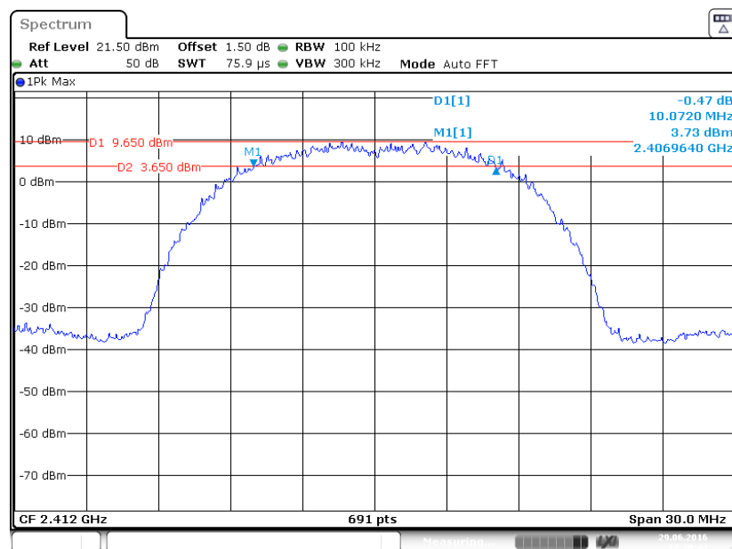
Chain 0 802.11b Low Channel
