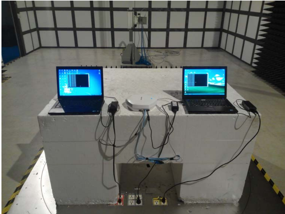
Radiated Emissions- Front View (Above 1G)
