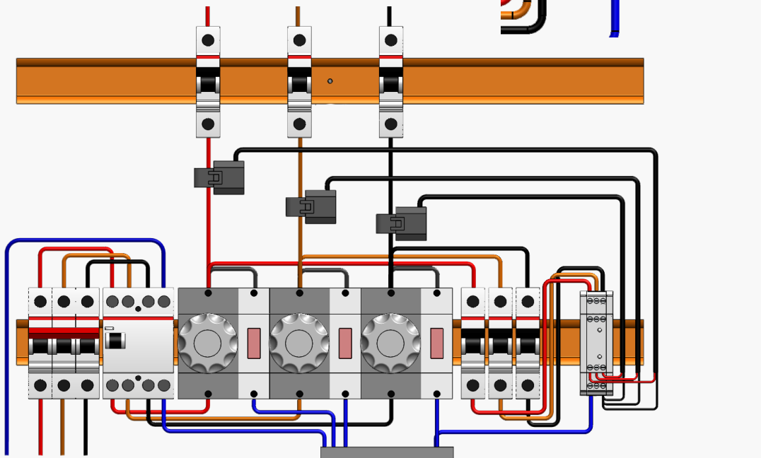
Electrical Panel with DinRail 3-Phase Advanced NB in a 3-Phase Panel
