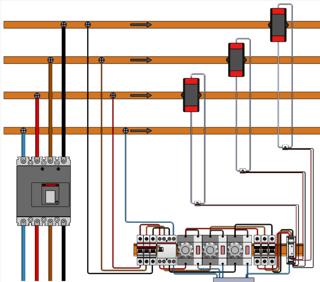
Electrical Panel with DinRail 3-Phase Advanced version 5A in a 3-Phase Panel
