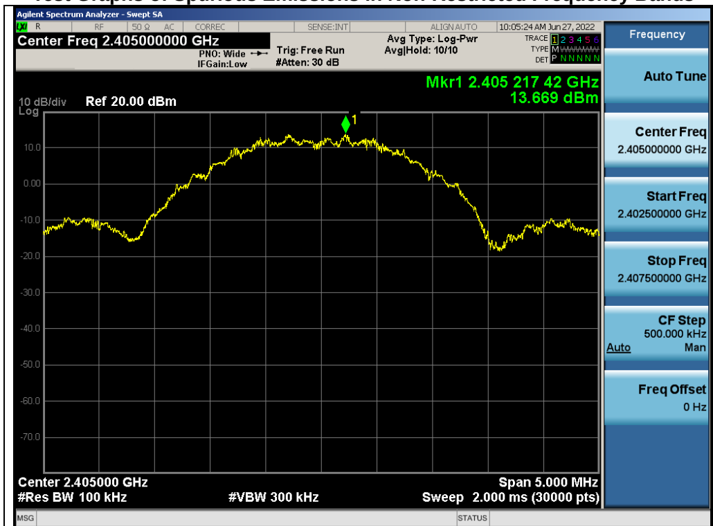
Test_Graph_2.4G_ANT1_2405_Reference Level
