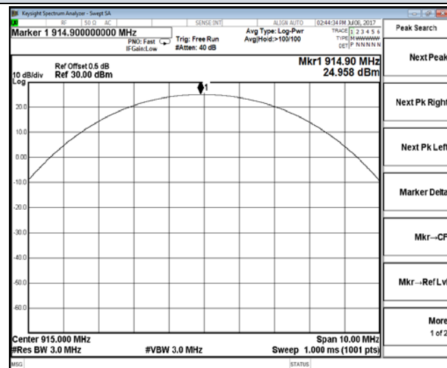
Channel 05 / 915 MHz
