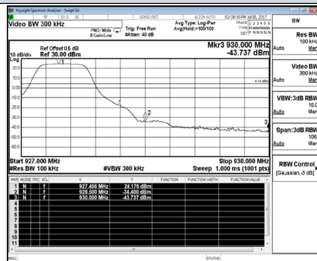
Channel 10 / 927.5 MHz
